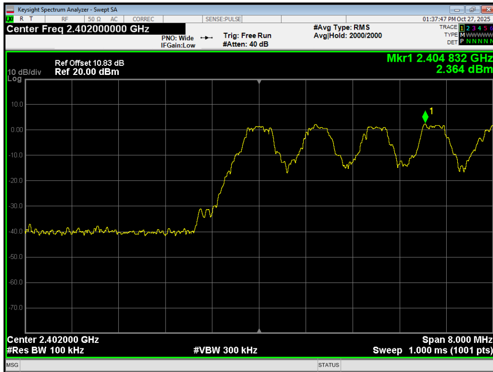
Band Edge(Hopping) 1-DH5 2402MHz Hopping Emission
