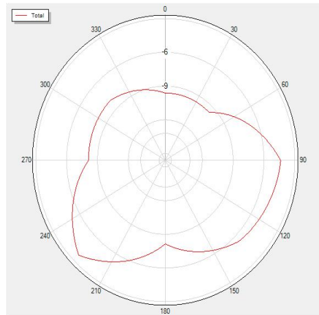
2450 Total
