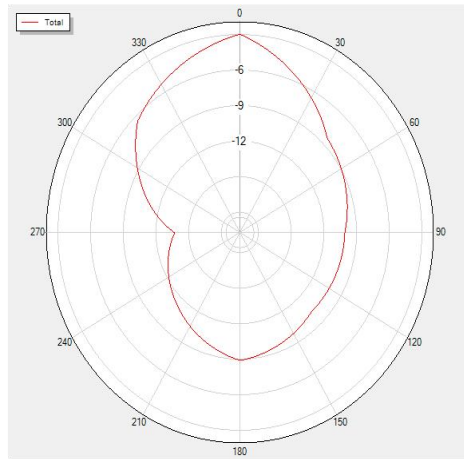
2400 Total
