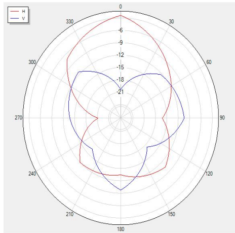
2400 Polar
