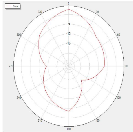
2450 Total
