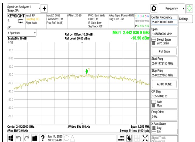
PSD_BLE 1M_MidCH20-2442MHz
