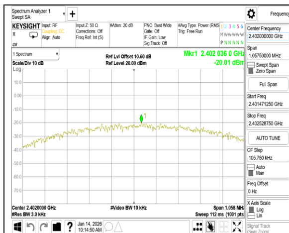
PSD_BLE 1M_LowCH00-2402MHz
