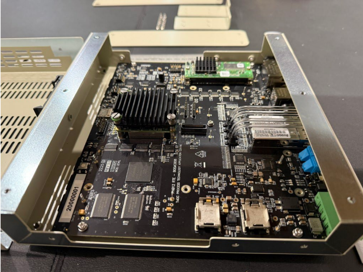
Figure 5 – PN912 Internal Left View
