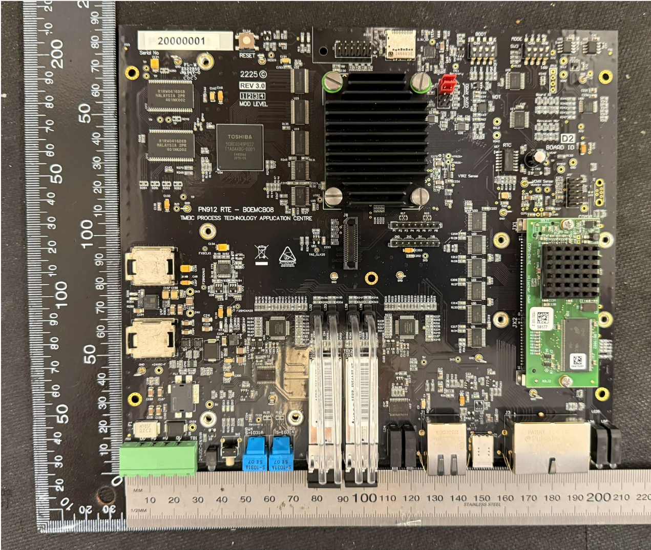
Figure 2 – PN912 Internal Main Board
