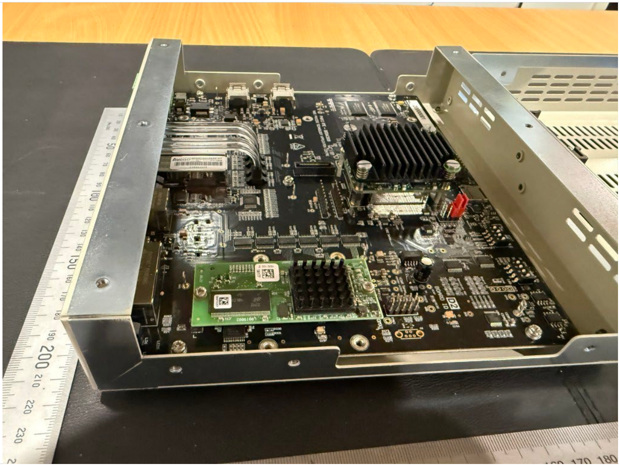
Figure 6 – PN912 Internal Right View
