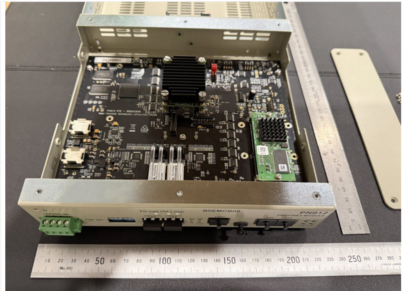
Figure 3 – PN912 Internal Front View
