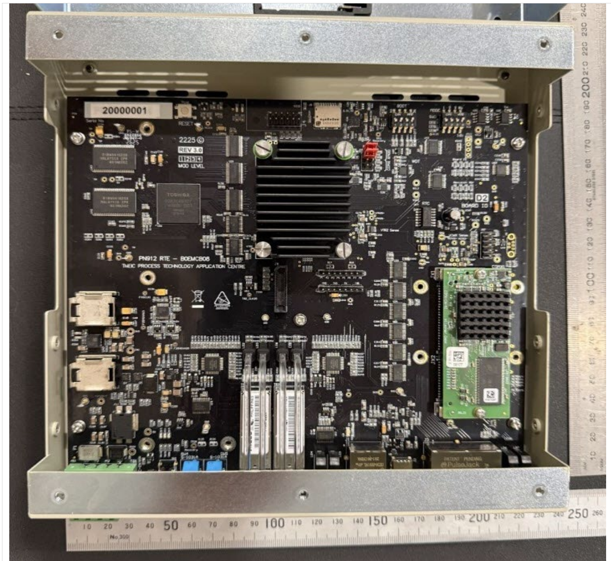
Figure 4 – PN912 Internal Top View
