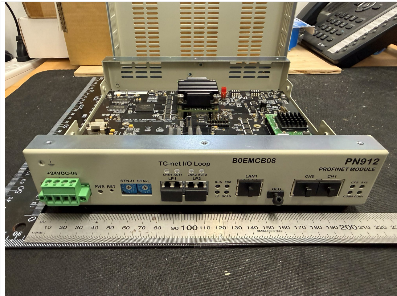
Figure 1 – PN912 Internal Front View
