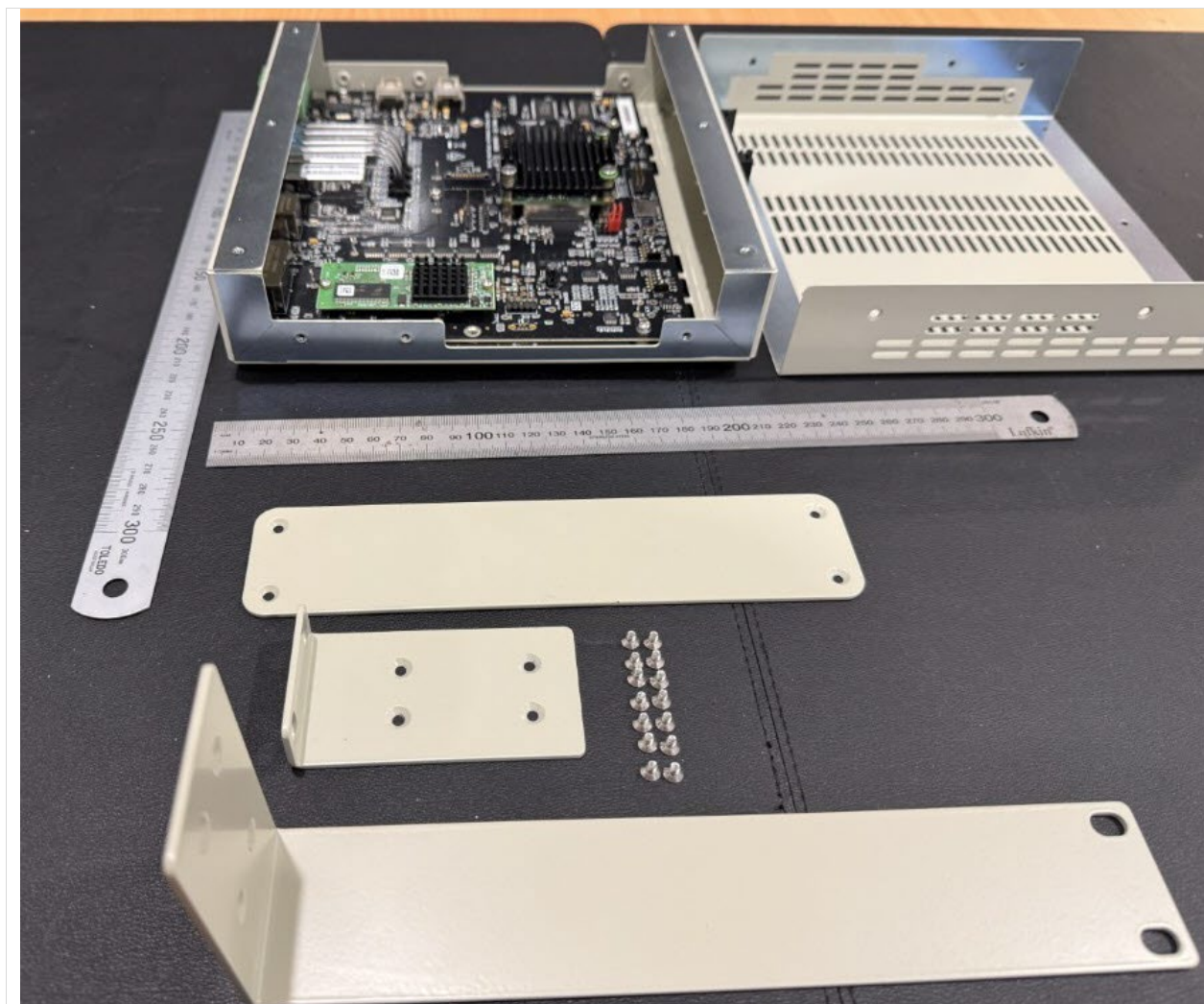
Figure 7 – PN912 Internal View & Accessories
