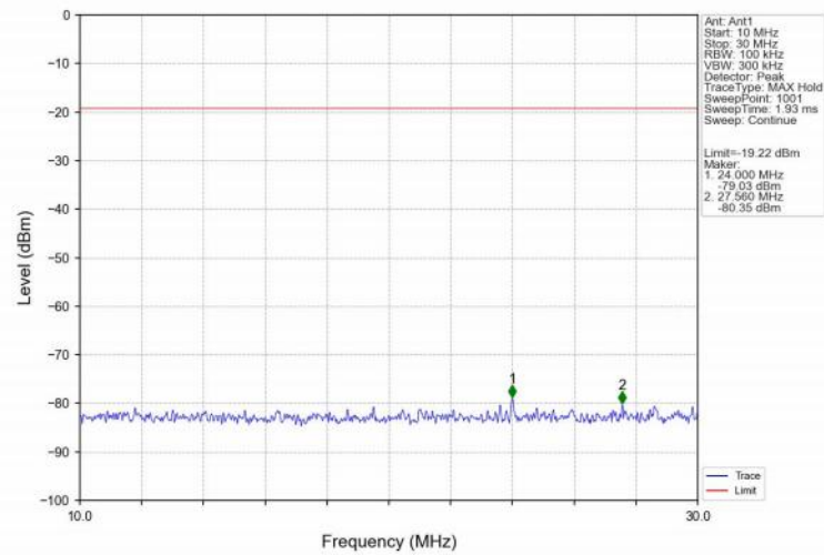
Pi/4DQPSK_2DH5_HCH_2480MHz_Ant1_NTNV
