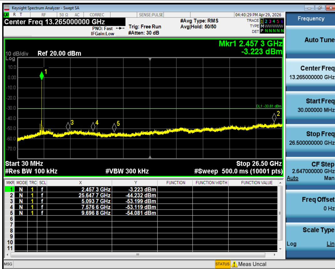
Tx. Spurious NVNT ax20 2462MHz Ant1 Emission
