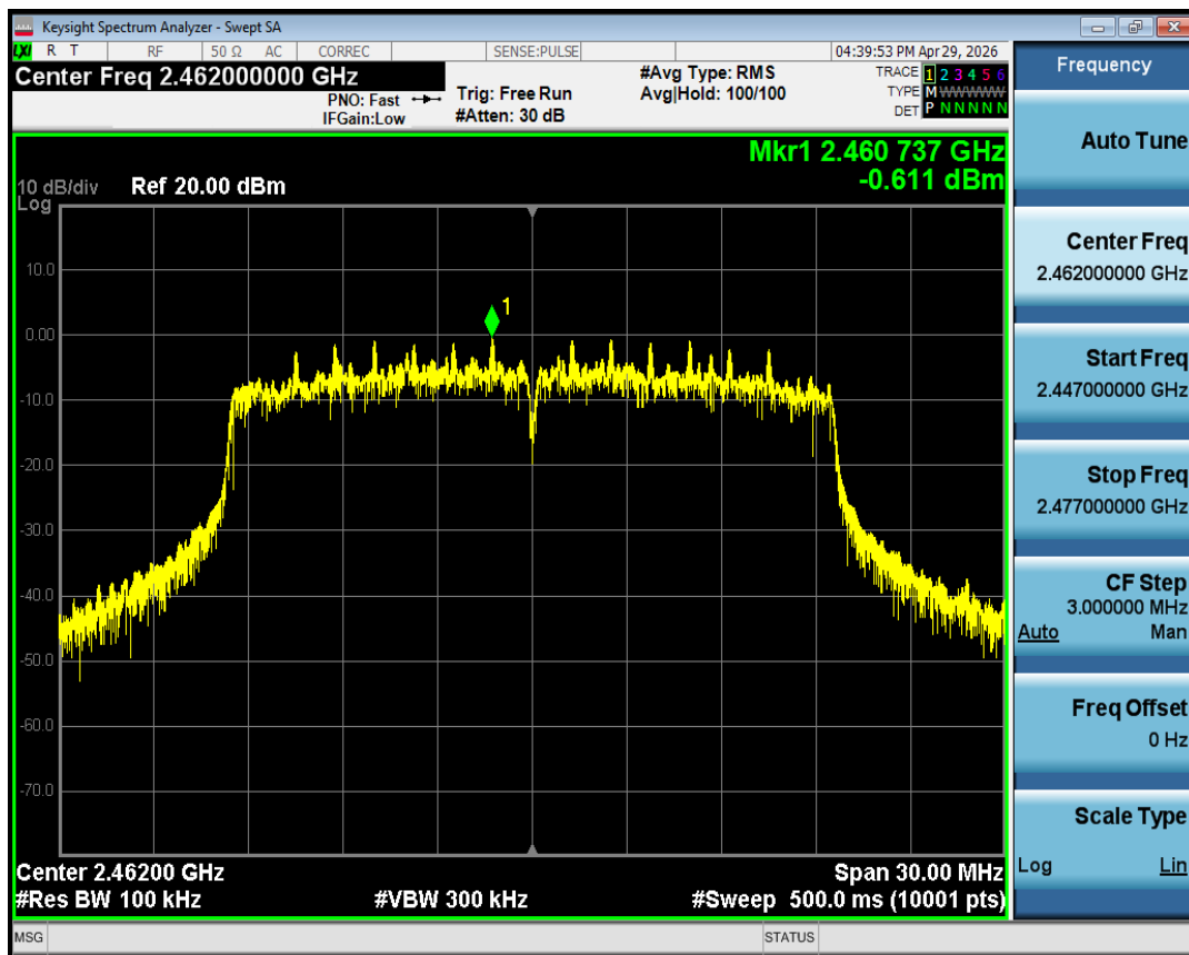
Tx. Spurious NVNT ax20 2462MHz Ant1 Ref
