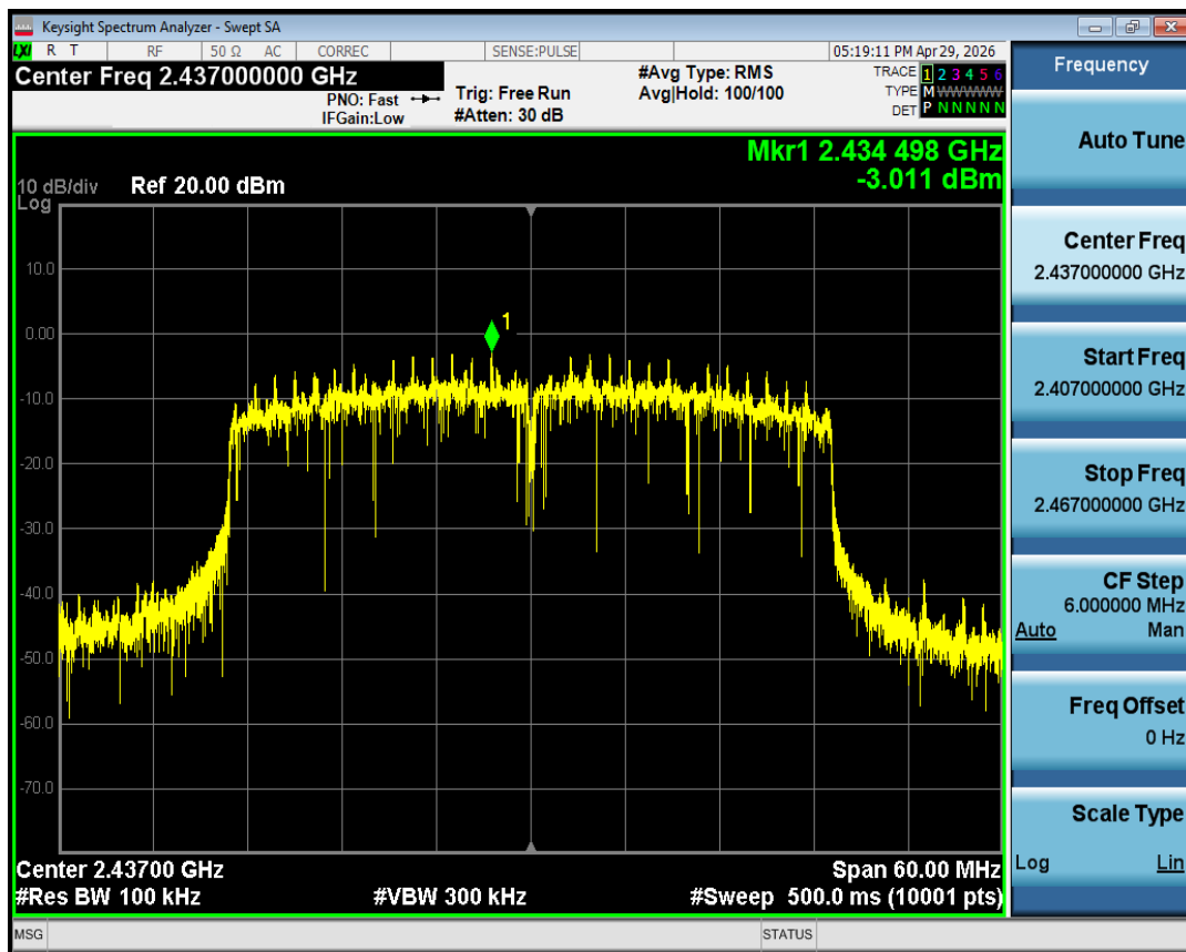
Tx. Spurious NVNT ax40 2437MHz Ant1 Ref
