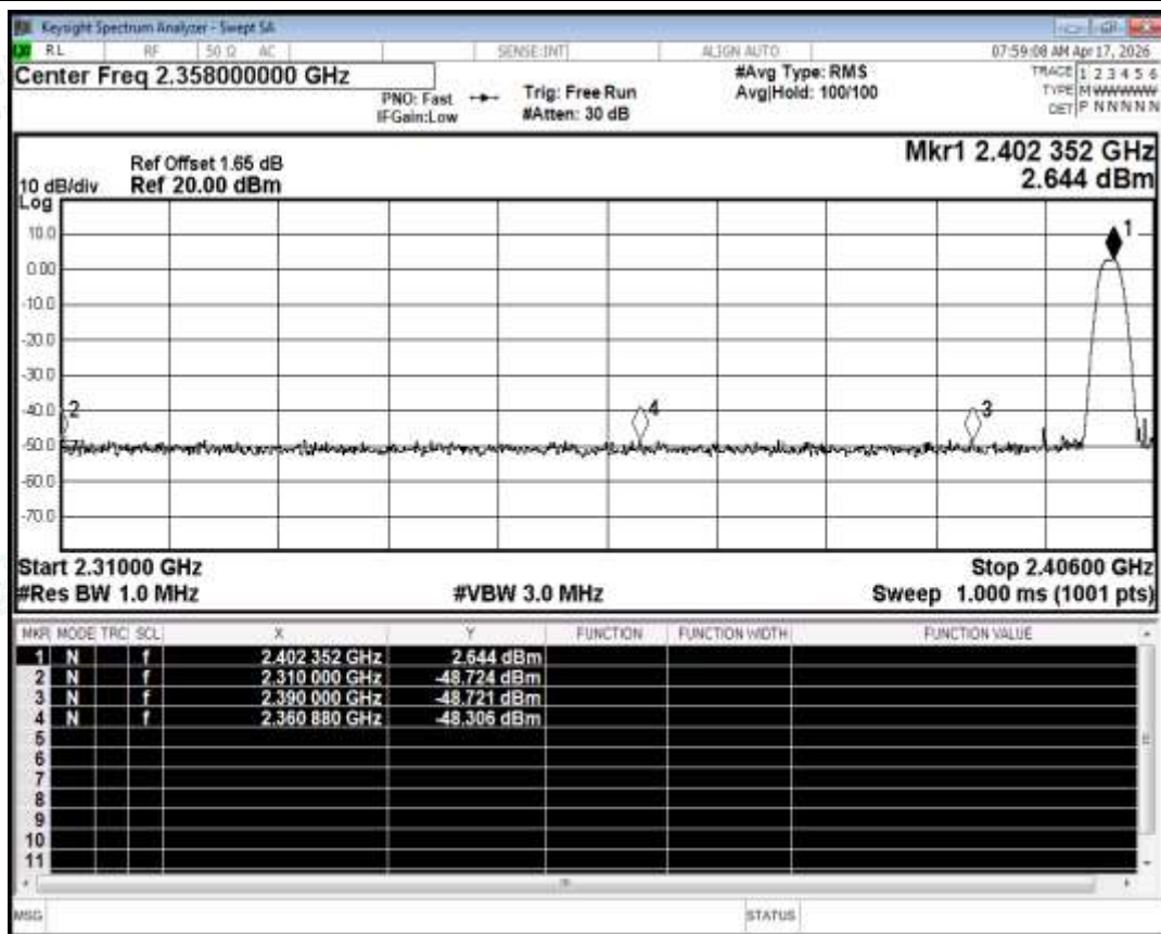
Restrict Band NVNT BLE 2402MHz Ant1 Peak
