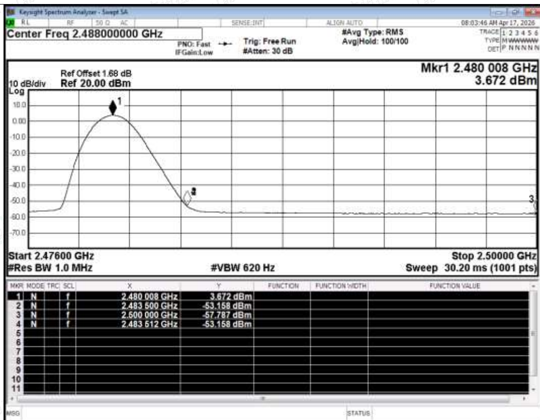
Restrict Band NVNT BLE 2480MHz Ant1 Average
