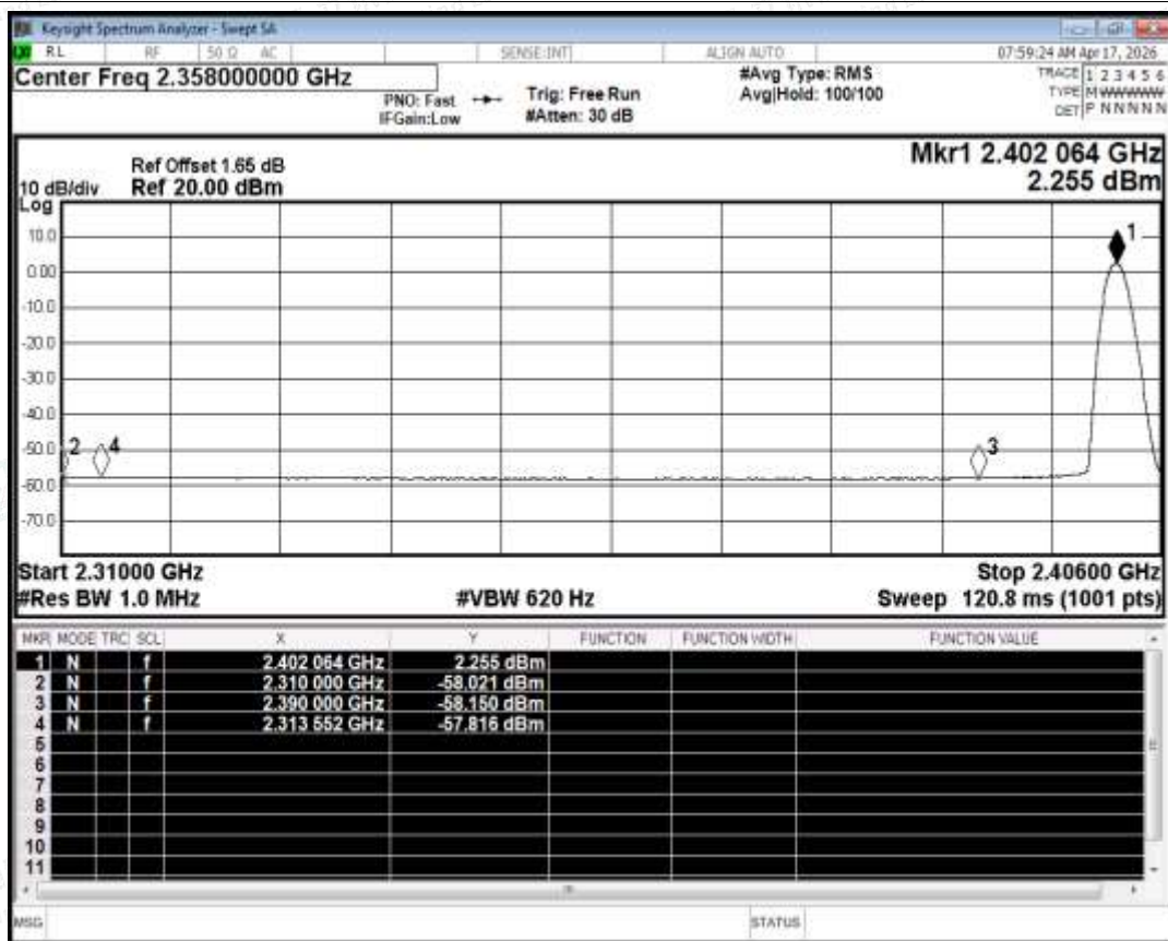
Restrict Band NVNT BLE 2402MHz Ant1 Average
