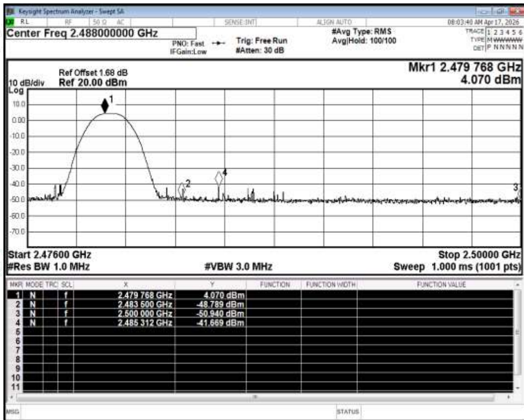
Restrict Band NVNT BLE 2480MHz Ant1 Peak
