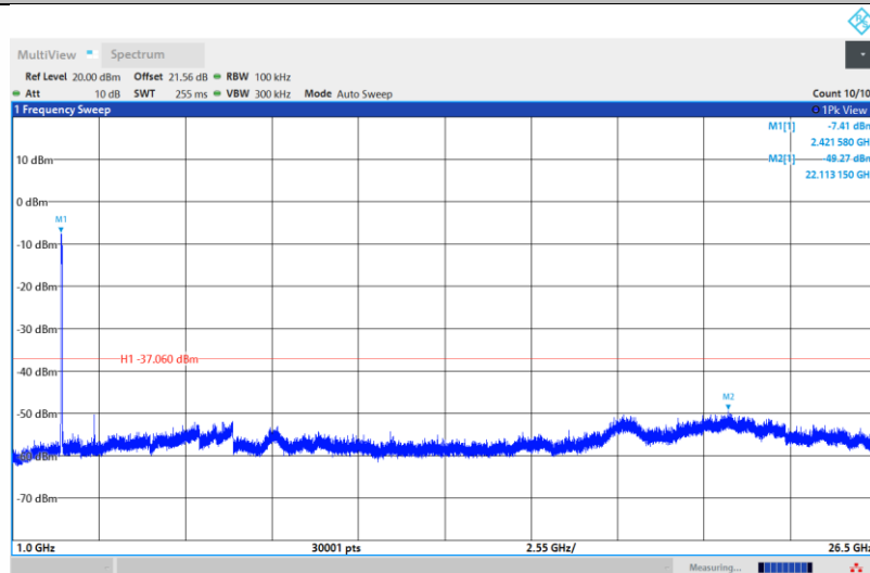
11N40SISO-Ant1-2437-1000~26500-PASS
