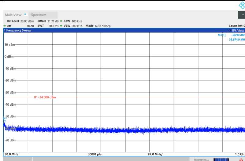
11N20SISO-Ant1-2412-30~1000-PASS
