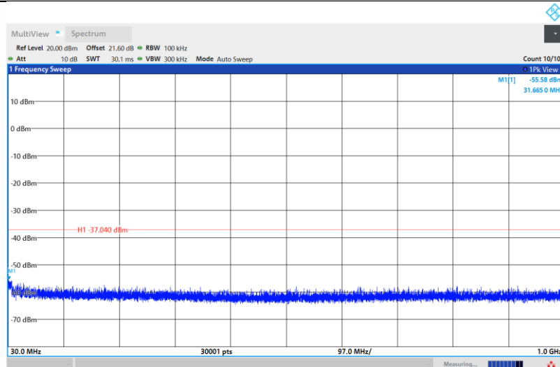
11N40SISO-Ant1-2422-30~1000-PASS
