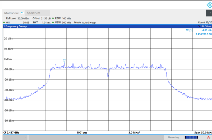
11G-Ant1-2437-0~Reference-PASS
