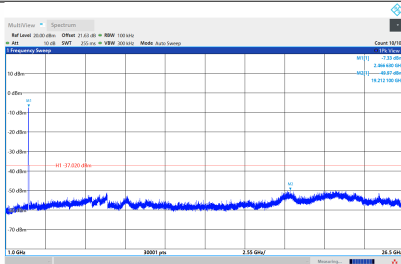
11N40SISO-Ant1-2452-1000~26500-PASS
