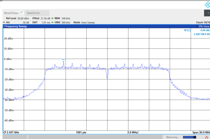
11N20SISO-Ant1-2437-0~Reference-PASS
