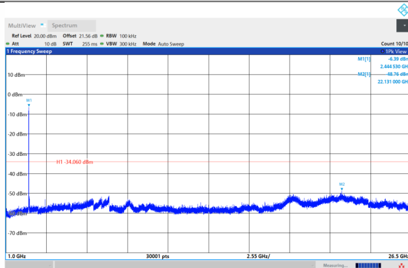
11N20SISO-Ant1-2437-1000~26500-PASS
