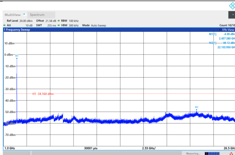
11N20SISO-Ant1-2462-1000~26500-PASS
