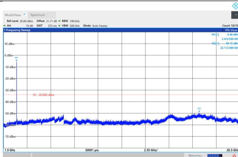
11N20SISO-Ant1-2412-1000~26500-PASS
