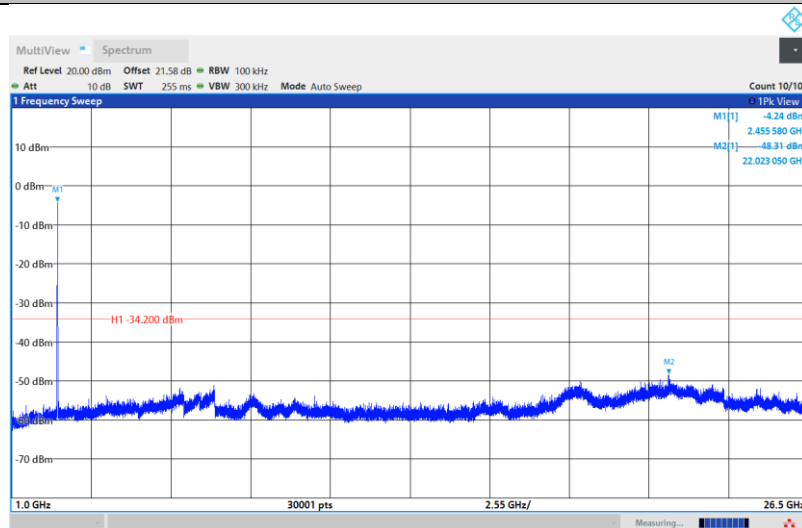
11G-Ant1-2462-1000~26500-PASS
