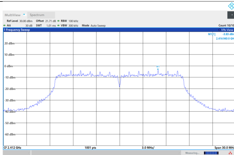
11G-Ant1-2412-0~Reference-PASS
