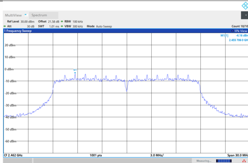
11N20SISO-Ant1-2462-0~Reference-PASS
