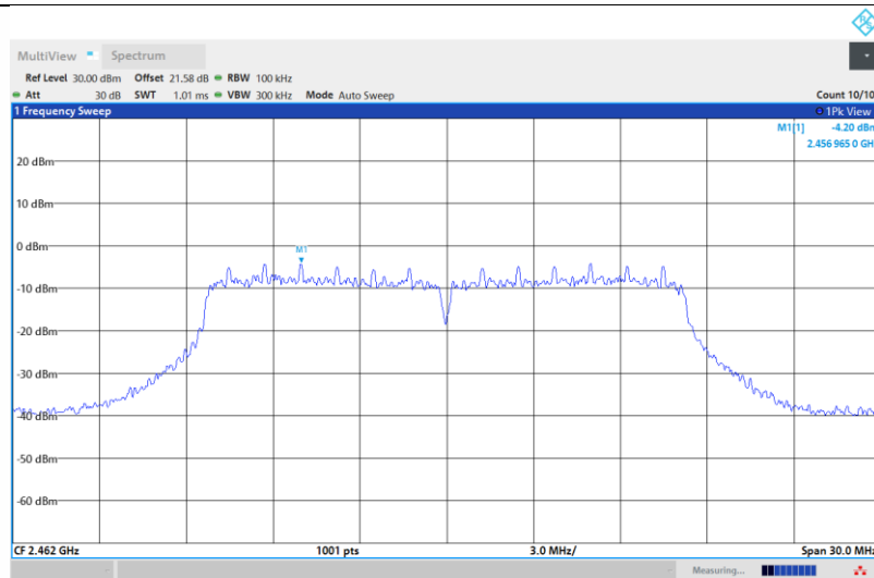
11G-Ant1-2462-0~Reference-PASS
