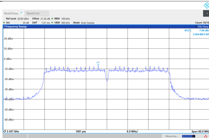
11N40SISO-Ant1-2437-0~Reference-PASS
