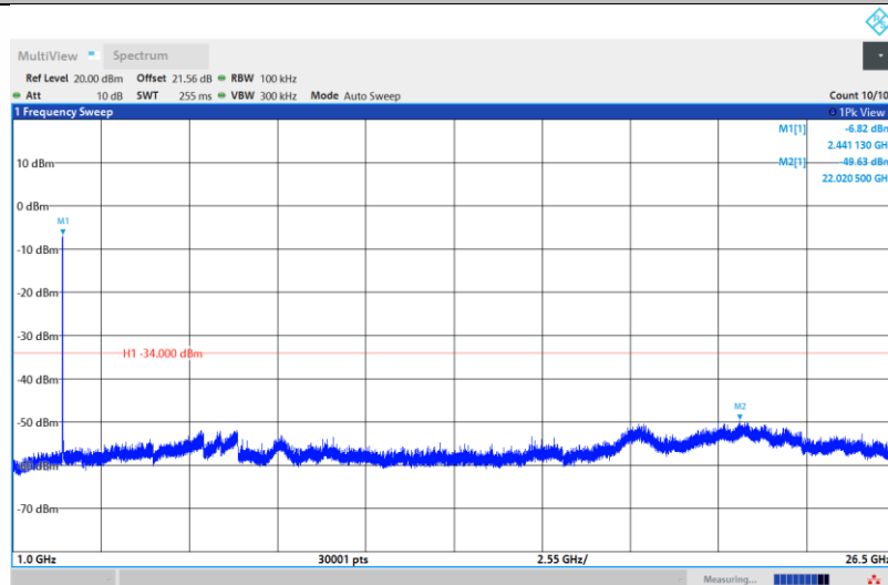
11G-Ant1-2437-1000~26500-PASS
