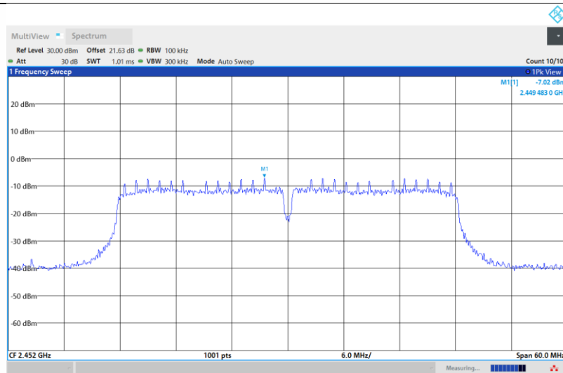
11N40SISO-Ant1-2452-0~Reference-PASS
