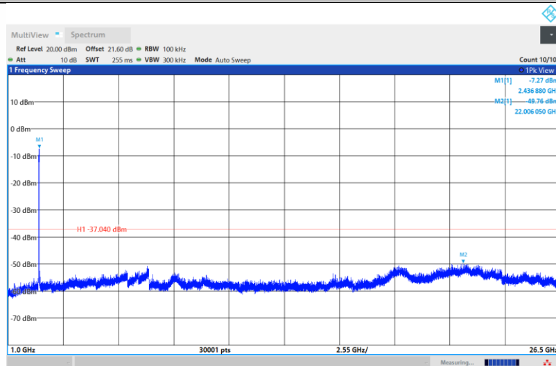
11N40SISO-Ant1-2422-1000~26500-PASS
