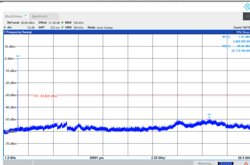
11B-Ant1-2462-1000~26500-PASS
