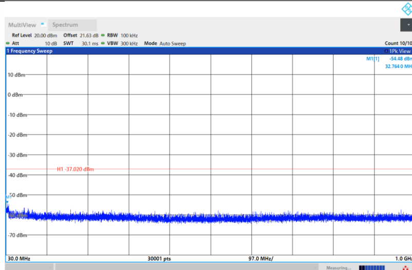
11N40SISO-Ant1-2452-30~1000-PASS
