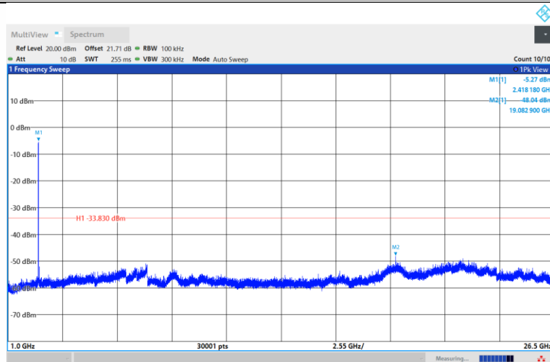
11G-Ant1-2412-1000~26500-PASS
