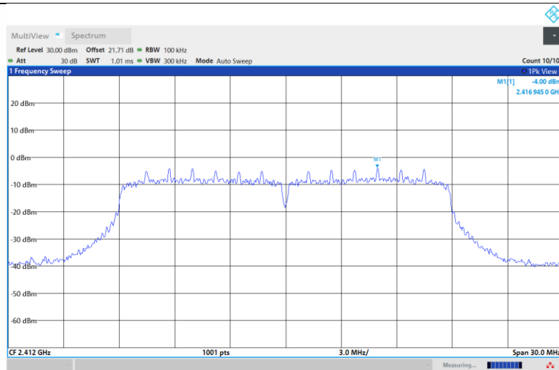
11N20SISO-Ant1-2412-0~Reference-PASS
