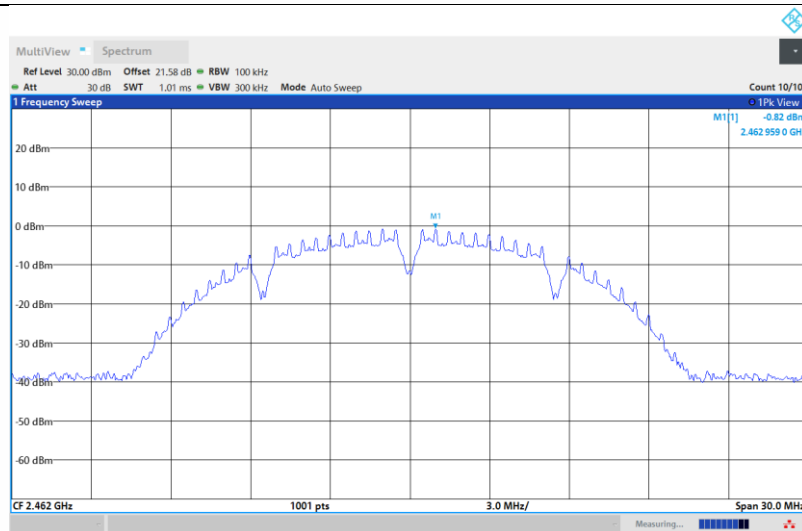
11B-Ant1-2462-0~Reference-PASS
