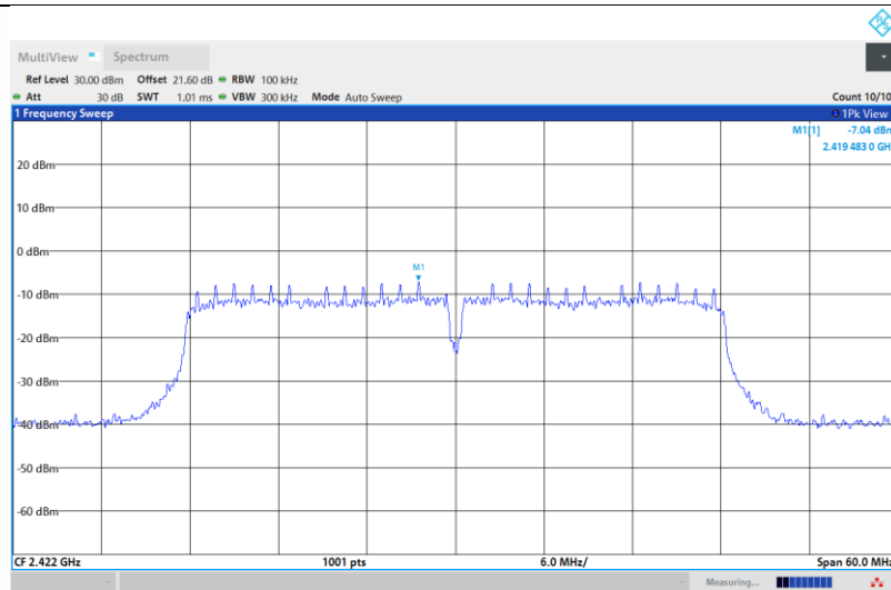
11N40SISO-Ant1-2422-0~Reference-PASS
