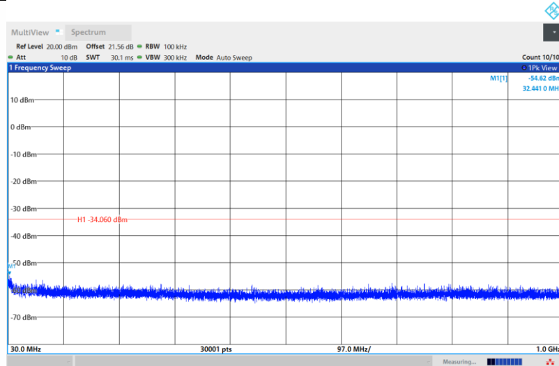
11N20SISO-Ant1-2437-30~1000-PASS
