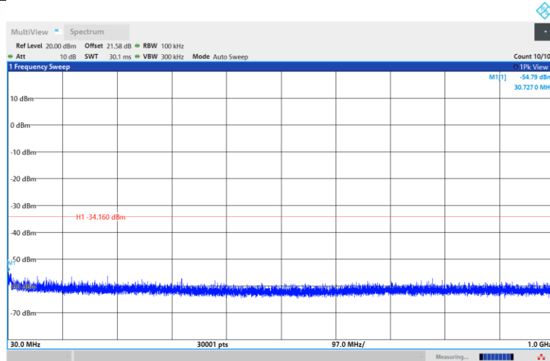
11N20SISO-Ant1-2462-30~1000-PASS
