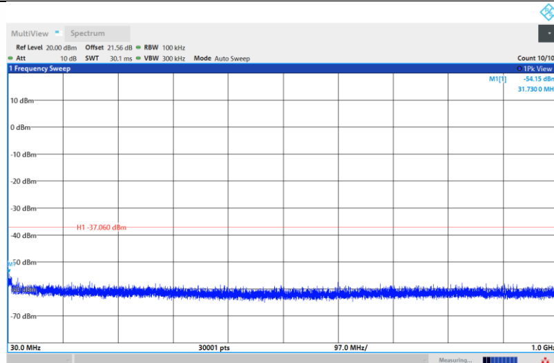
11N40SISO-Ant1-2437-30~1000-PASS
