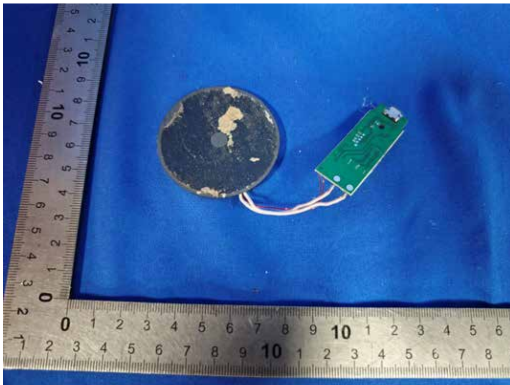
FIGURE 24 FSCR Mix 5.5 x 8.5 WALTON WIRELESS CHARGING JOURNAL (2800-58BK) MAINBOARD BACK
