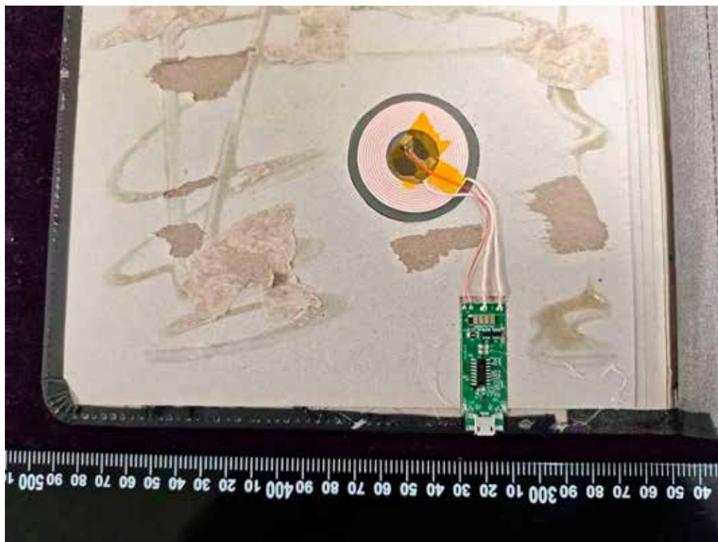
FIGURE 11 FSC MIX VIENNA WIRELESS CHARGING WRITING PAD (0911-07BK) MAINBOARD FRONT
