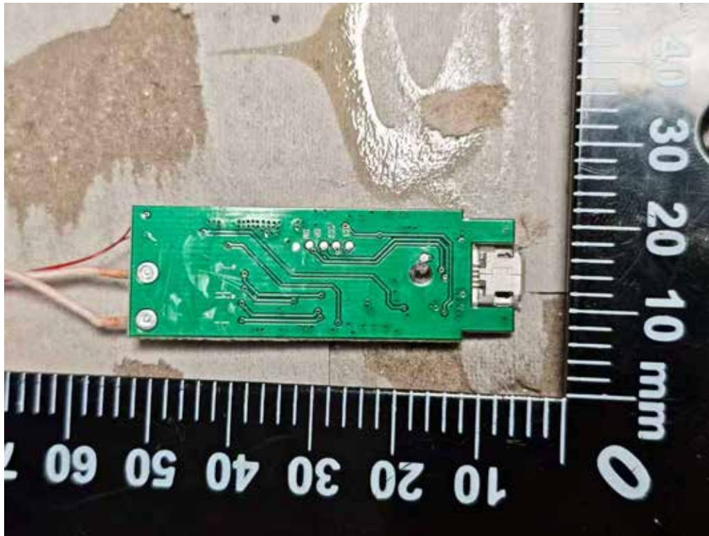
FIGURE 13 FSC MIX VIENNA WIRELESS CHARGING WRITING PAD (0911-07BK) LOOP COIL ANTENNA
