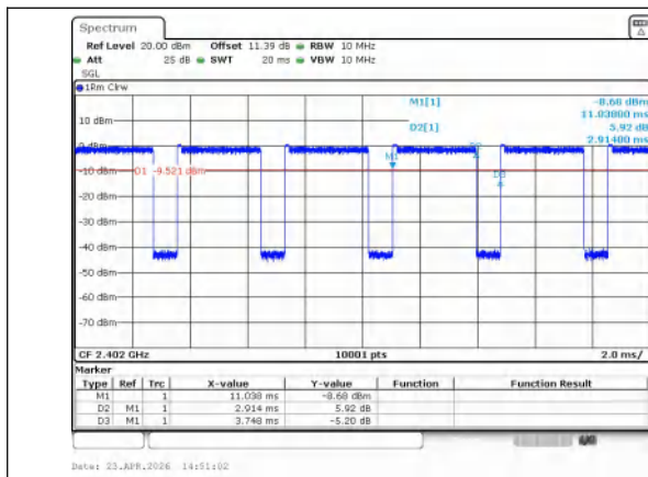
8DPSK(3-DH5)_Channel 0
