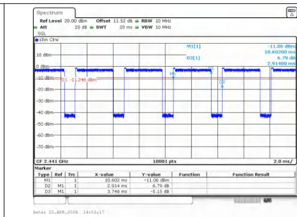
8DPSK(3-DH5)_Channel 39
