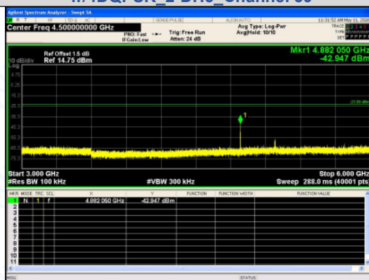
3000.0 MHz - 6000.0 MHz π/4DQPSK 2-DH5 Channel 39
