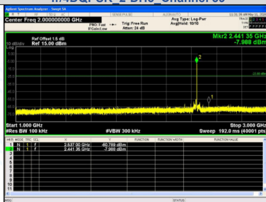
1000.0 MHz - 3000.0 MHz π/4DQPSK 2-DH5 Channel 39
