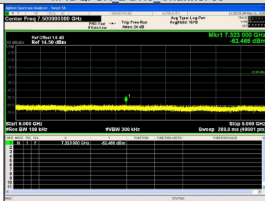
6000.0 MHz - 9000.0 MHz π/4DQPSK 2-DH5 Channel 39
