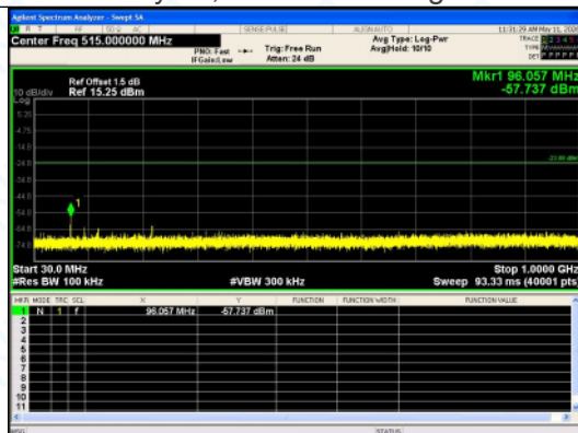
30.0 MHz - 1000.0 MHz π/4DQPSK 2-DH5 Channel 39
