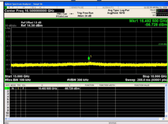
15000.0 MHz - 18000.0 MHz π/4DQPSK 2-DH5 Channel 39
