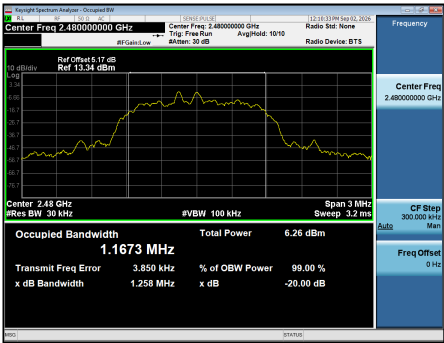
-20dB_Bandwidth_NVNT_ANT1_2-DH1_2480_00
