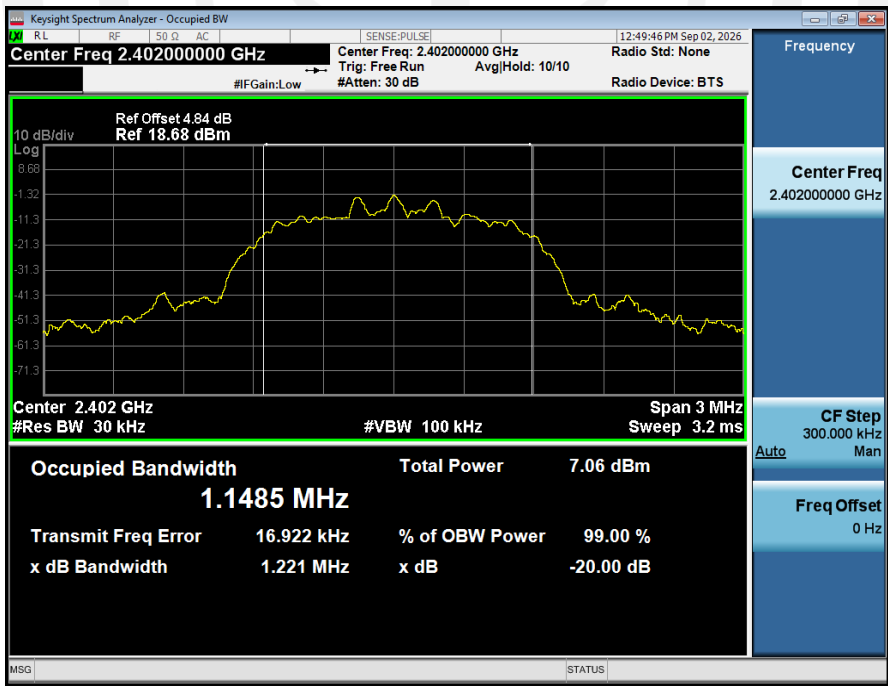
-20dB_Bandwidth_NVNT_ANT1_3-DH1_2402_00
