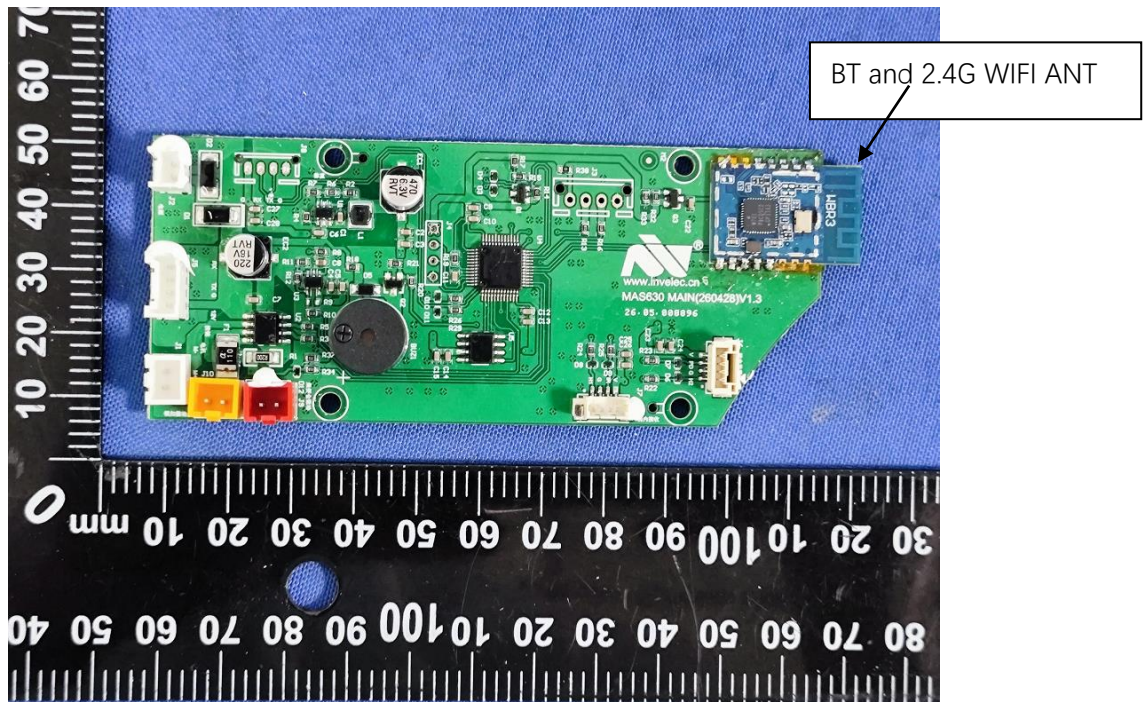
Main PCB view
