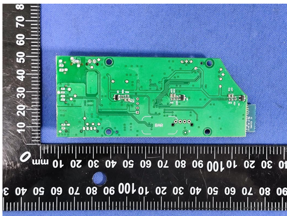
Main PCB view
