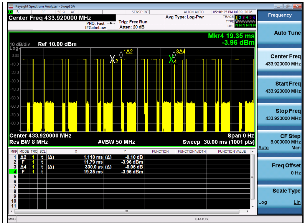
Test_Graph_Short Pulse_Pulse Type 1&2
