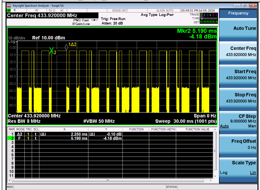
Test_Graph_Short Pulse_Pulse Type 3
