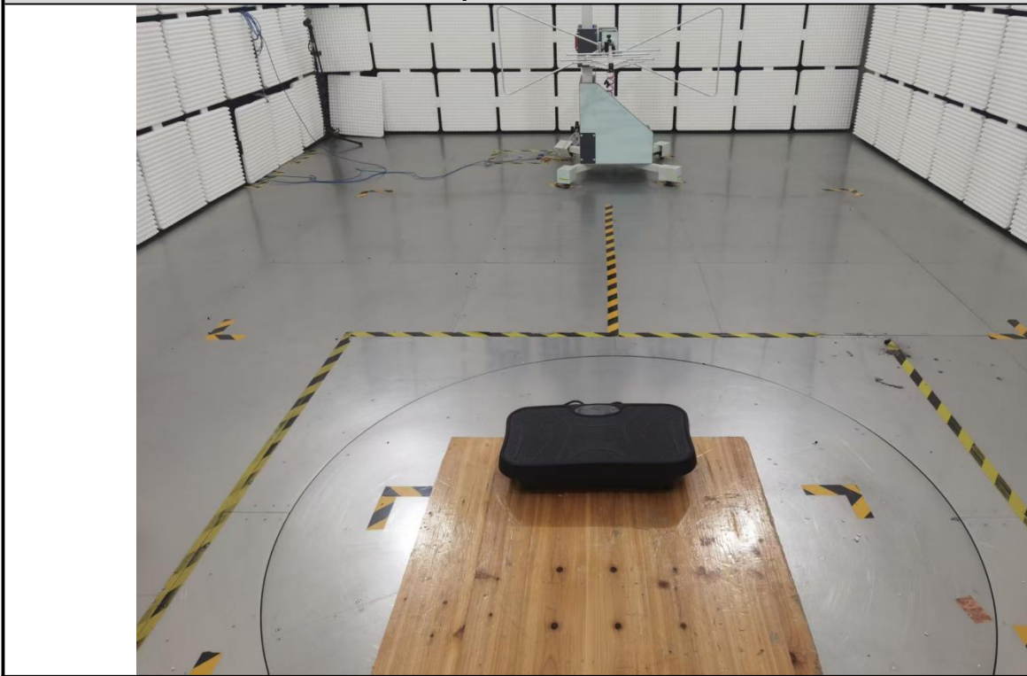
Radiated Spurious Emission, Below 1GHz
