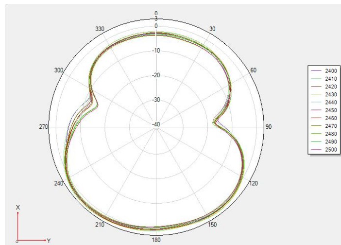
Theta 90 2D
