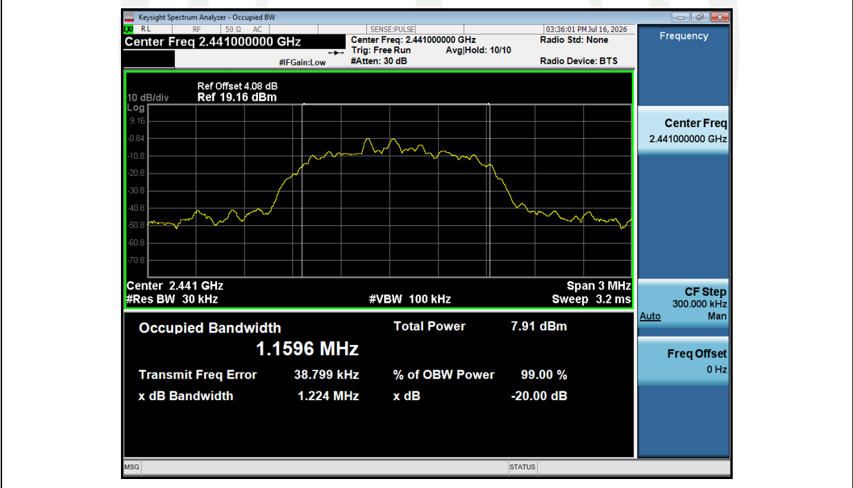
-20dB_Bandwidth_NVNT_ANT1_3-DH1_2441_00
