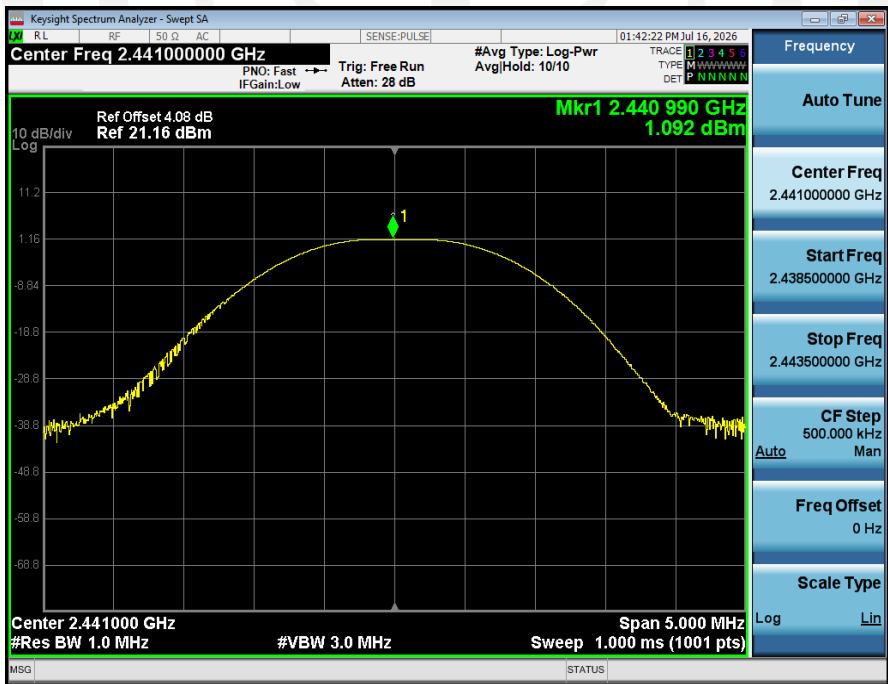
Peak_Output_Power_NVNT_ANT1_1-DH1_2441_00
