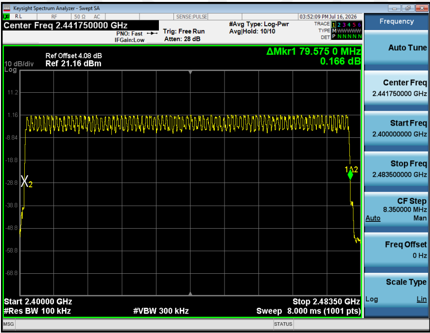
Number_of_Hopping_Channel_(Hopping)_NVNT_ANT1_3-DH1_Hopping
