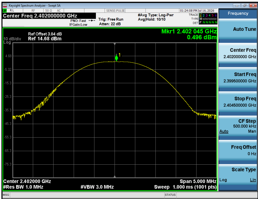
Peak_Output_Power_NVNT_ANT1_1-DH1_2402_00
