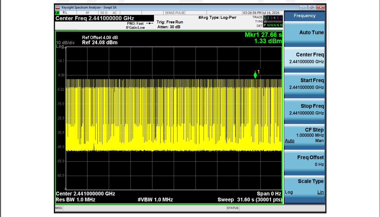
Dwell_Time_(Hopping)_NVNT_ANT1_2-DH1_2441_00_Accumulated
