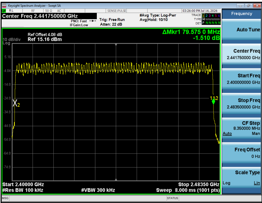
Number_of_Hopping_Channel_(Hopping)_NVNT_ANT1_2-DH1_Hopping
