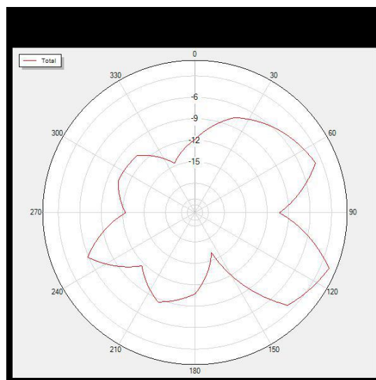
2420P0 Total
