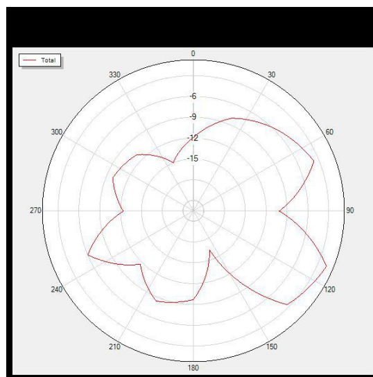
2440P0 Total
