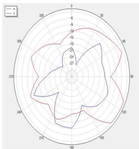
2500P0 Polar
