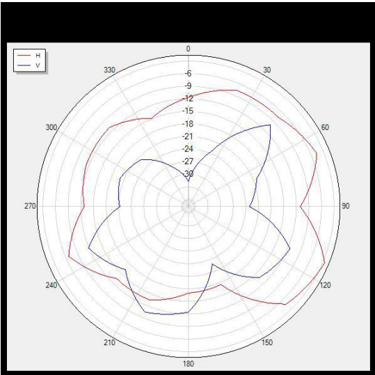
2400P0 Polar
