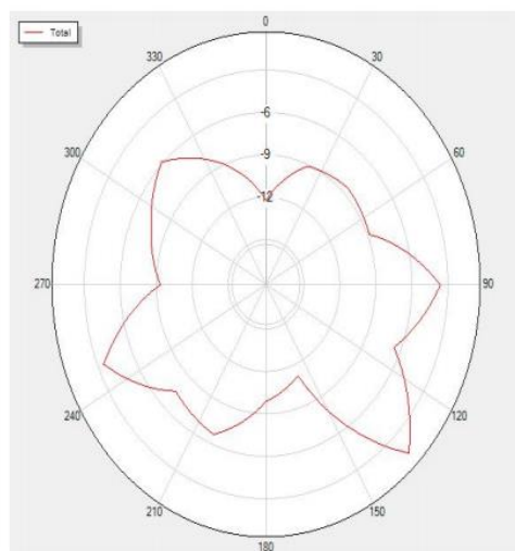
2490P90 Total
