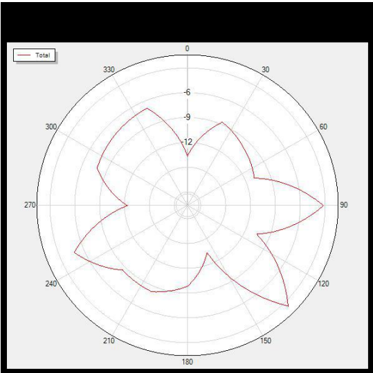
2400P90 Total
