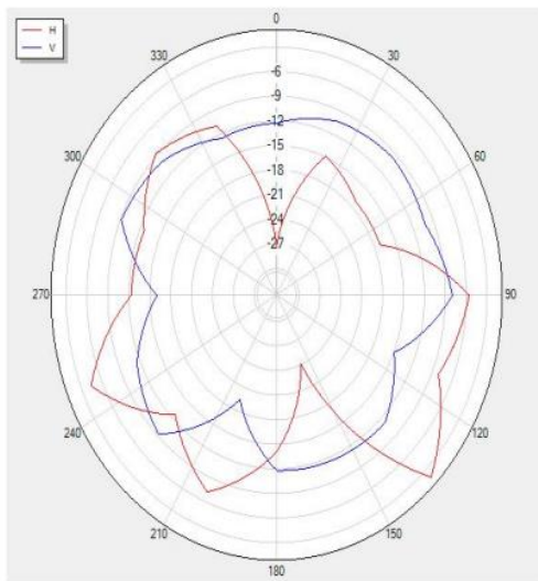
2470P90 Polar
