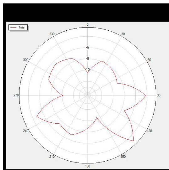
2440P90 Total
