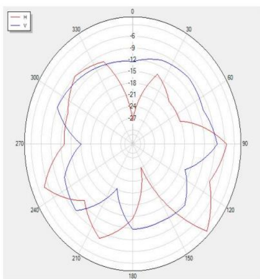
2450P90 Polar
