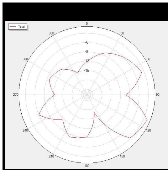
2450P0 Total
