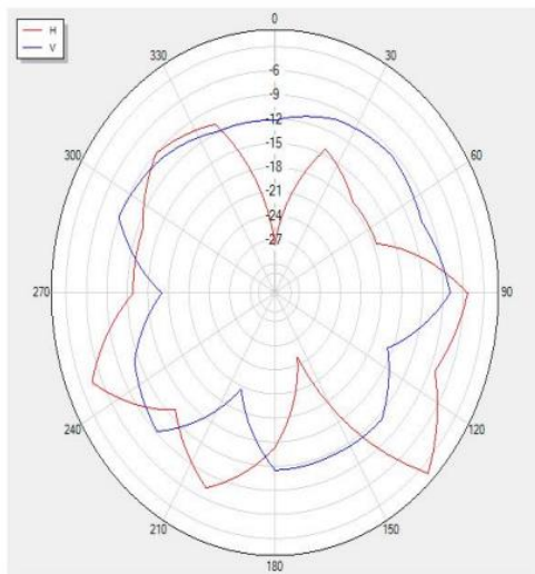
2460P90 Polar
