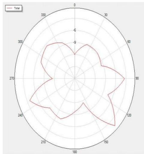
2460P90 Total
