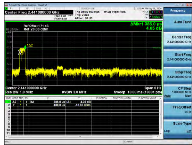
Burst(2DH1)
