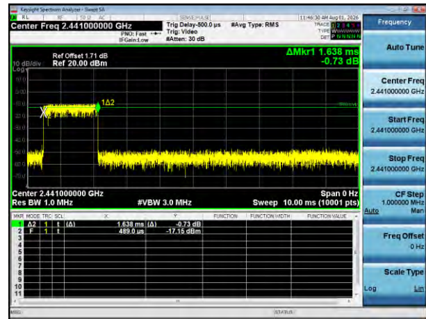
Burst(2DH3)
