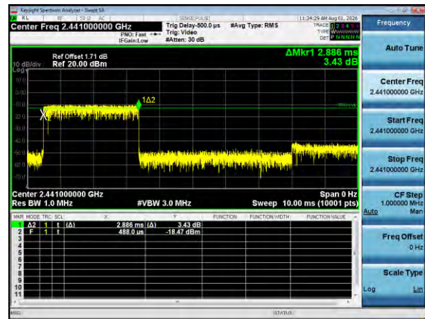
Burst(2DH5)
