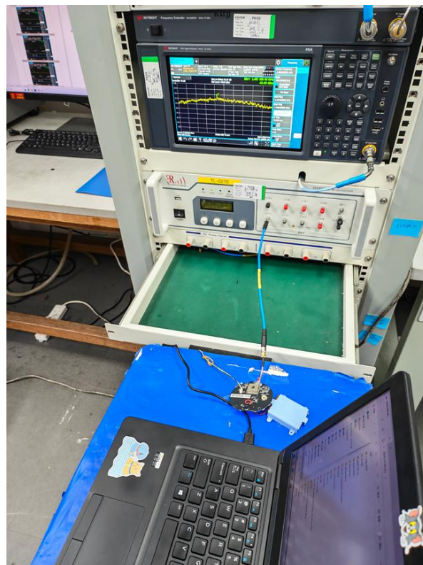
RF conducted test
