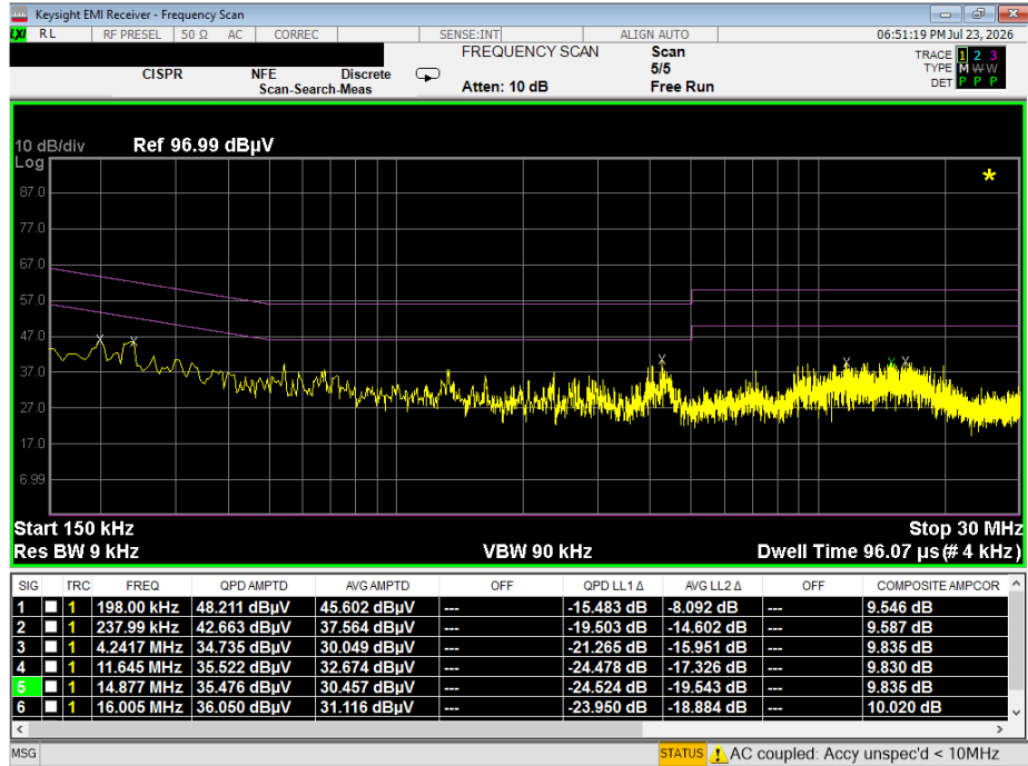
Plot 7-3. Line Conducted Plot (L1)
