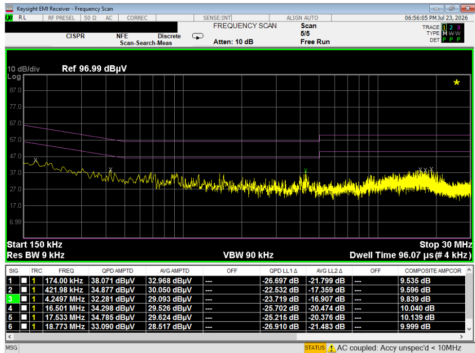
Plot 7-4. Line Conducted Plot (N)
