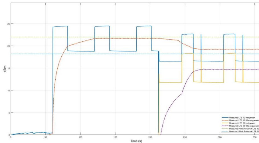
Figure 11.10-1 Conducted Tx power for LTE B12/LTE B66 inter-band ULCA in test TC15
