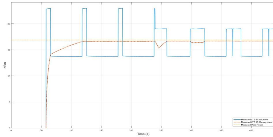
Figure 11.3-1 Time average conducted power of LTE B66 in TC01
