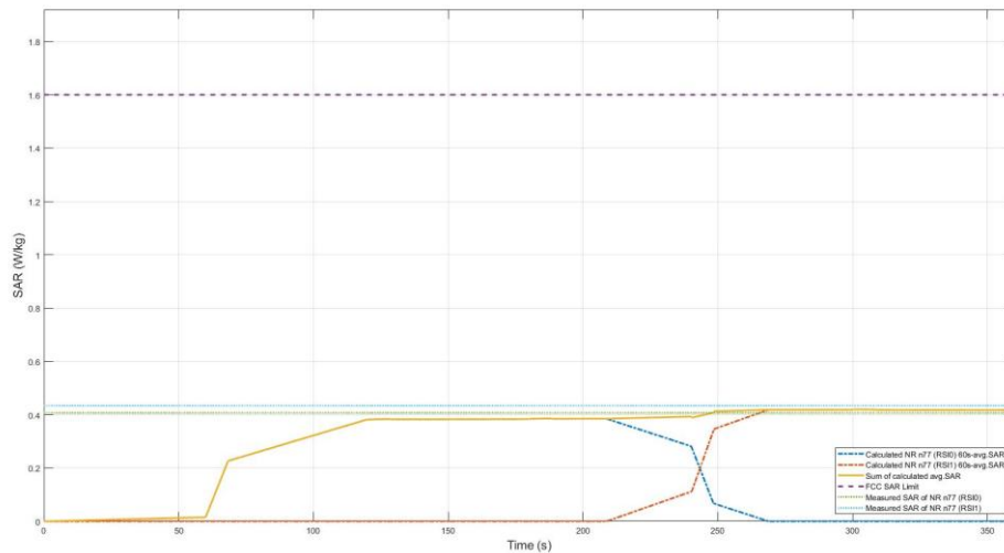
Figure 11.9-2 Total time-averaged SAR in TC14
