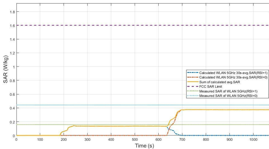
Figure 11.9-6 Total time-averaged SAR in WTC01
