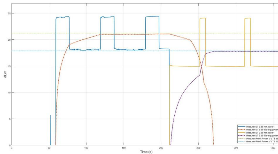
Figure 11.7-1 Conducted Tx power for antenna switching in test TC12 [LTE 26 to LTE 25]
