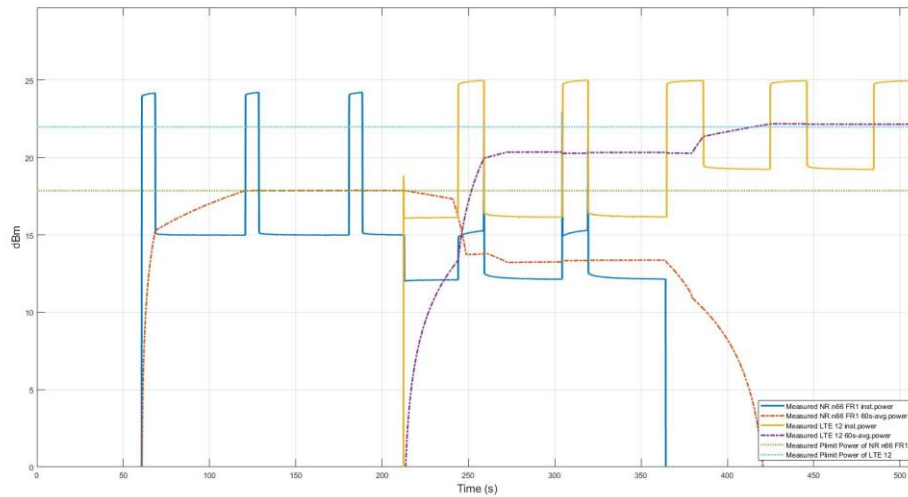
Figure 11.8-1 Conducted Transmitted power for LTE B12 and NR n66 in test TC13
