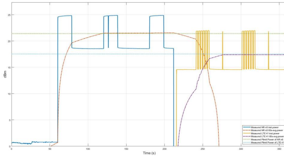
Figure 11.6-1 Conducted Tx power for SAR IRAT re-selection in test TC11 [n5 to LTE B41]
