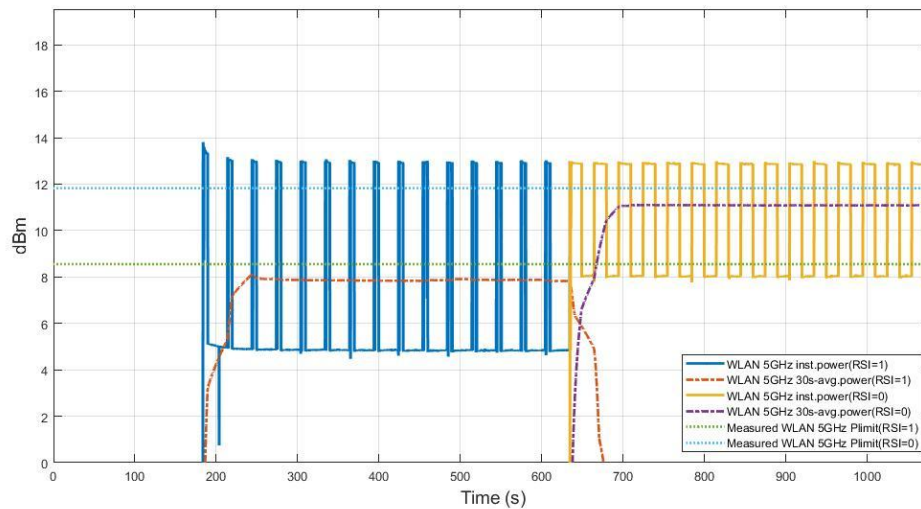
Figure 11.9-5 Conducted Tx power for WLAN 5GHz in WTC02
