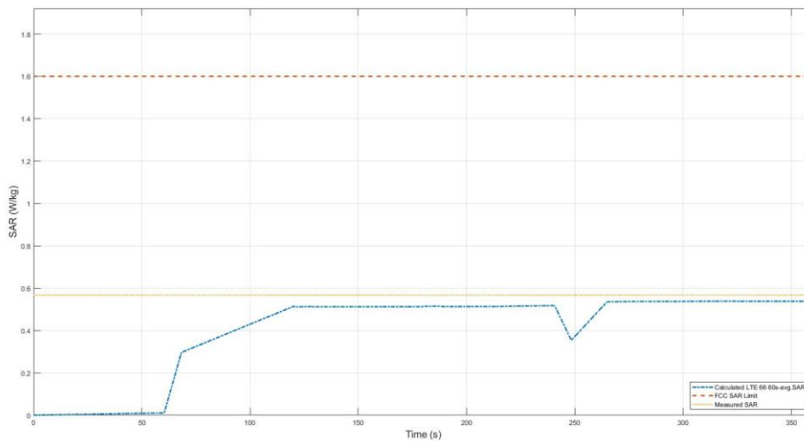
Figure 11.5-2 Total time-averaged SAR in TC10
