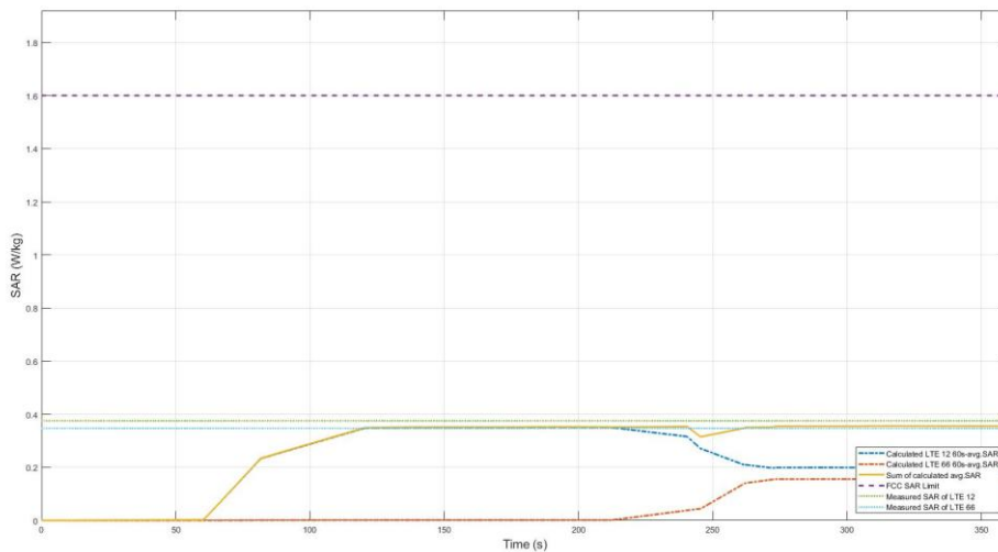
Figure 11.10-2 Total time-averaged SAR in TC16
