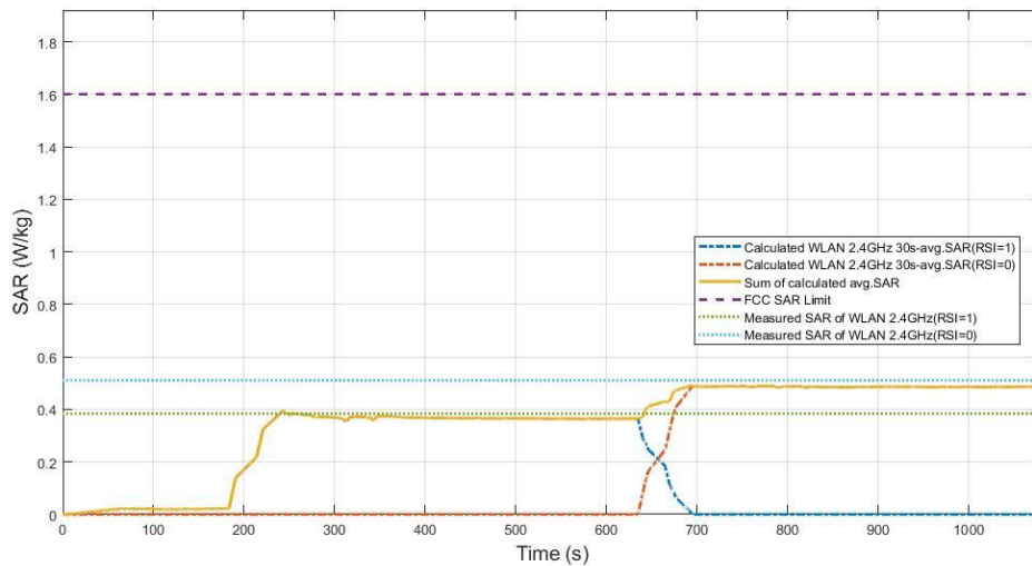
Figure 11.9-4 Total time-averaged SAR in WTC01
