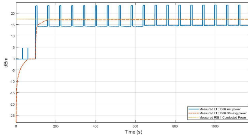
Figure 11.5-1 Conducted Tx power in SAR Modulation Change in test LTE Band 66 case TC10
