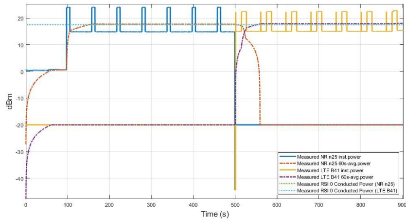
Figure 11.6-1 Conducted Tx power for SAR IRAT re-selection in test TC11 [n25 to LTE B41]
