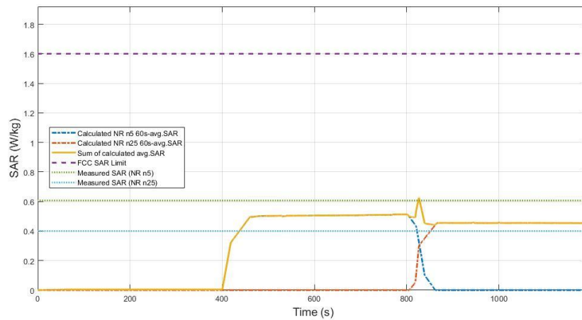
Figure 11.7-2 Total time-averaged SAR in TC12
