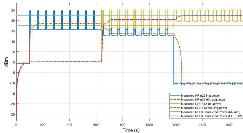
Figure 11.8-1 Conducted Transmitted power for LTE B12 and NR n25 in test TC13
