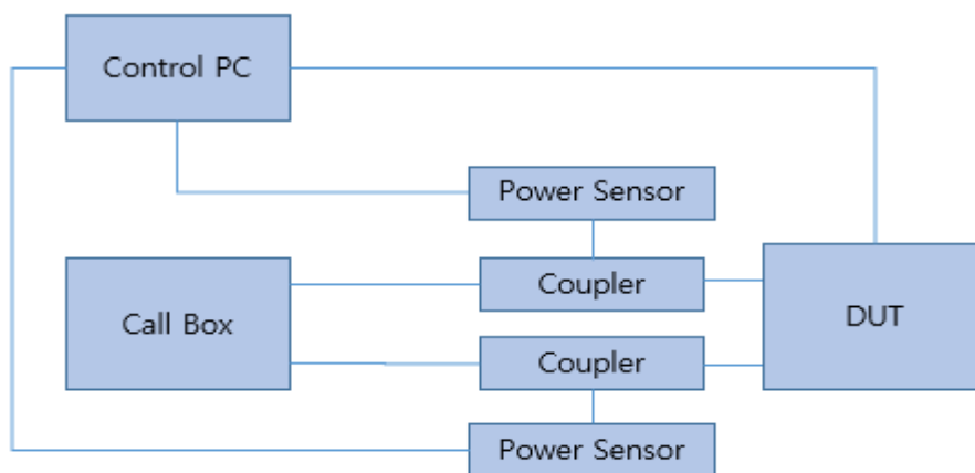
Figure 11.1-2 Test set-up for WLAN and Bluetooth
