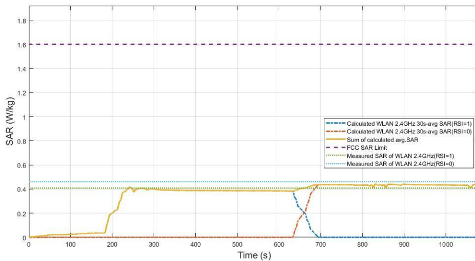
Figure 11.3-18 Total time-averaged SAR in WTC01
