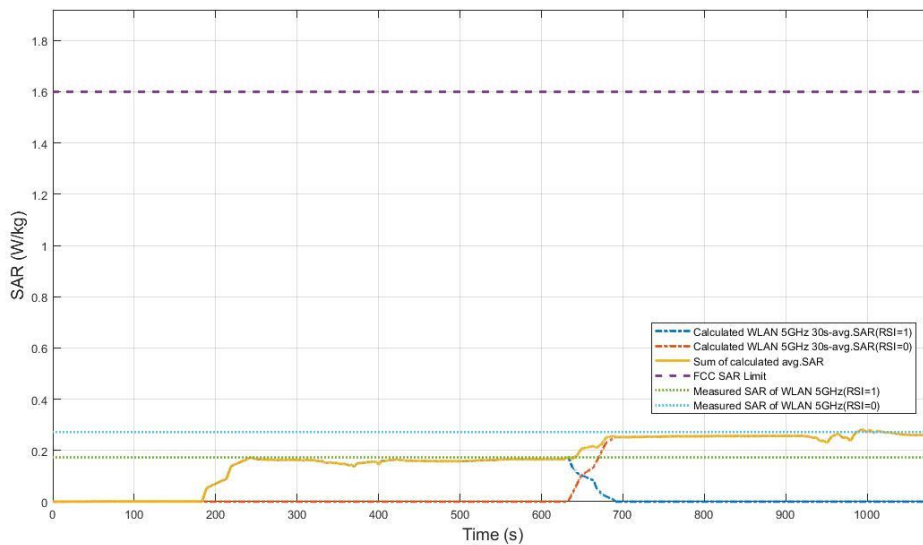
Figure 11.3-20 Total time-averaged SAR in WTC01
