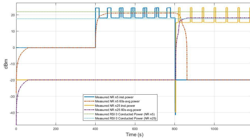
Figure 11.7-1 Conducted Tx power for antenna switching in test TC12 [n5 to n25]
