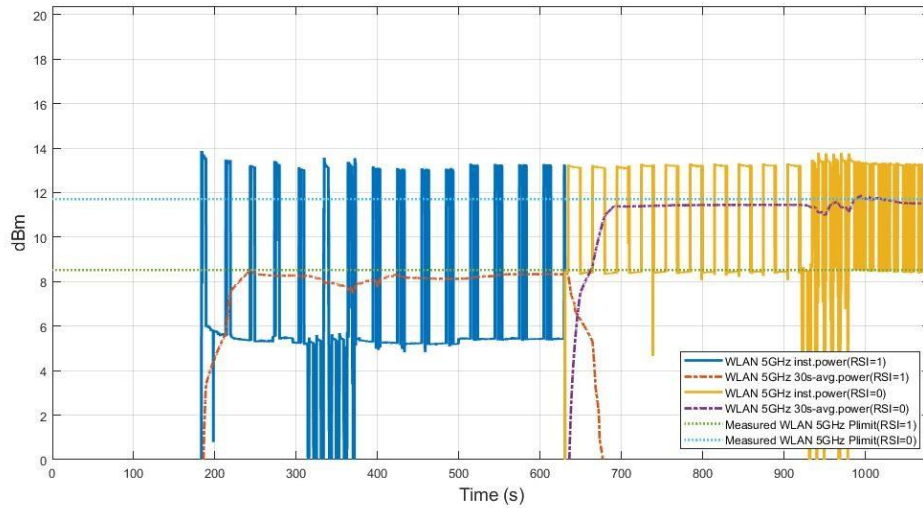
Figure 11.3-19 Conducted Tx power for WLAN 5GHz in WTC02
