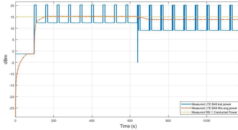
Figure 11.11-1 Conducted Tx power for LTE B48 intra-band ULCA in test TC16
