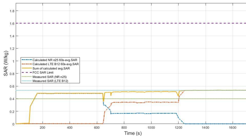
Figure 11.8-2 Total time-averaged SAR LTE B12 and NR n25 in TC13
