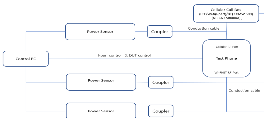
Figure 11.1-3 Test set-up for C-TAS
