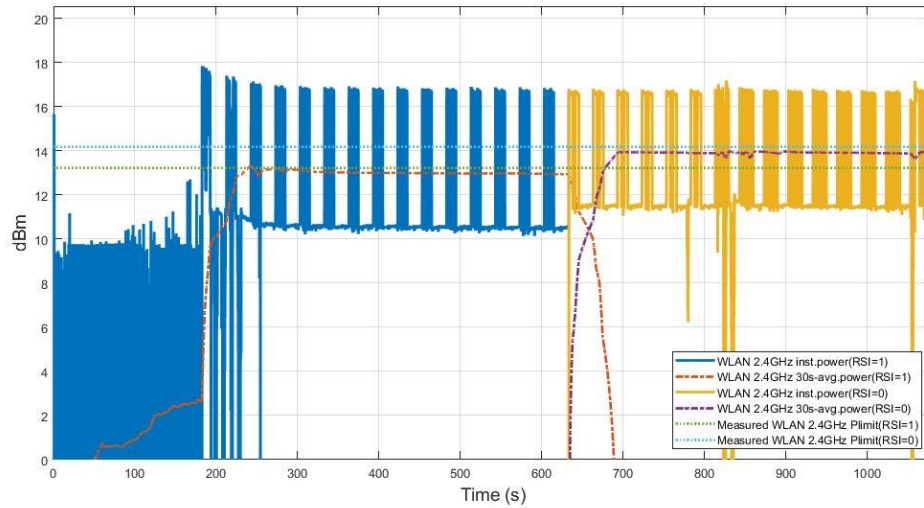
Figure 11.3-17 Conducted Tx power for WLAN 2.4GHz in WTC01
