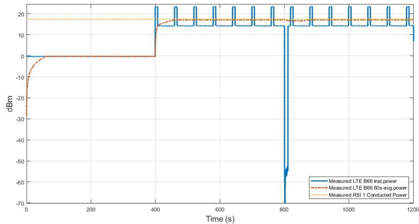
Figure 11.4-1 Conducted Tx power in Call_Disconnect_Reestablishment LTE Band 66 case TC09
