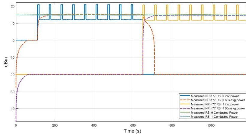
Figure 11.9-1 Conducted Tx power for SAR RSI change in test TC14 [NR n77]
