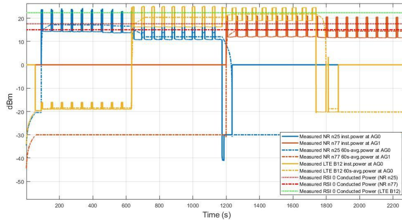
Figure 11.10-1 Conducted Transmitted power for LTE B12(AG0) and NR n25(AG0), n77(AG1) in Test TC15
