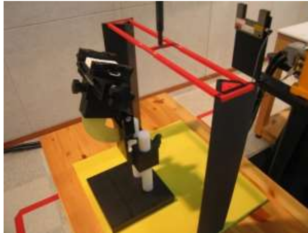
Figure 2. HAC Phantom & Device Holder
