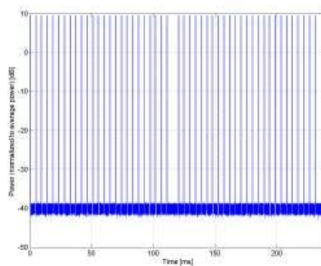
Time Domain
