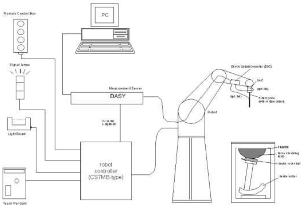
Figure 1. HAC Test Measurement Set-up
