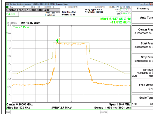
6165 MHz CHAIN 0
