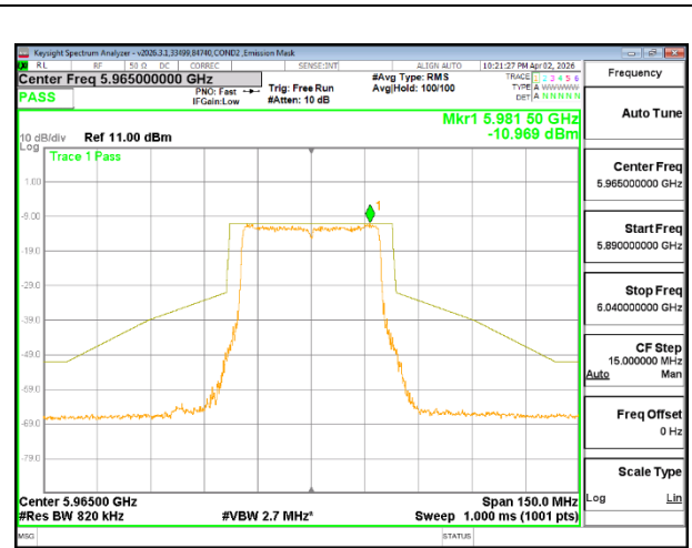
5965 MHz CHAIN 1
