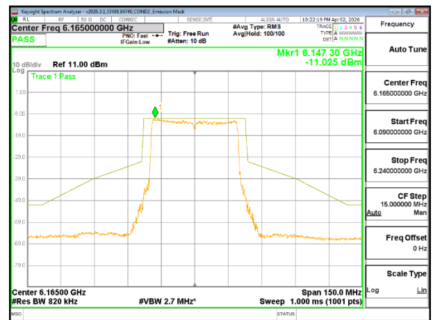
6165 MHz CHAIN 1
