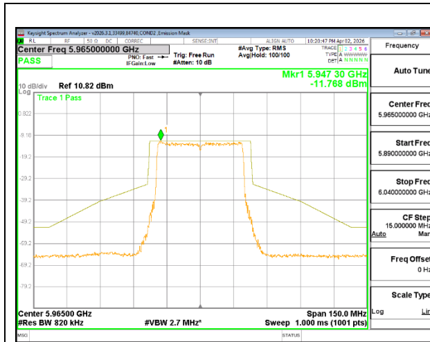
5965 MHz CHAIN 0
