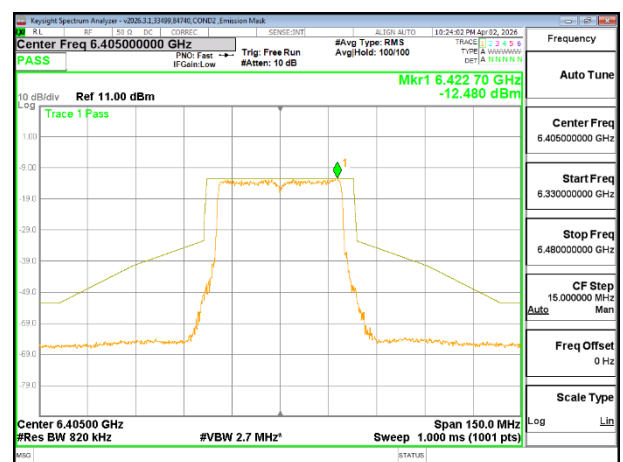
6405 MHz CHAIN 1
