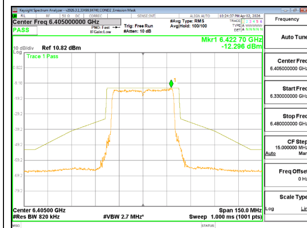
6405 MHz CHAIN 0
