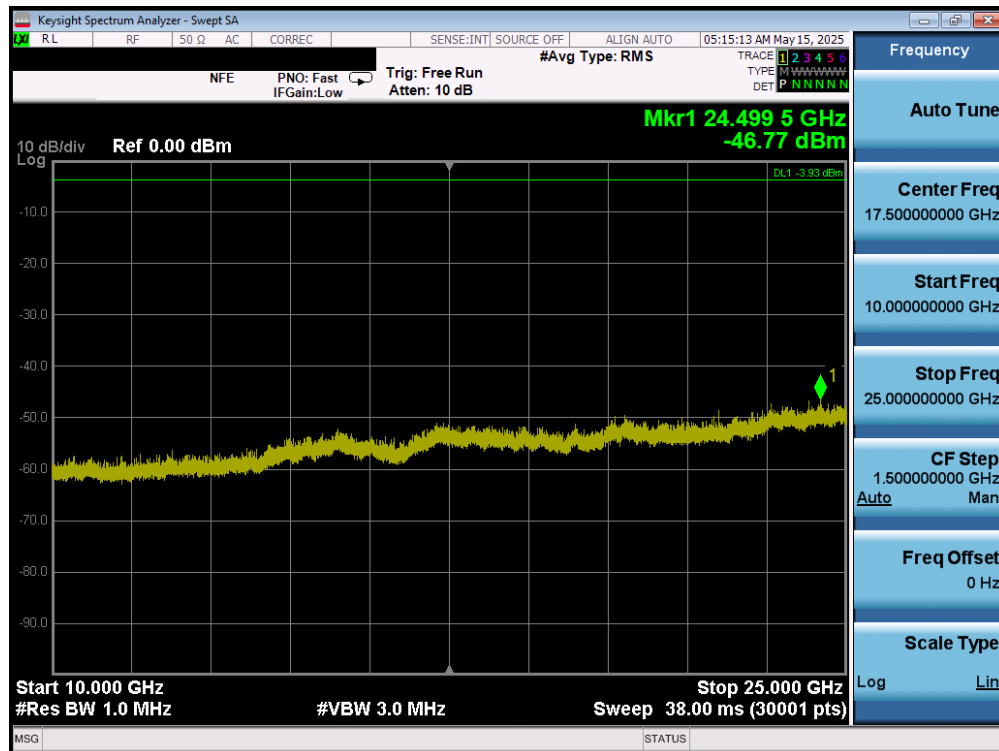
Plot 7-134. Conducted Spurious Plot (Bluetooth (LE), 1Mbps – Ch. 17) – Ant 2
