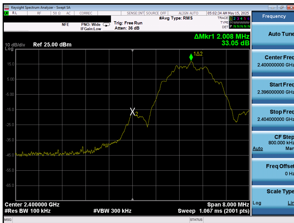
Plot 7-111. Band Edge Plot (Bluetooth (LE), 2Mbps – Ch. 37) – Ant 1
