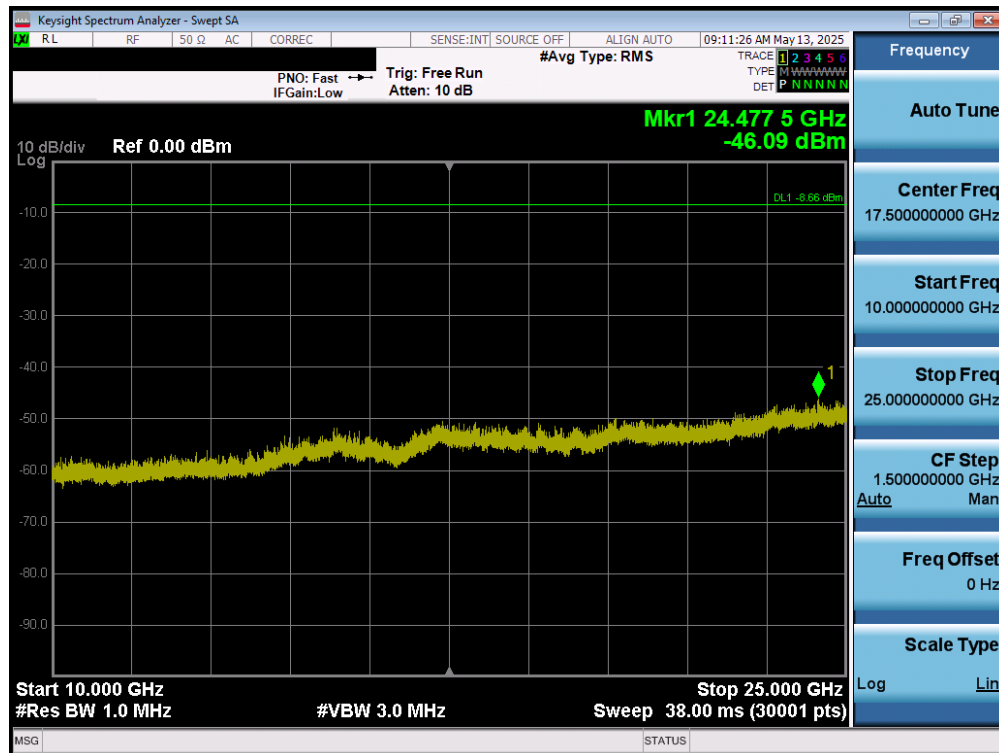
Plot 7-146. Conducted Spurious Plot (Bluetooth (LE), 1Mbps – Ch. 17) – Dual Ant 2
