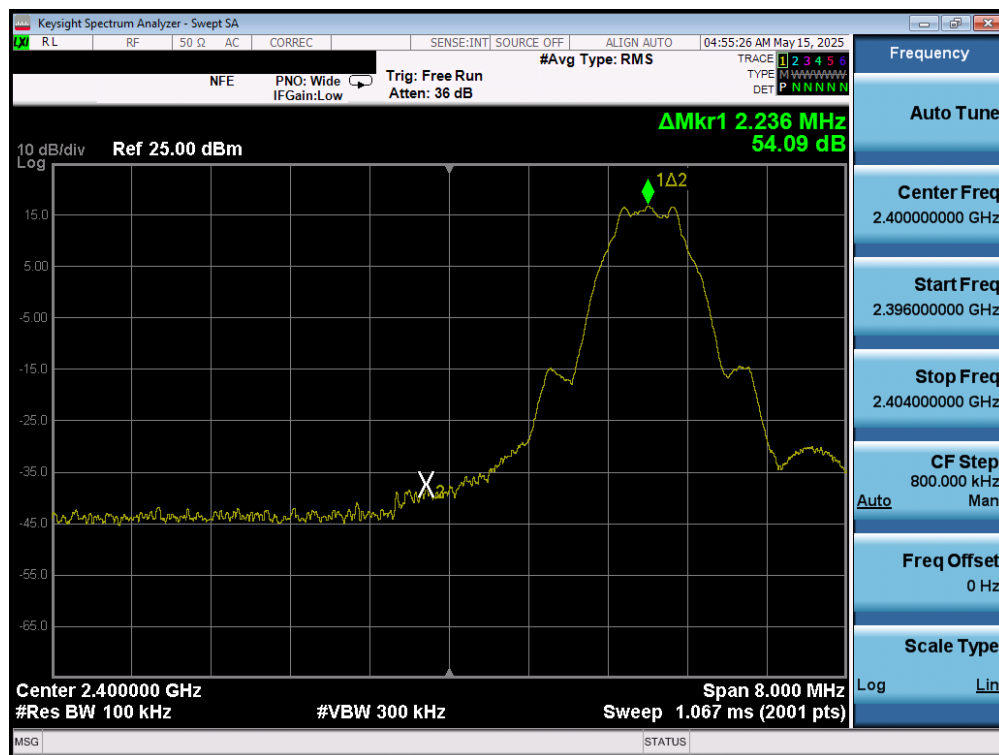
Plot 7-109. Band Edge Plot (Bluetooth (LE), 1Mbps – Ch. 37) – Ant 1
