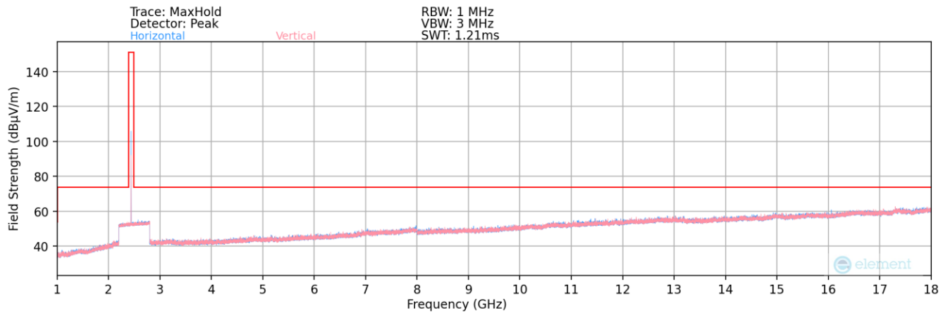
Plot 7-153. Radiated Spurious Plot above 1GHz (Bluetooth (LE) – Ch. 17) – Ant 2
