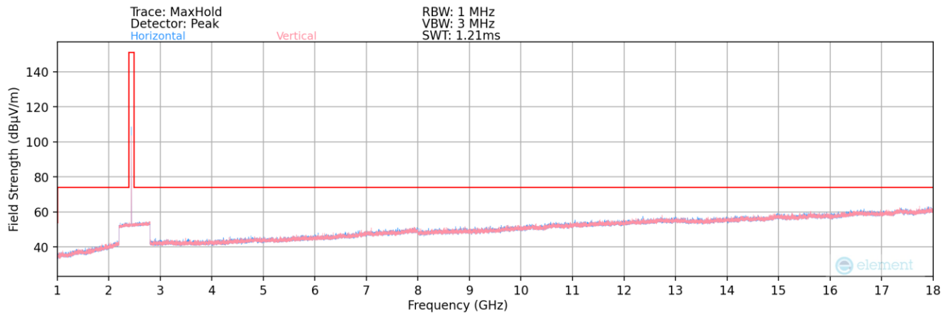
Plot 7-156. Radiated Spurious Plot above 1GHz (Bluetooth (LE) – Ch. 17) – Dual Ant
