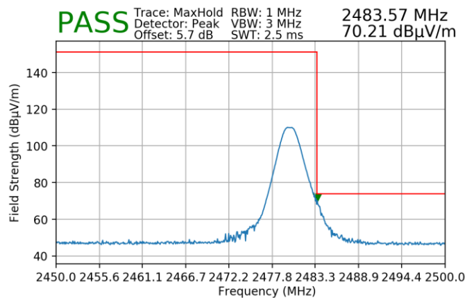
Plot 7-163. Radiated Restricted Upper Band Edge Measurement (Peak) – Dual Ant
