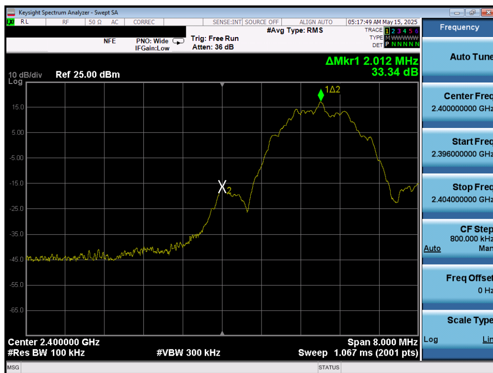
Plot 7-115. Band Edge Plot (Bluetooth (LE), 2Mbps – Ch. 37) – Ant 2
