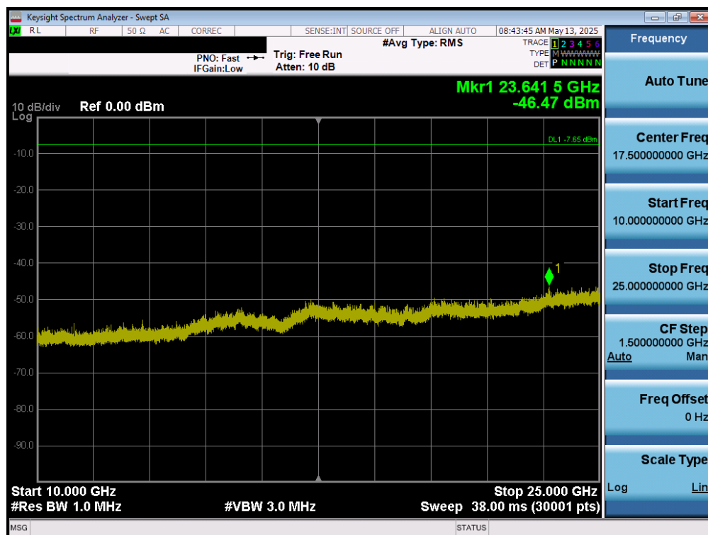
Plot 7-142. Conducted Spurious Plot (Bluetooth (LE), 1Mbps – Ch. 39) – Dual Ant 1
