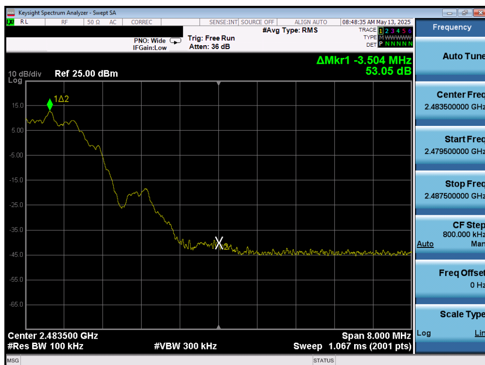
Plot 7-120. Band Edge Plot (Bluetooth (LE), 2Mbps – Ch. 39) – Dual Ant 1
