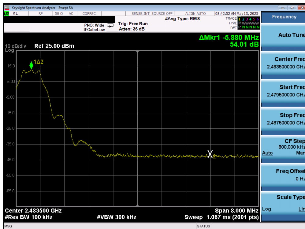
Plot 7-118. Band Edge Plot (Bluetooth (LE), 1Mbps – Ch. 39) – Dual Ant 1
