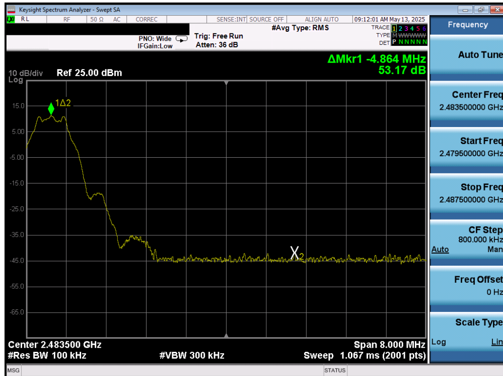
Plot 7-122. Band Edge Plot (Bluetooth (LE), 1Mbps - Ch. 39) - Dual Ant 2
