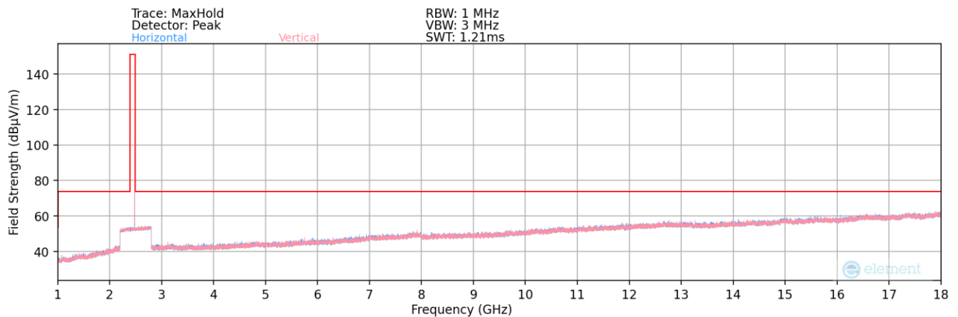
Plot 7-154. Radiated Spurious Plot above 1GHz (Bluetooth (LE) – Ch. 39) – Ant 2
