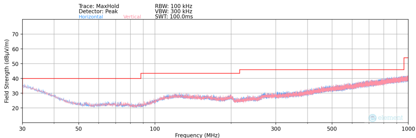
Plot 7-166. Radiated Spurious Plot below 1GHz – Dual Ant
