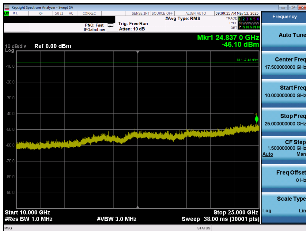
Plot 7-144. Conducted Spurious Plot (Bluetooth (LE), 1Mbps – Ch. 37) – Dual Ant 2
