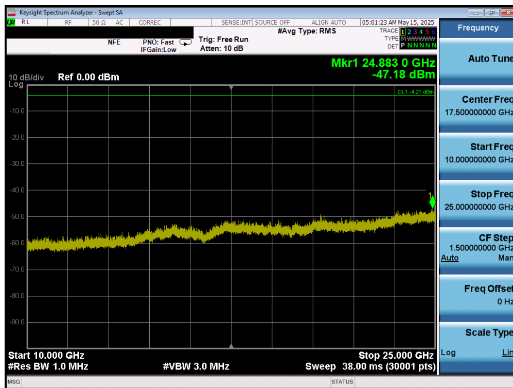
Plot 7-130. Conducted Spurious Plot (Bluetooth (LE), 1Mbps – Ch. 39) – Ant 1
