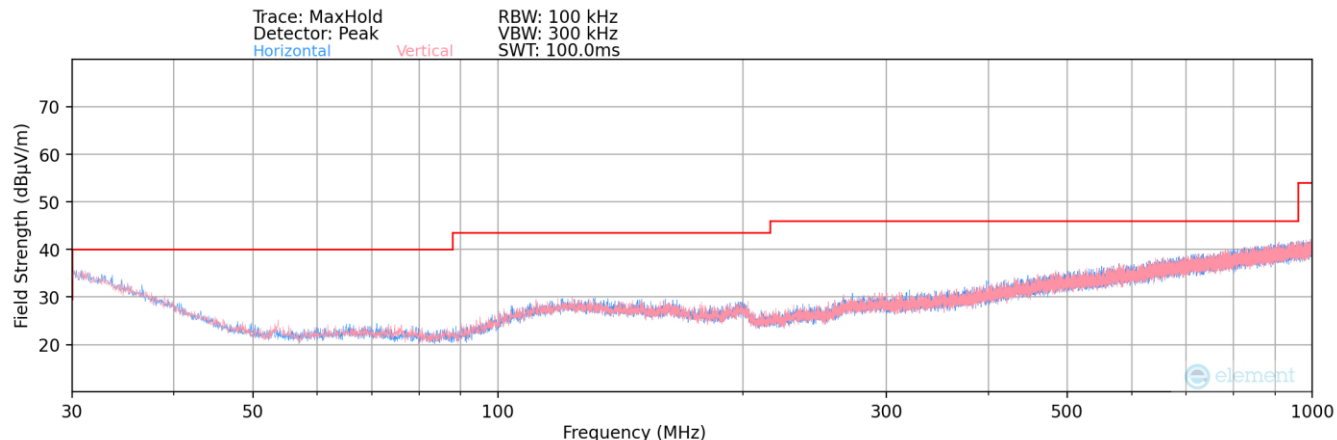
Plot 7-164. Radiated Spurious Plot below 1GHz – Ant 1
