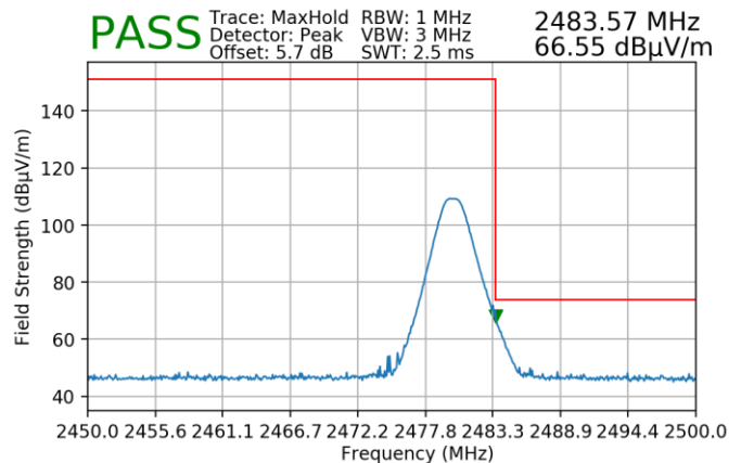
Plot 7-161. Radiated Restricted Upper Band Edge Measurement (Peak) – Ant 2
