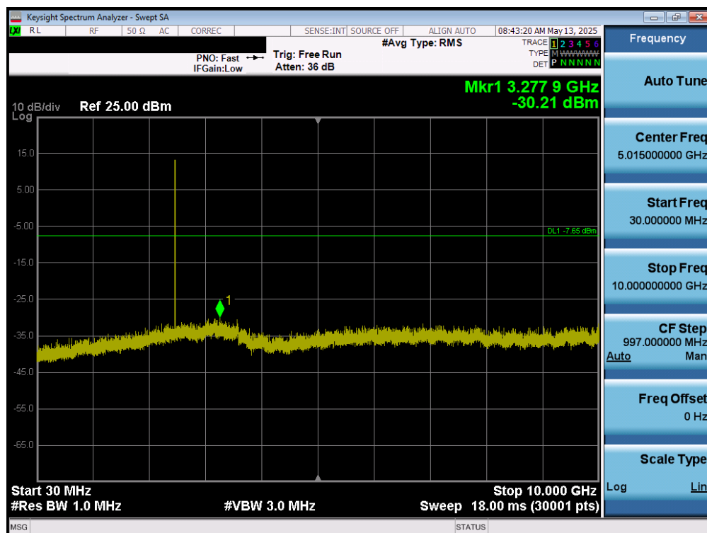
Plot 7-141. Conducted Spurious Plot (Bluetooth (LE), 1Mbps – Ch. 39) – Dual Ant 1
