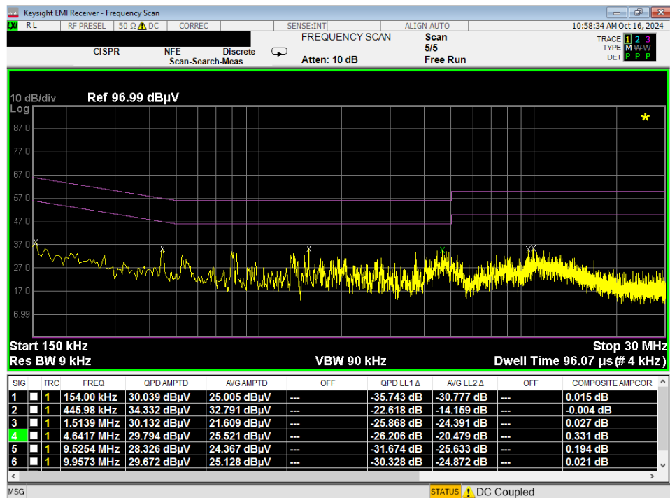
Plot 7-169. Line Conducted Plot with Bluetooth LE (L1) - WCP
