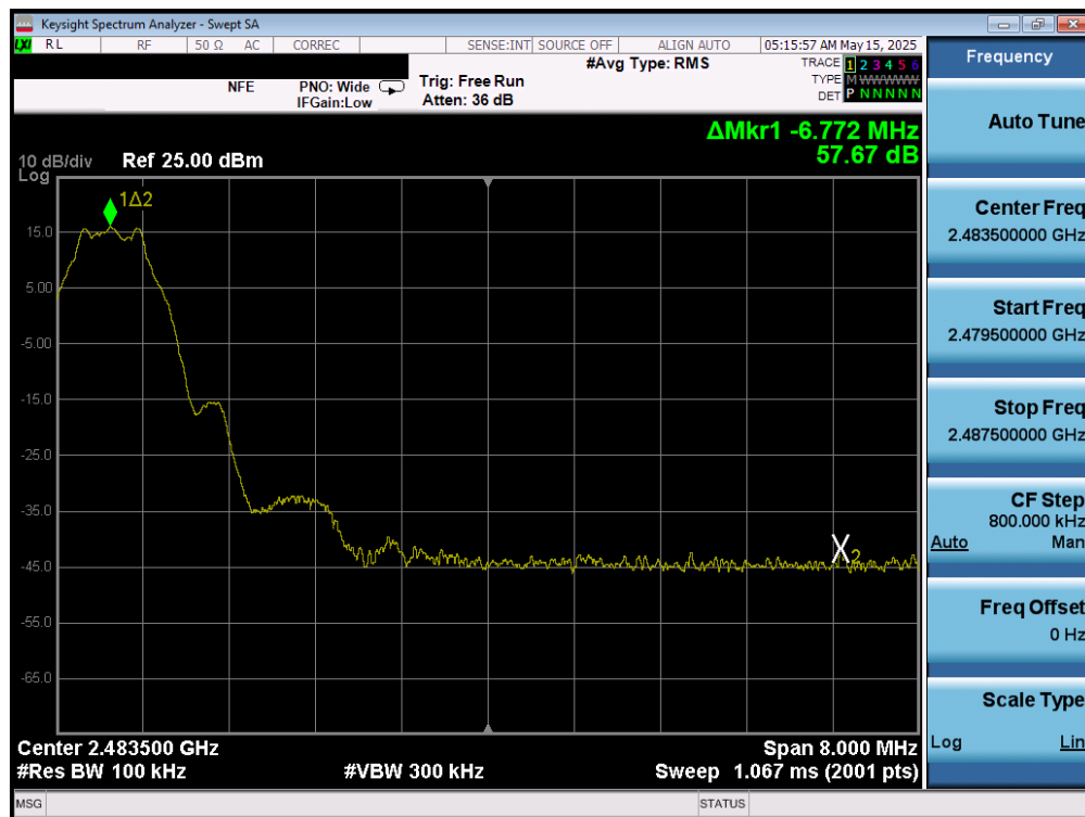
Plot 7-114. Band Edge Plot (Bluetooth (LE), 1Mbps – Ch. 39) – Ant 2
