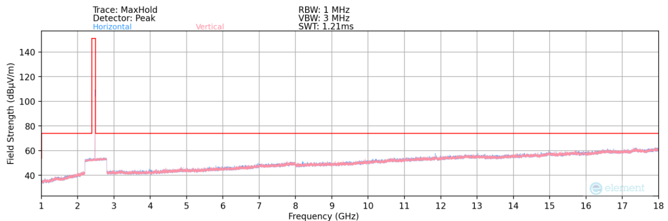
Plot 7-151. Radiated Spurious Plot above 1GHz (Bluetooth (LE) – Ch. 39) – Ant 1
