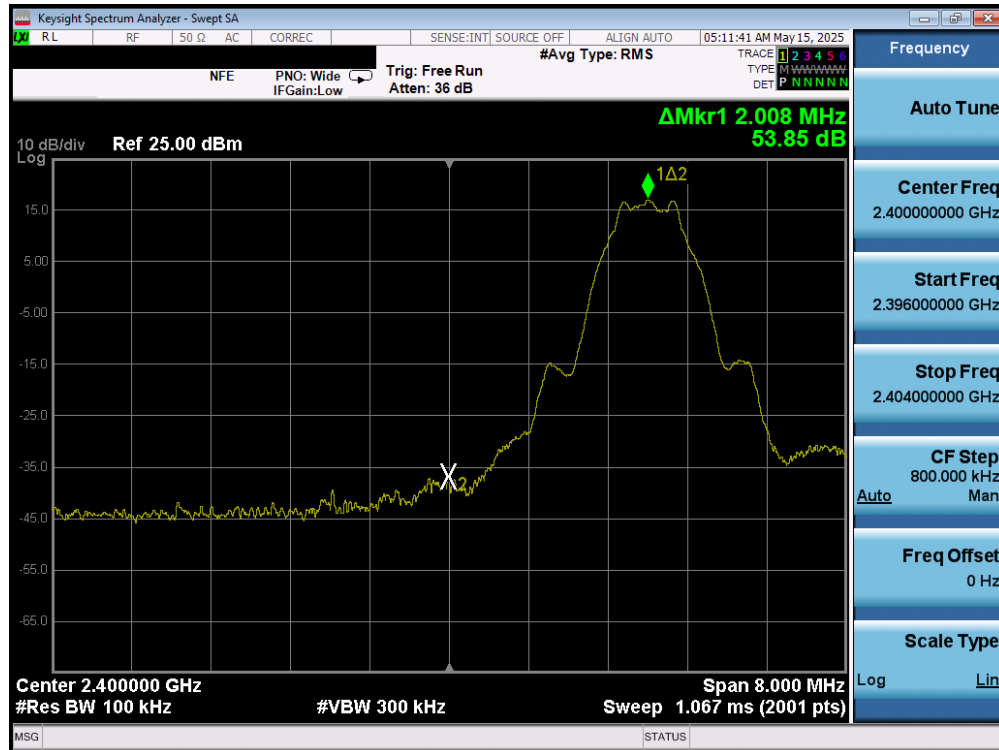
Plot 7-113. Band Edge Plot (Bluetooth (LE), 1Mbps – Ch. 37) – Ant 2
