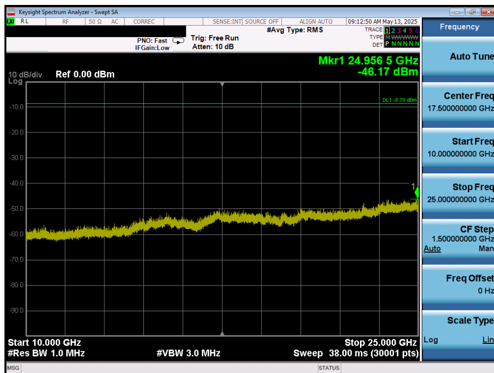
Plot 7-148. Conducted Spurious Plot (Bluetooth (LE), 1Mbps – Ch. 39) – Dual Ant 2
