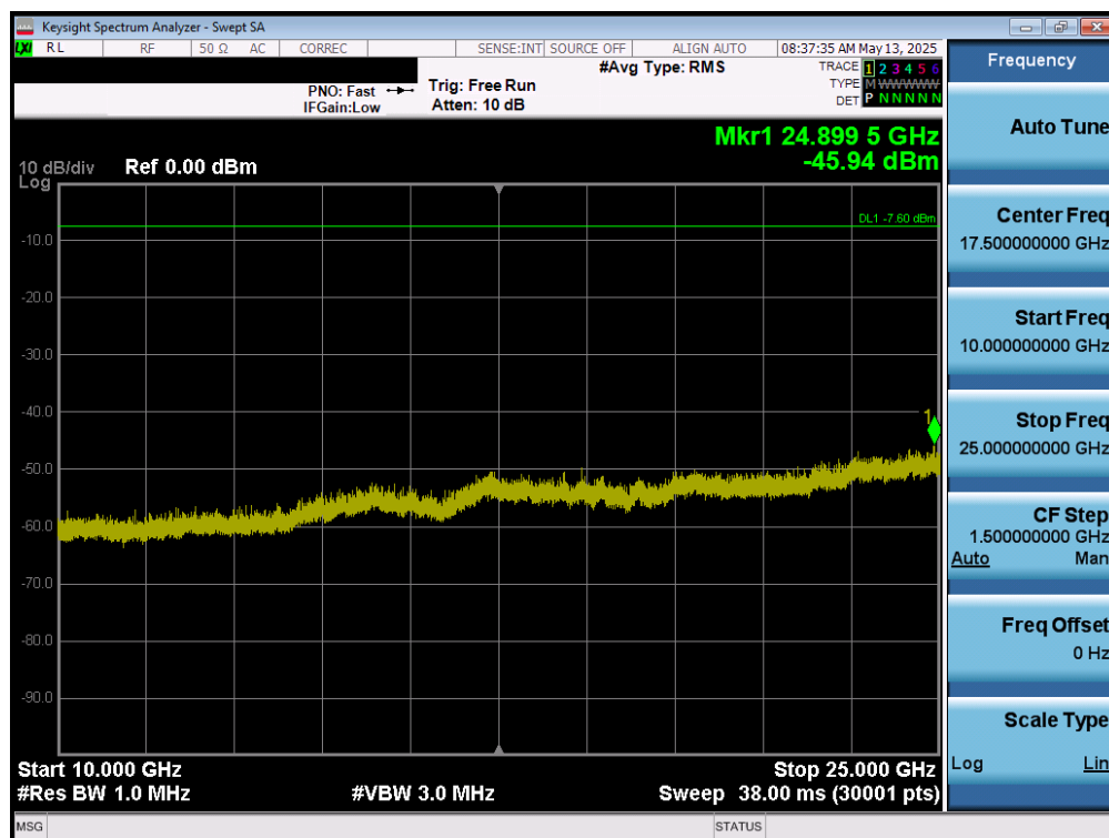
Plot 7-140. Conducted Spurious Plot (Bluetooth (LE), 1Mbps – Ch. 17) – Dual Ant 1
