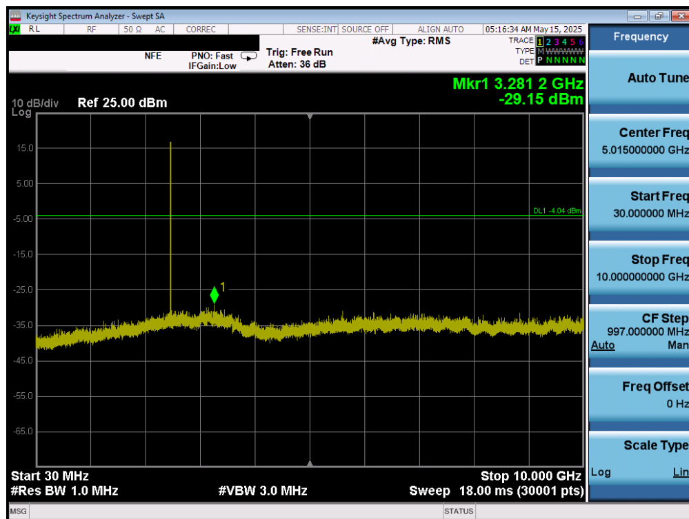
Plot 7-135. Conducted Spurious Plot (Bluetooth (LE), 1Mbps – Ch. 39) – Ant 2
