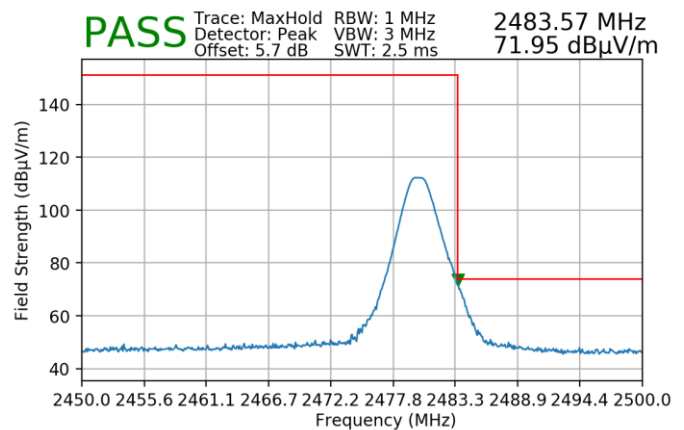
Plot 7-159. Radiated Restricted Upper Band Edge Measurement (Peak) – Ant 1
