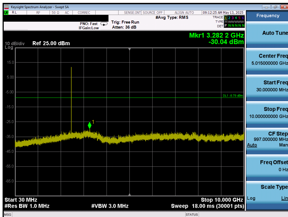
Plot 7-147. Conducted Spurious Plot (Bluetooth (LE), 1Mbps – Ch. 39) – Dual Ant 2
