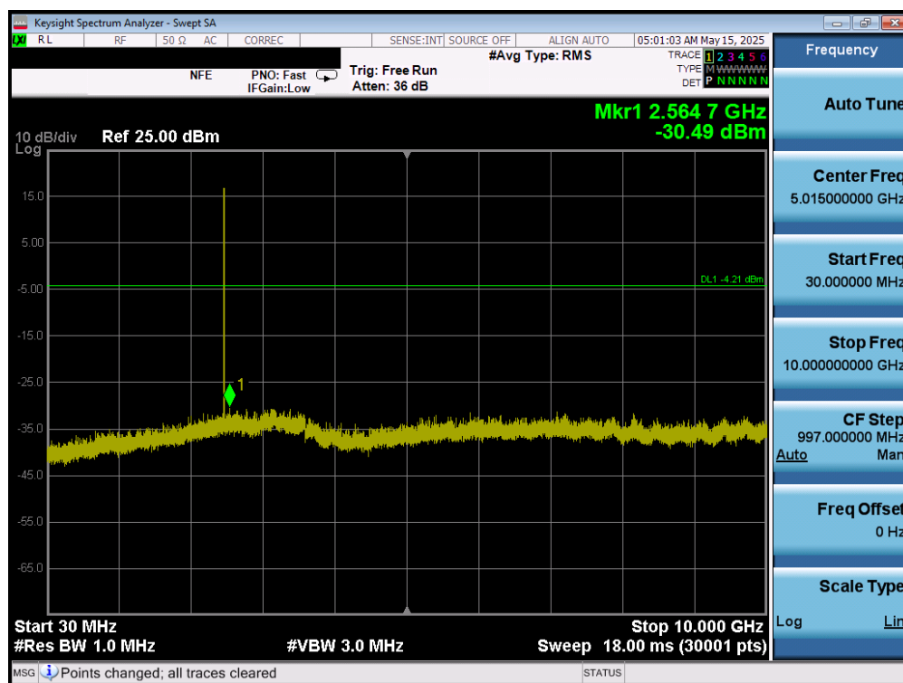
Plot 7-129. Conducted Spurious Plot (Bluetooth (LE), 1Mbps – Ch. 39) – Ant 1
