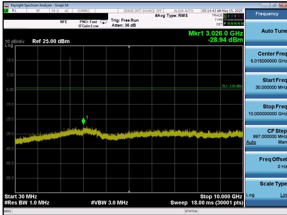
Plot 7-133. Conducted Spurious Plot (Bluetooth (LE), 1Mbps – Ch. 17) – Ant 2
