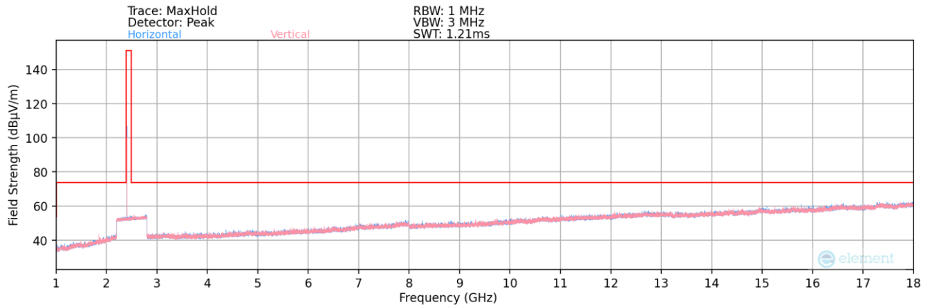
Plot 7-155. Radiated Spurious Plot above 1GHz (Bluetooth (LE) – Ch. 37) – Dual Ant
