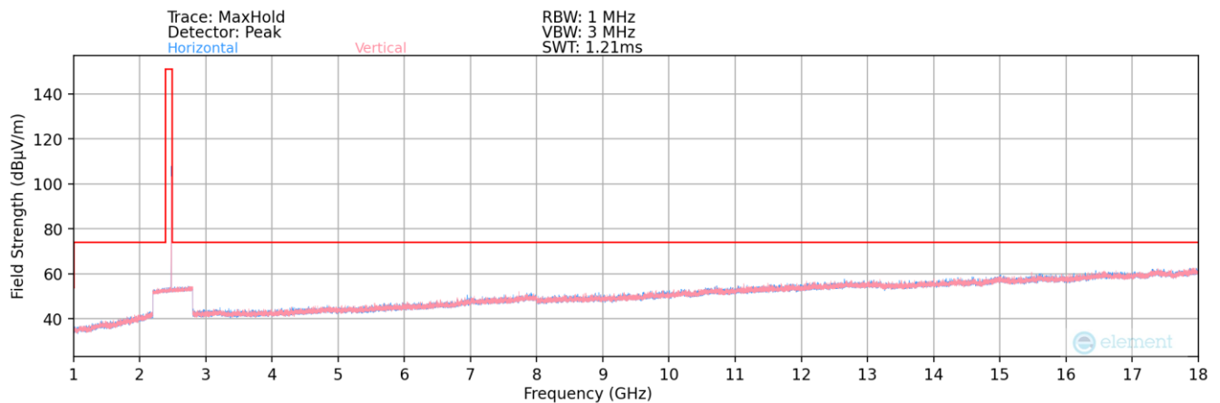
Plot 7-157. Radiated Spurious Plot above 1GHz (Bluetooth (LE) – Ch. 39) – Dual Ant
