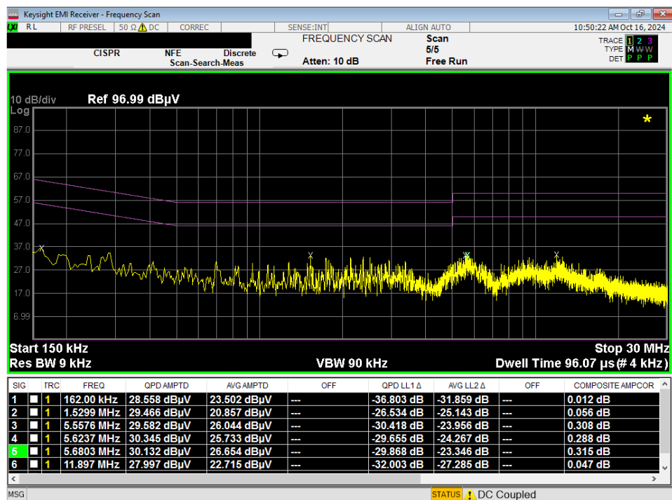
Plot 7-168. Line Conducted Plot with Bluetooth LE (N)
