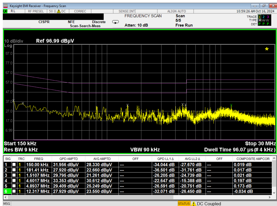
Plot 7-170. Line Conducted Plot with Bluetooth LE (N) - WCP
