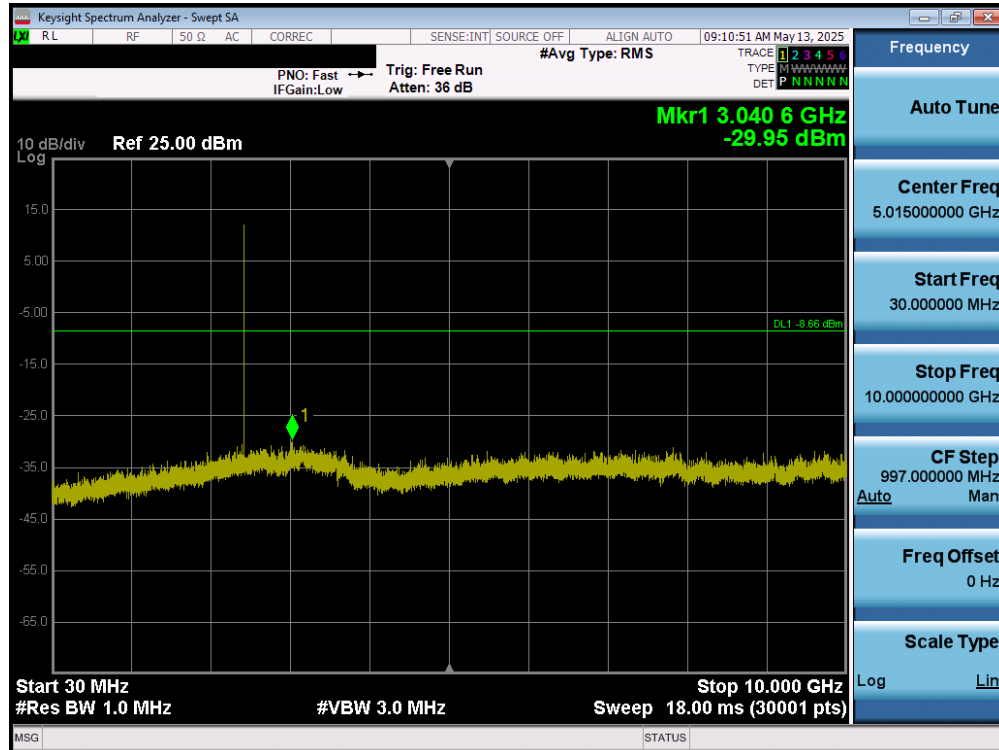
Plot 7-145. Conducted Spurious Plot (Bluetooth (LE), 1Mbps – Ch. 17) – Dual Ant 2
