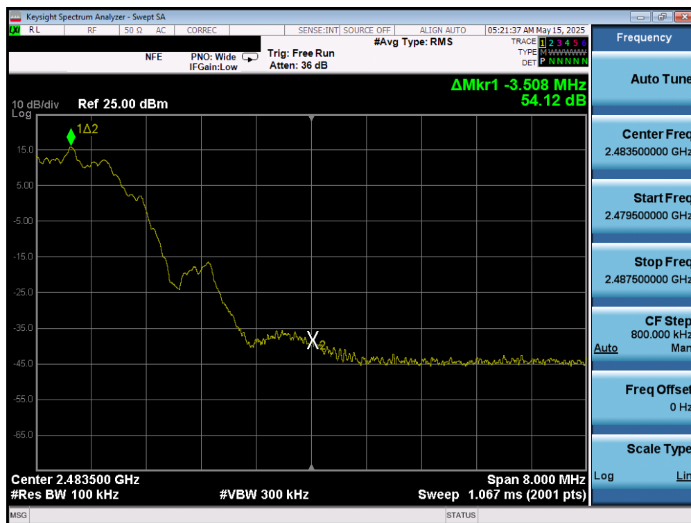
Plot 7-116. Band Edge Plot (Bluetooth (LE), 2Mbps – Ch. 39) – Ant 2
