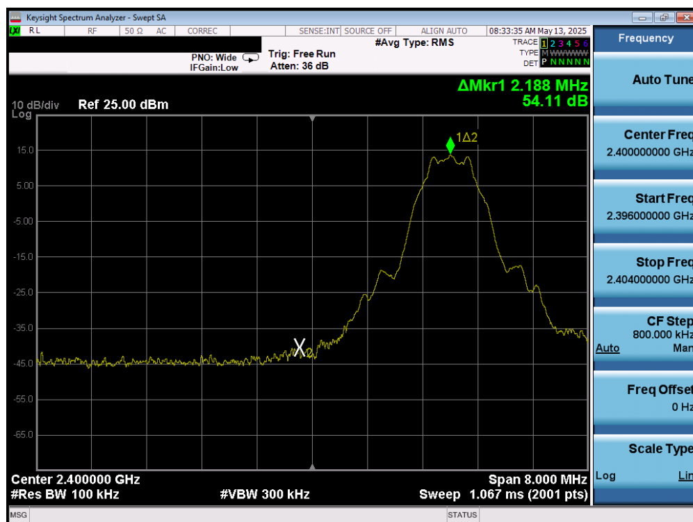
Plot 7-117. Band Edge Plot (Bluetooth (LE), 1Mbps – Ch. 37) – Dual Ant 1
