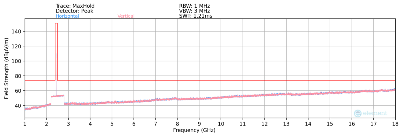
Plot 7-150. Radiated Spurious Plot above 1GHz (Bluetooth (LE) – Ch. 17) – Ant 1
