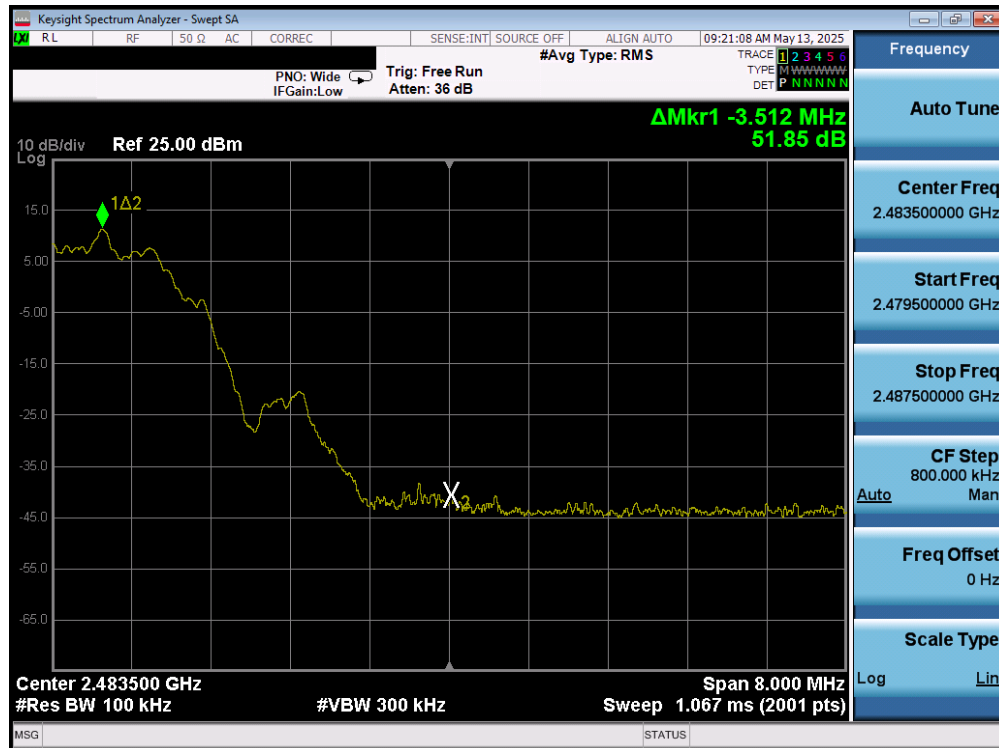
Plot 7-124. Band Edge Plot (Bluetooth (LE), 2Mbps – Ch. 39) – Dual Ant 2
