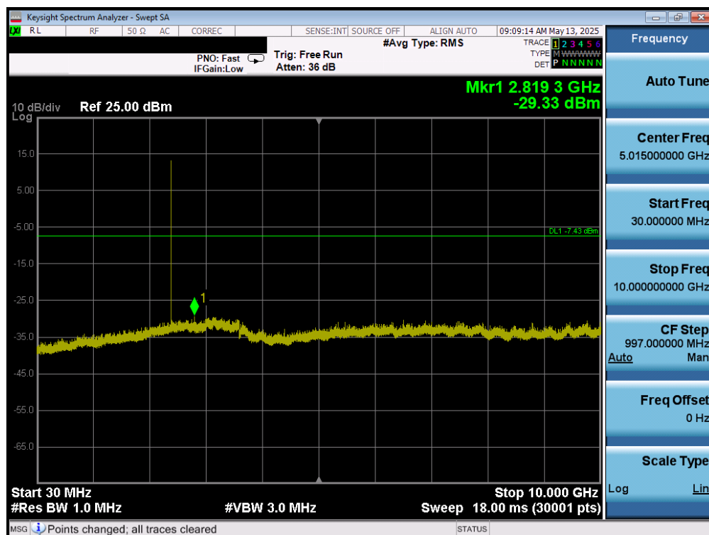
Plot 7-143. Conducted Spurious Plot (Bluetooth (LE), 1Mbps – Ch. 37) – Dual Ant 2
