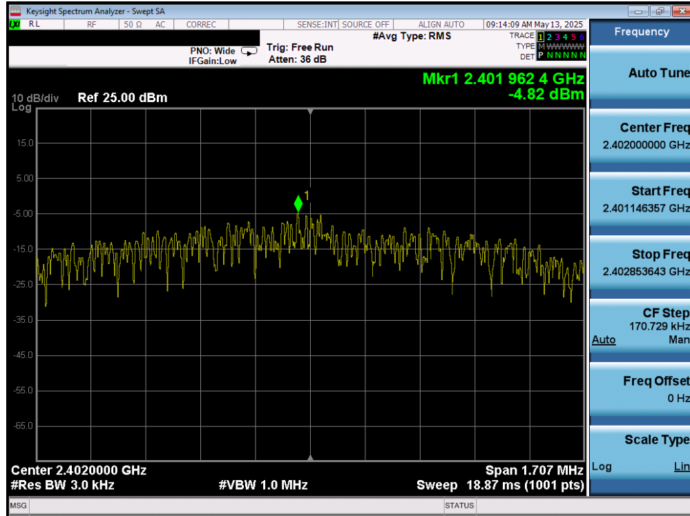
Plot 7-106. Power Spectral Density Plot (Bluetooth (LE), 2Mbps – Ch. 37) – Dual Ant 2
