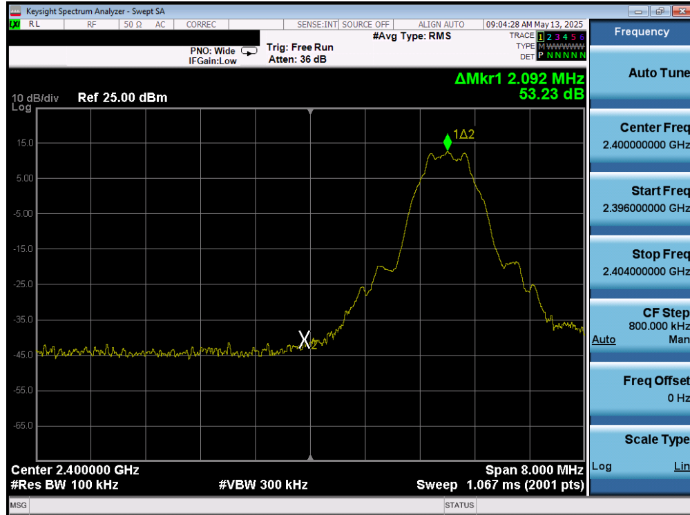
Plot 7-121. Band Edge Plot (Bluetooth (LE), 1Mbps - Ch. 37) - Dual Ant 2
