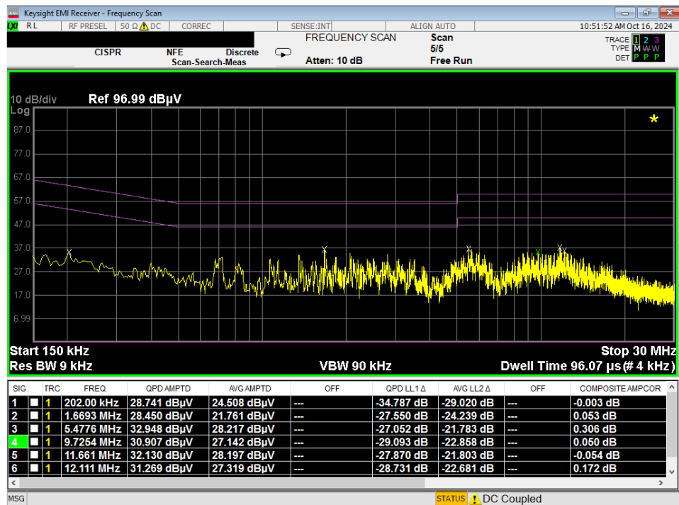
Plot 7-167. Line Conducted Plot with Bluetooth LE (L1)
