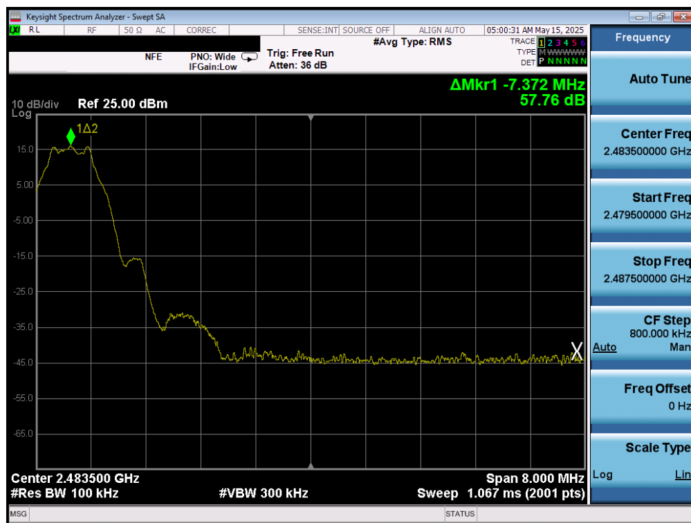
Plot 7-110. Band Edge Plot (Bluetooth (LE), 1Mbps – Ch. 39) – Ant 1
