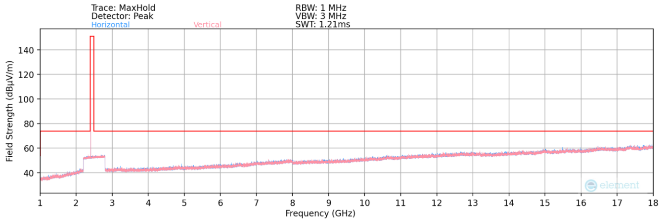
Plot 7-152. Radiated Spurious Plot above 1GHz (Bluetooth (LE) – Ch. 37) – Ant 2
