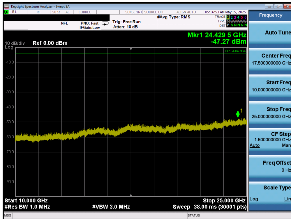
Plot 7-136. Conducted Spurious Plot (Bluetooth (LE), 1Mbps – Ch. 39) – Ant 2
