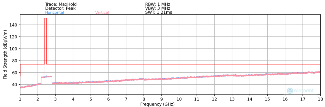
Plot 7-149. Radiated Spurious Plot above 1GHz (Bluetooth (LE) – Ch. 37) – Ant 1
