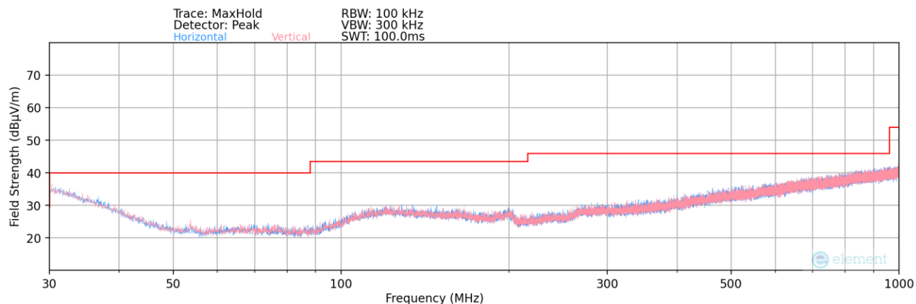
Plot 7-165. Radiated Spurious Plot below 1GHz – Ant 2
