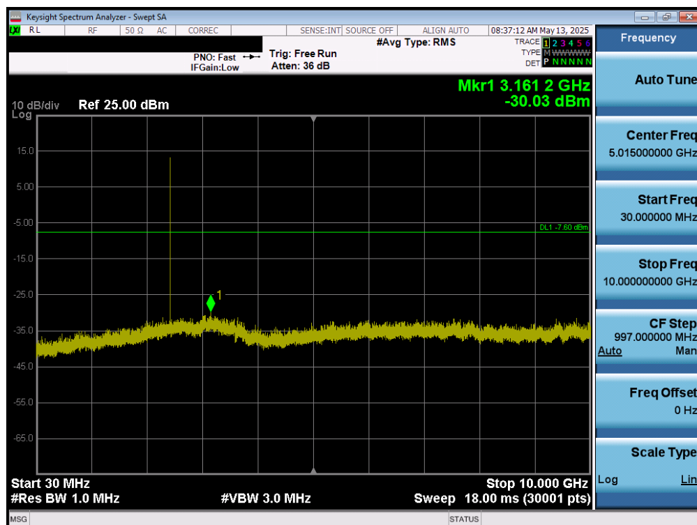
Plot 7-139. Conducted Spurious Plot (Bluetooth (LE), 1Mbps – Ch. 17) – Dual Ant 1
