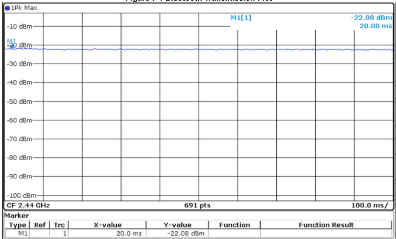
Figure 7-1 Bluetooth Transmission Plot
