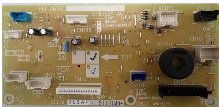
Top and bottom view of PCB A UNIT (Main control Board)
