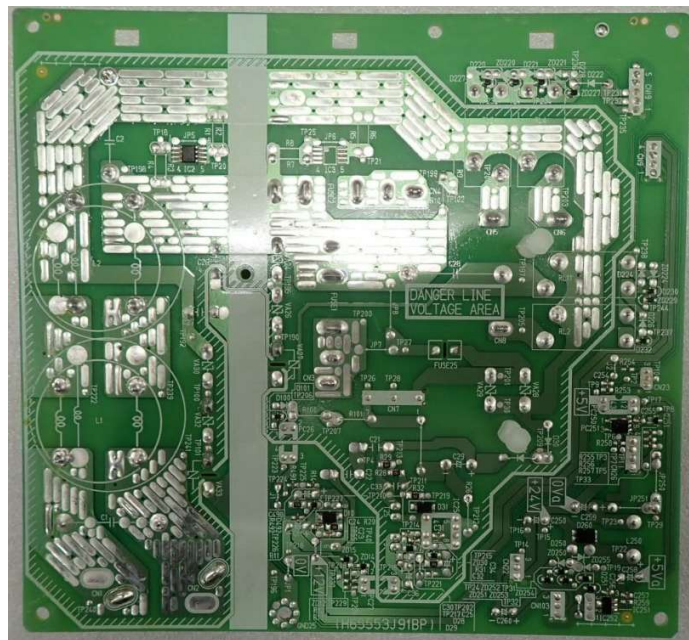
Top and bottom view of PCB D UNIT (Power supply, Power relay, Line noise filter Board)
