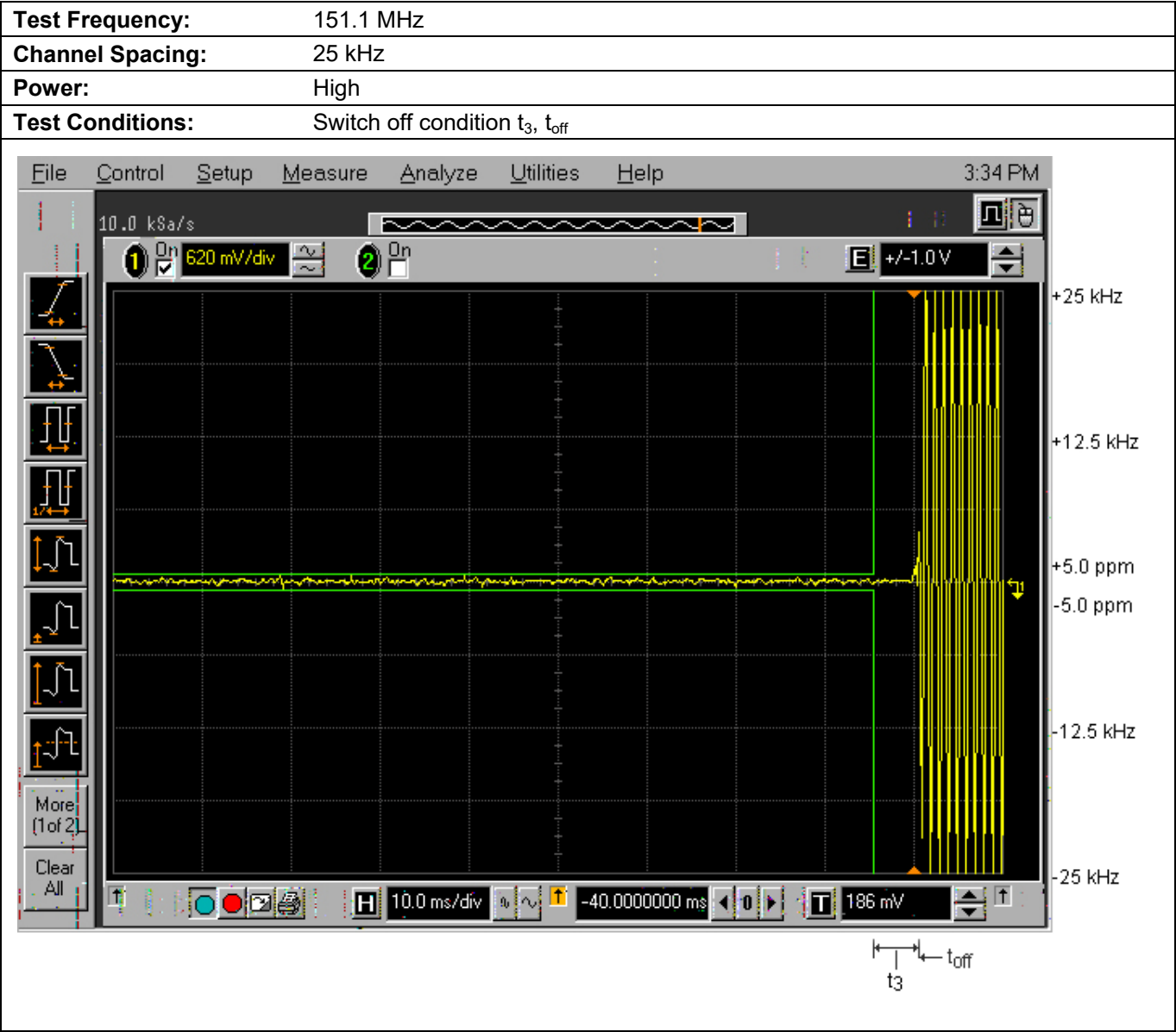
Plot 5.12.3.6. Transient Frequency Behavior for 25 kHz Channel Spacing
