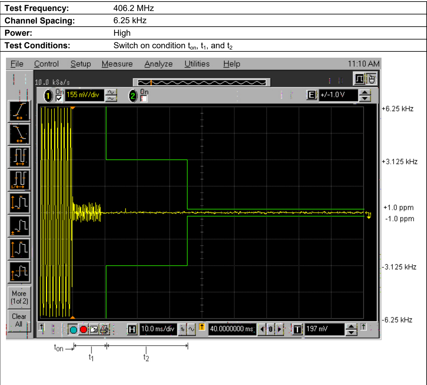
Plot 5.12.3.1. Transient Frequency Behavior for 6.25 kHz Channel Spacing
