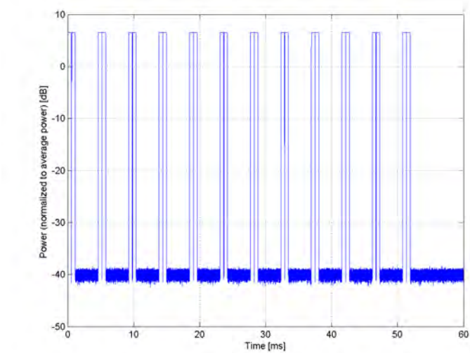
Time Domain
