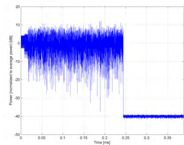
Time Domain
