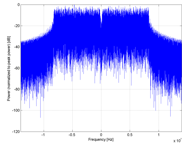
Frequency Domain
