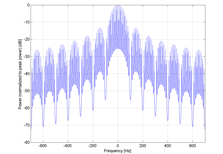
Frequency Domain
