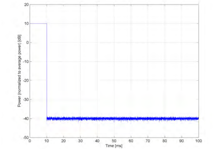
Time Domain
