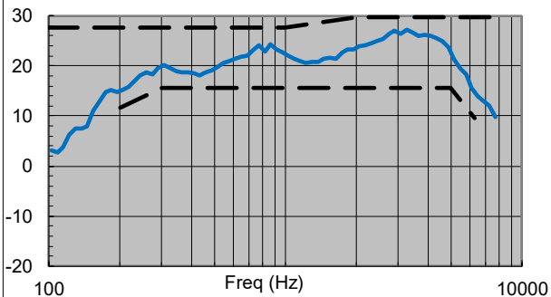
Receive Response DF 8N
