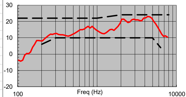
Receive Response FF 2N
