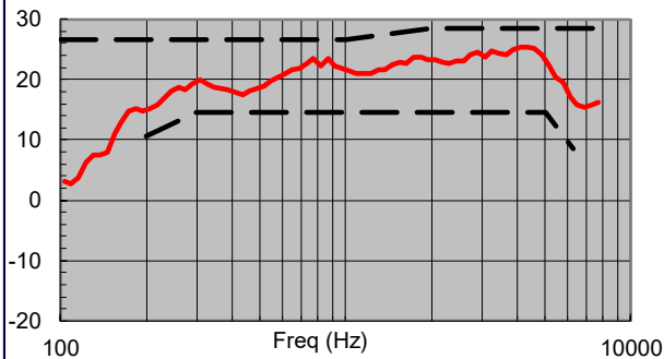
Receive Response FF 8N
