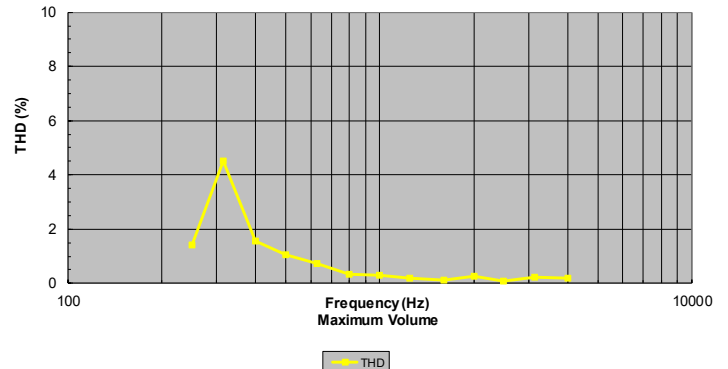
TIA-5050 Measurement at 2N Receive THD (comprised of 2nd & 3rd Harmonics)
