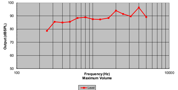
TIA-5050 Measurement at 2N Receive Output vs Frequency
