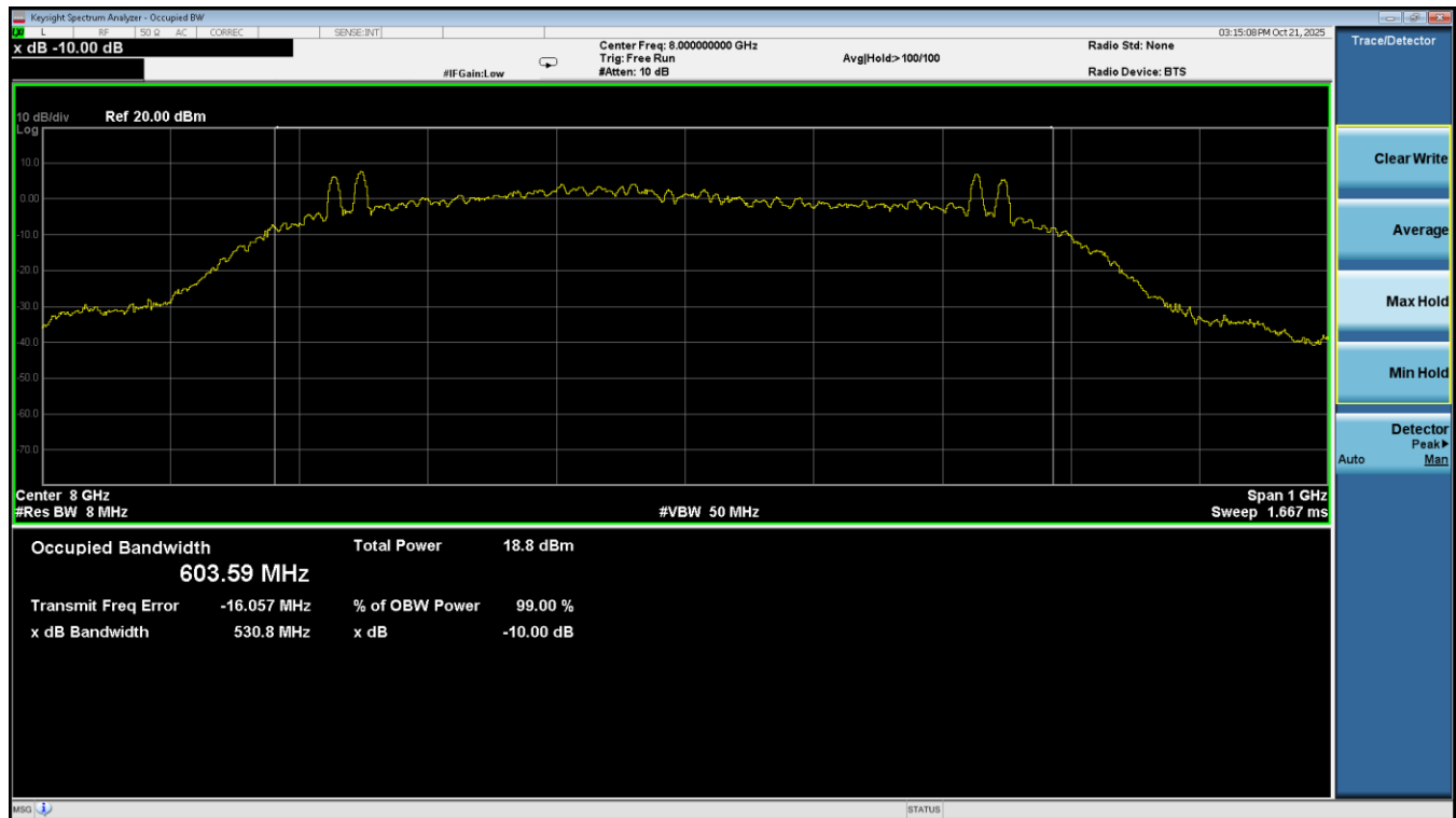
Plot 7-2. ISED 10dBc Occupied Bandwidth & 99% OBW (Ch. 9, Config 1/Payload125B)
