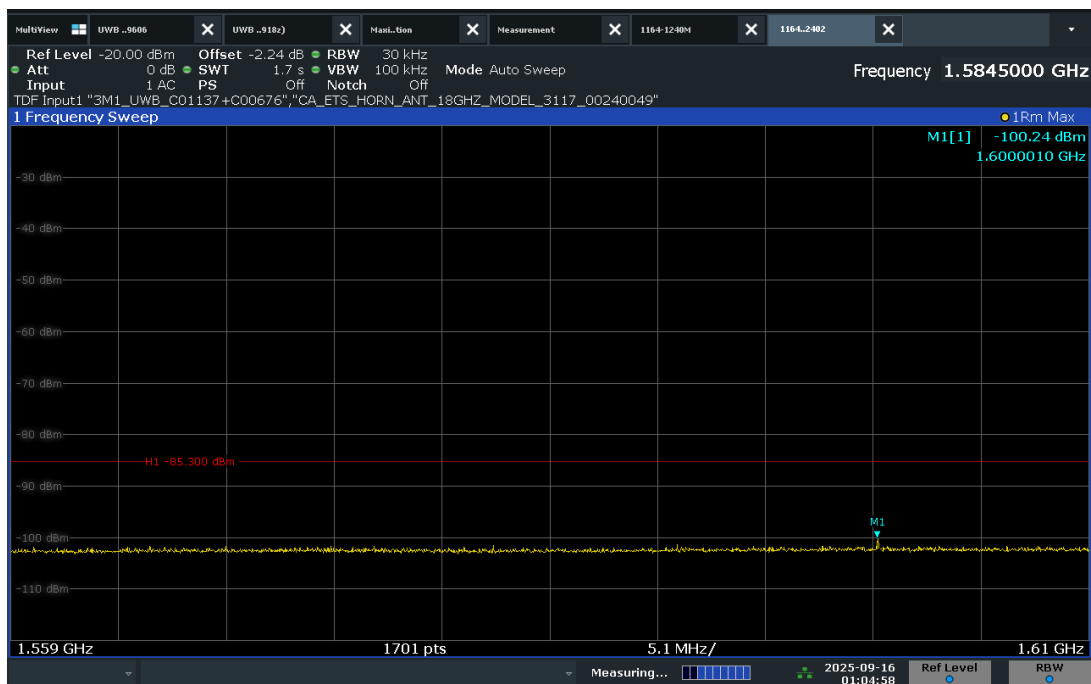
Plot 7-14. Radiated Spurious Emission 1559-1610MHz (Ch. 9, Config 1, Payload 125B Ant. Pol. V)
