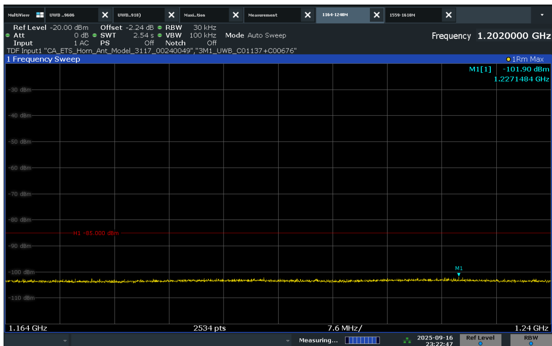
Plot 7-12. Radiated Spurious Emission 1164-1240MHz (Ch. 9, Config 1, Payload 125B Ant. Pol. V)
