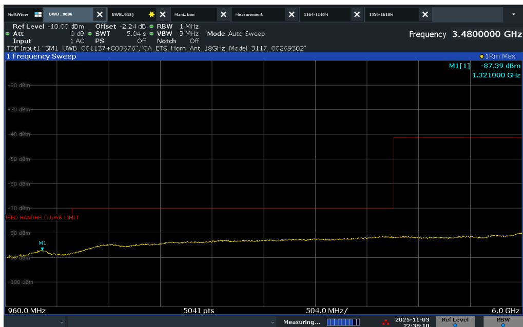
Plot 7-10. ISD Radiated Spurious Emission 960-6000MHz (Ch.9, Config 1, Payload 125B Ant. Pol. V)
