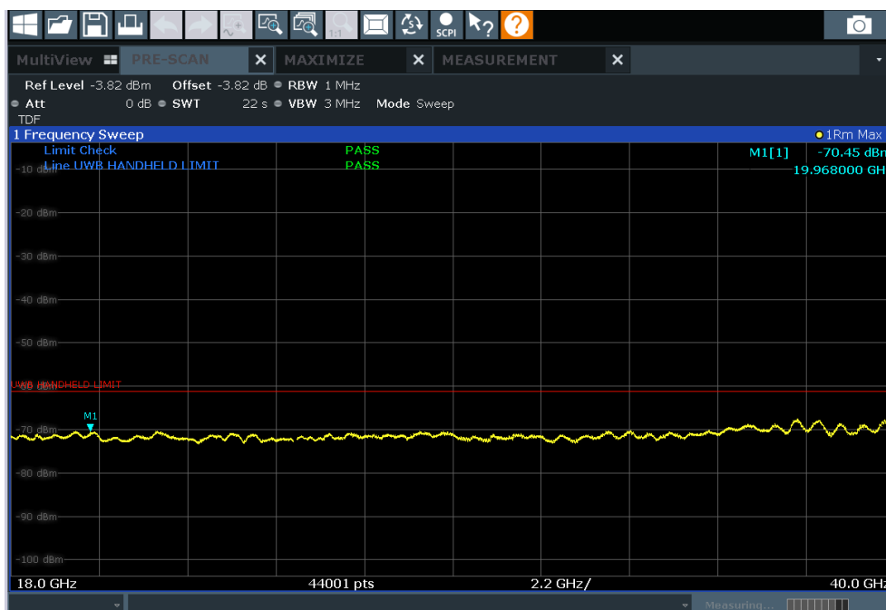
Plot 7-17. Radiated Spurious Emission 18-40GHz (Ch. 9, Config 1, Payload 125B Ant. Pol. H)
