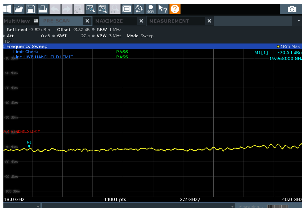
Plot 7-18. Radiated Spurious Emission 18-40GHz (Ch. 9, Config 1, Payload 125B Ant. Pol. V)
