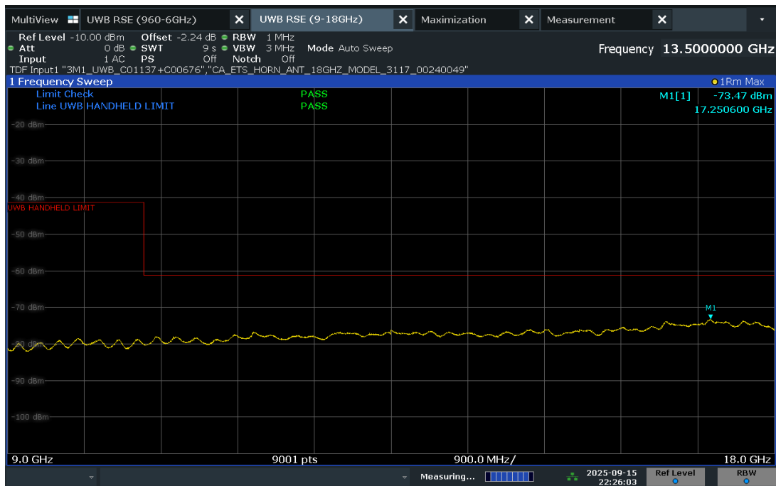
Plot 7-16. Radiated Spurious Emission 9-18GHz (Ch. 9, Config 1, Payload 125B Ant. Pol. V)
