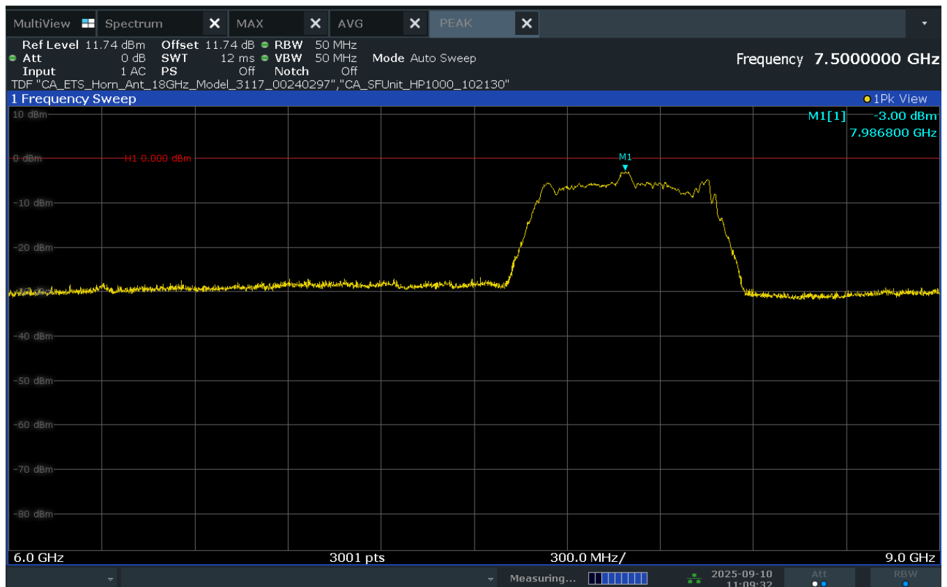
Plot 7-3. Peak Radiated Power (Ch. 9, Config 1 /Payload 125B)
