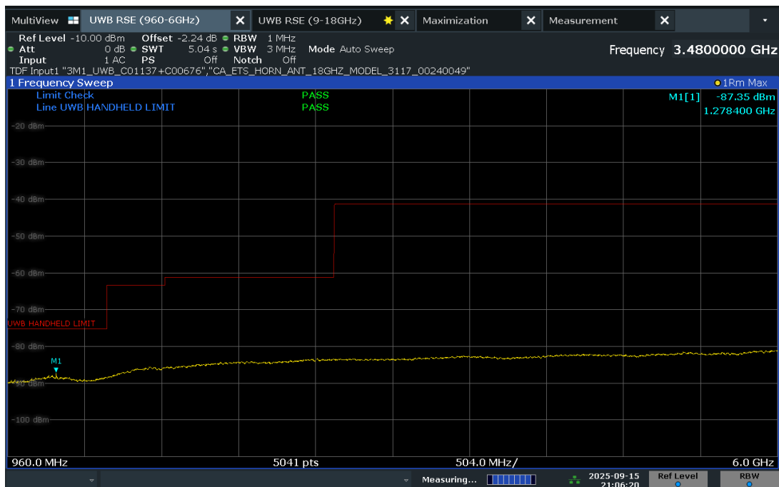
Plot 7-8. FCC Radiated Spurious Emission 960-6000MHz (Ch.9, Config 1, Payload 125B Ant. Pol. V)
