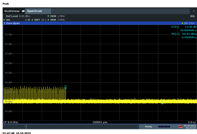
Plot 7-5. Cessation Time – Mode1 (Ch. 9, 8 GHz)
