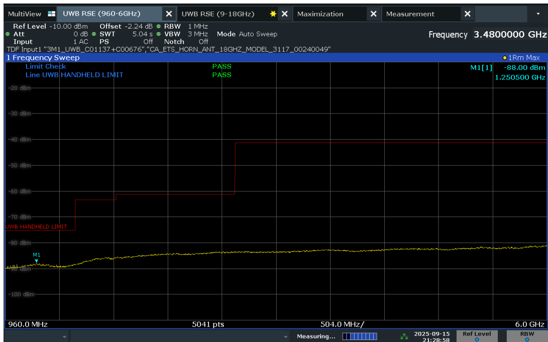
Plot 7-7. FCC Radiated Spurious Emission 960-6000MHz (Ch. 9, Config 1, Payload 125B Ant. Pol. H)
