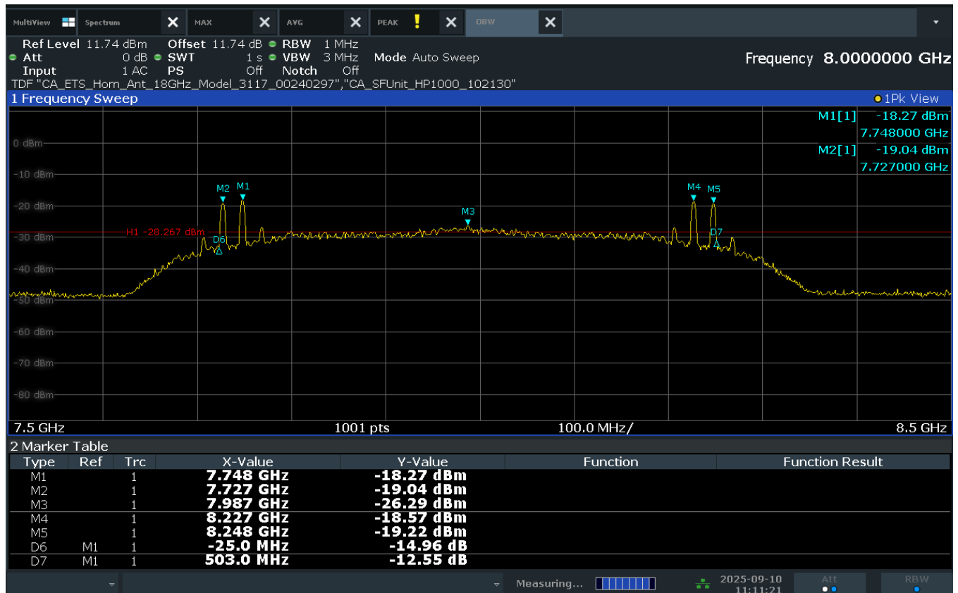
Plot 7-1. 10dBc Bandwidth (Ch. 9, Config 1/Payload 125B)
