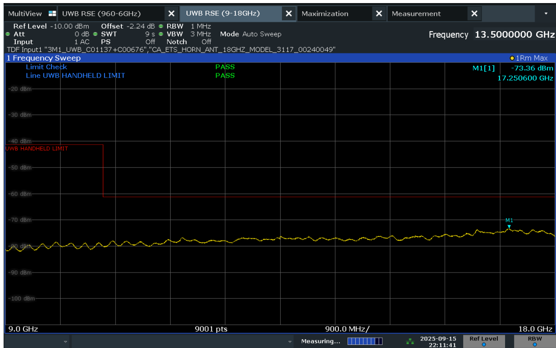
Plot 7-15. Radiated Spurious Emission 9-18GHz (Ch. 9, Config 1, Payload 125B Ant. Pol. H)
