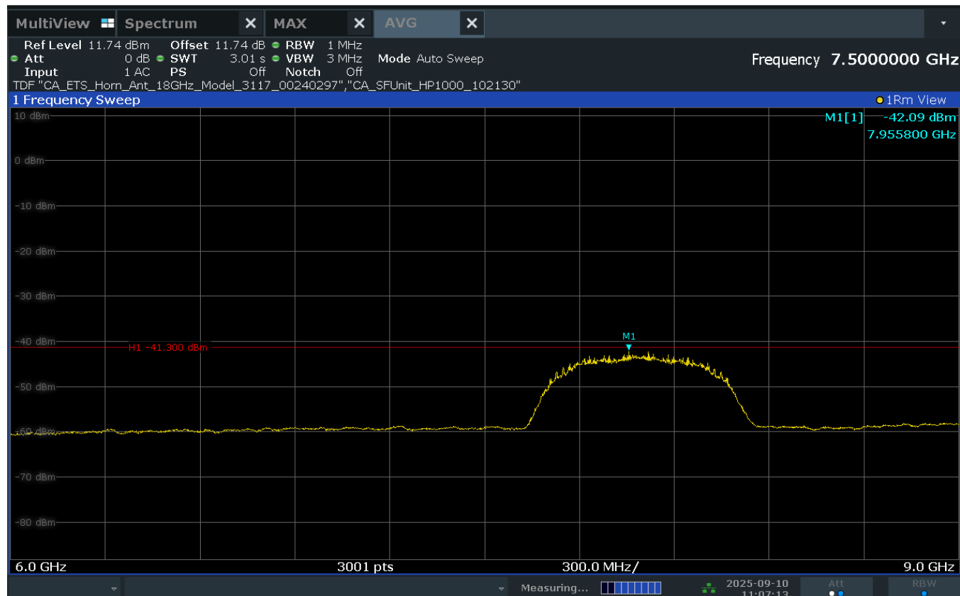
Plot 7-4. Average Radiated Power (Ch. 9, Config 1 /Payload 125B)
