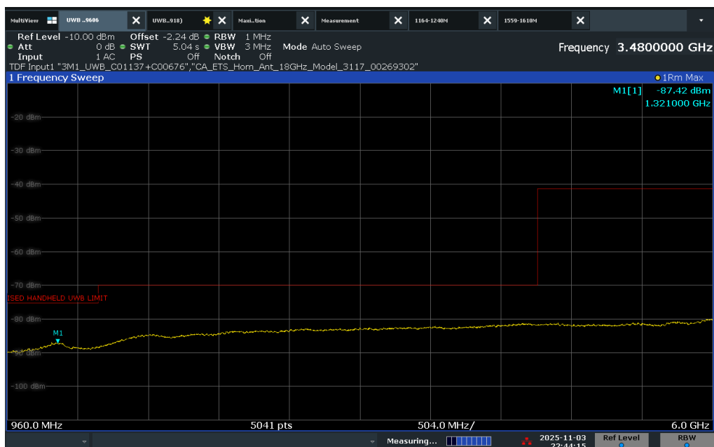
Plot 7-9. ISD Radiated Spurious Emission 960-6000MHz (Ch. 9, Config 1, Payload 125B Ant. Pol. H)
