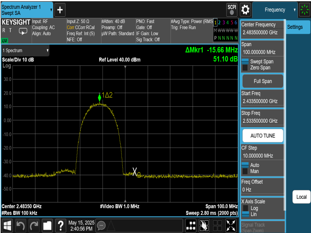
Plot 7-50. Band Edge Plot Antenna WF8 (802.11b – Ch. 13)
