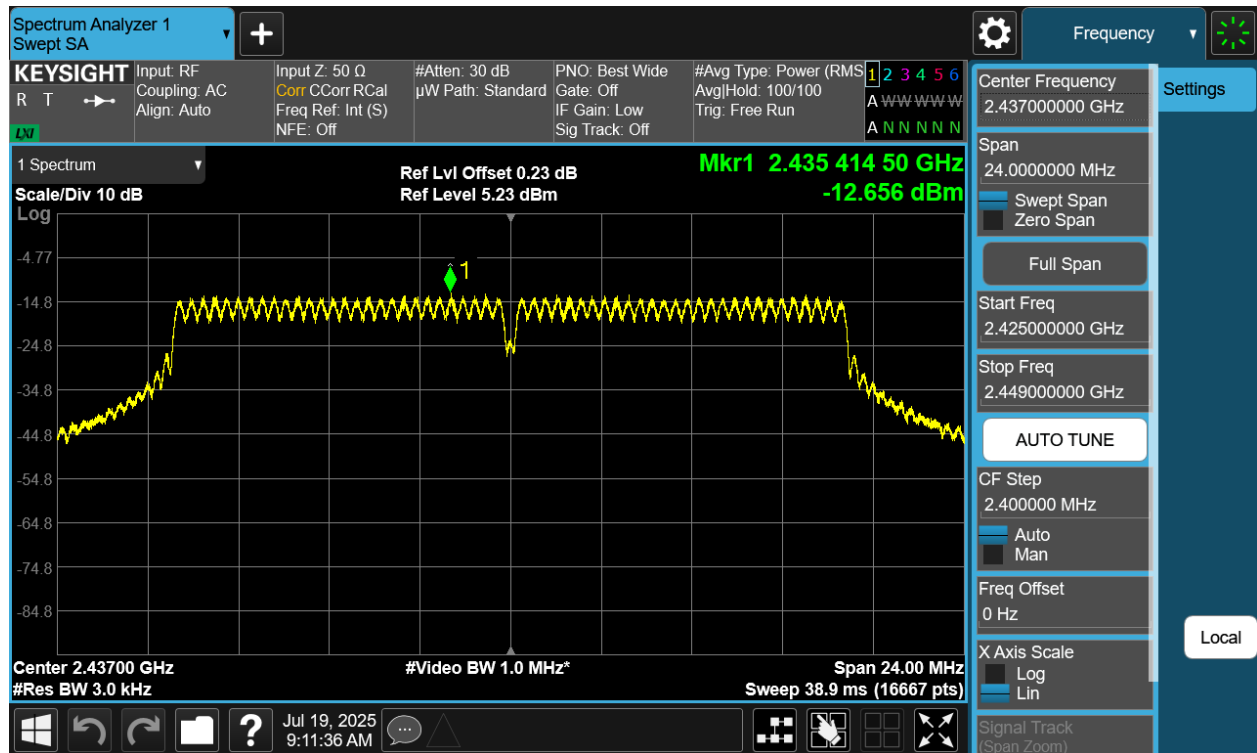
Plot 7-15 PSD Antenna WF8 (20MHz BW 802.11n - Ch.6)
