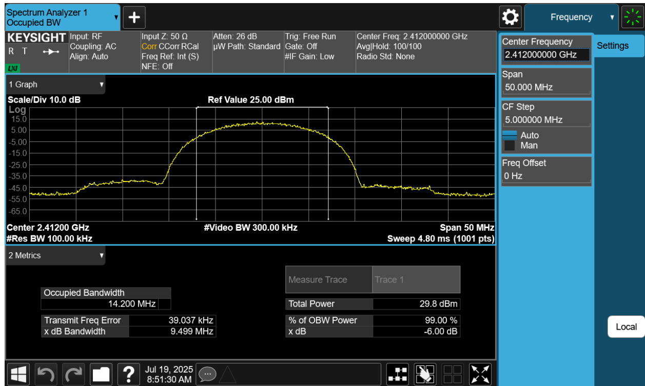
Plot 7-1 6dB BW & 99% OBW Antenna WF8 (20MHz BW 802.11b - Ch.1)
