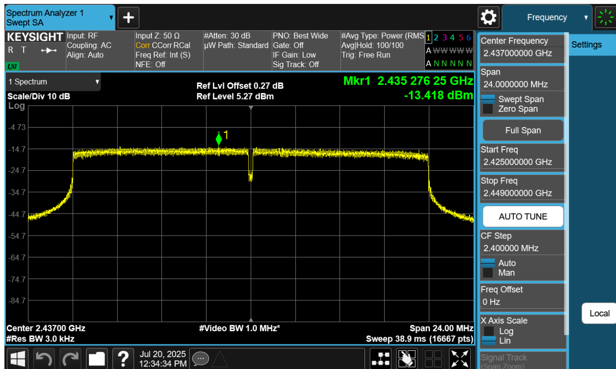
Plot 7-40 PSD CDD Diversity Antenna WF9 (20MHz BW 802.11be(SU) - Ch.6)
