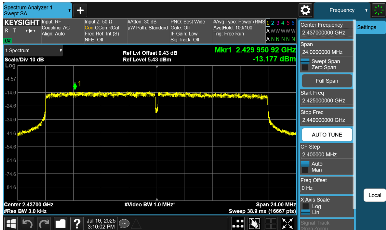
Plot 7-32 PSD CDD Primary Antenna WF7 (20MHz BW 802.11be(SU) - Ch.6)
