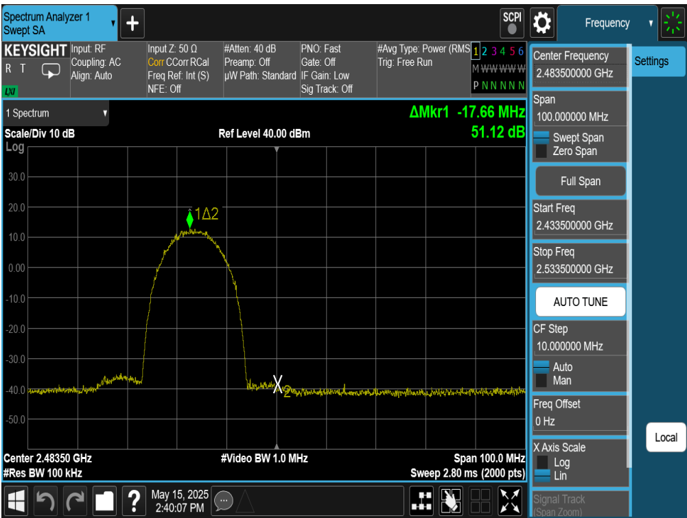
Plot 7-49. Band Edge Plot Antenna WF8 (802.11b – Ch. 12)
