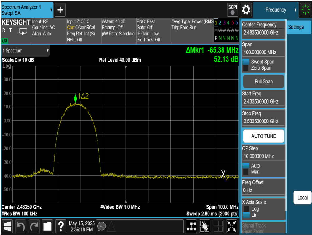
Plot 7-48. Band Edge Plot Antenna WF8 (802.11b – Ch. 11)
