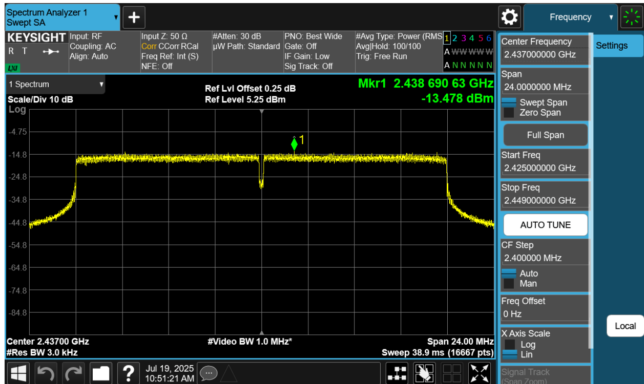
Plot 7-36 PSD CDD Diversity Antenna WF8 (20MHz BW 802.11be(SU) - Ch.6)
