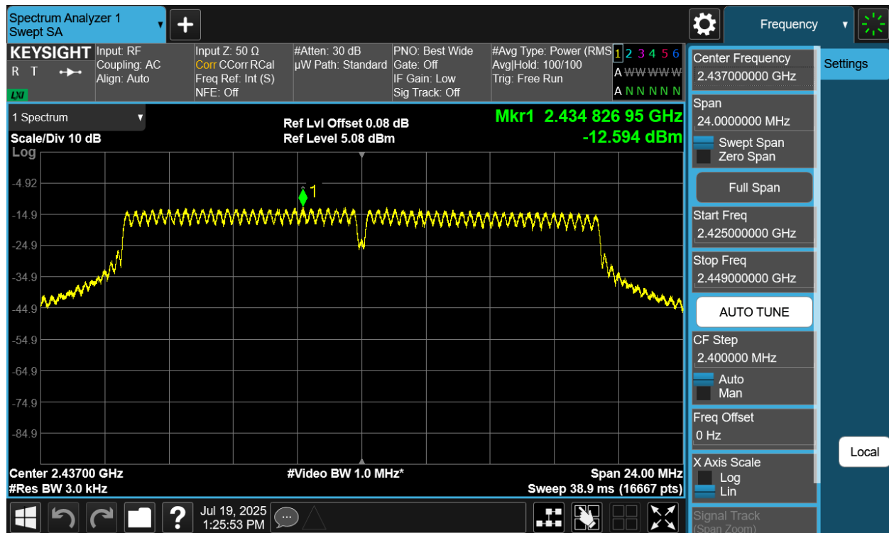
Plot 7-19 PSD Antenna WF7 (20MHz BW 802.11n - Ch.6)
