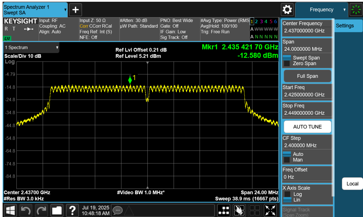
Plot 7-35 PSD CDD Diversity Antenna WF8 (20MHz BW 802.11n - Ch.6)
