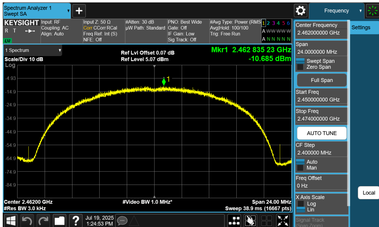
Plot 7-17 PSD Antenna WF7 (20MHz BW 802.11b - Ch.11)
