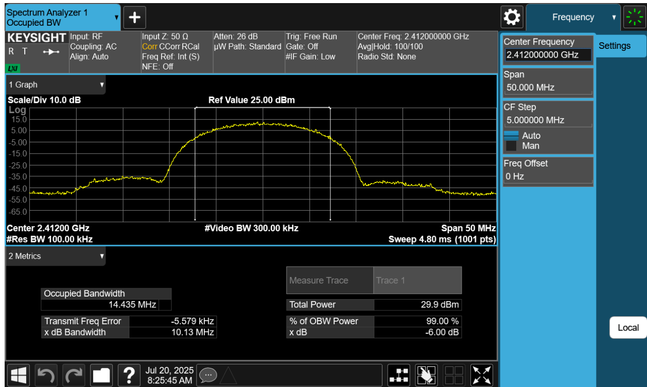
Plot 7-9 6dB BW & 99% OBW Antenna WF9 (20MHz BW 802.11b - Ch.1)
