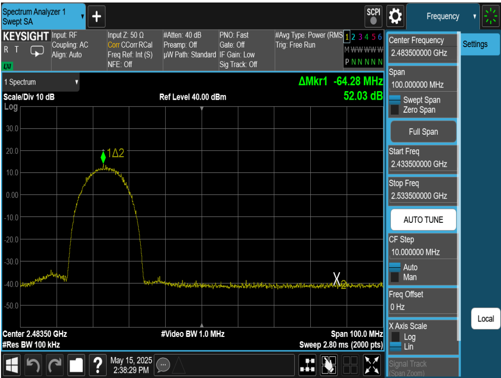
Plot 7-47. Band Edge Plot Antenna WF8 (802.11b – Ch. 10)
