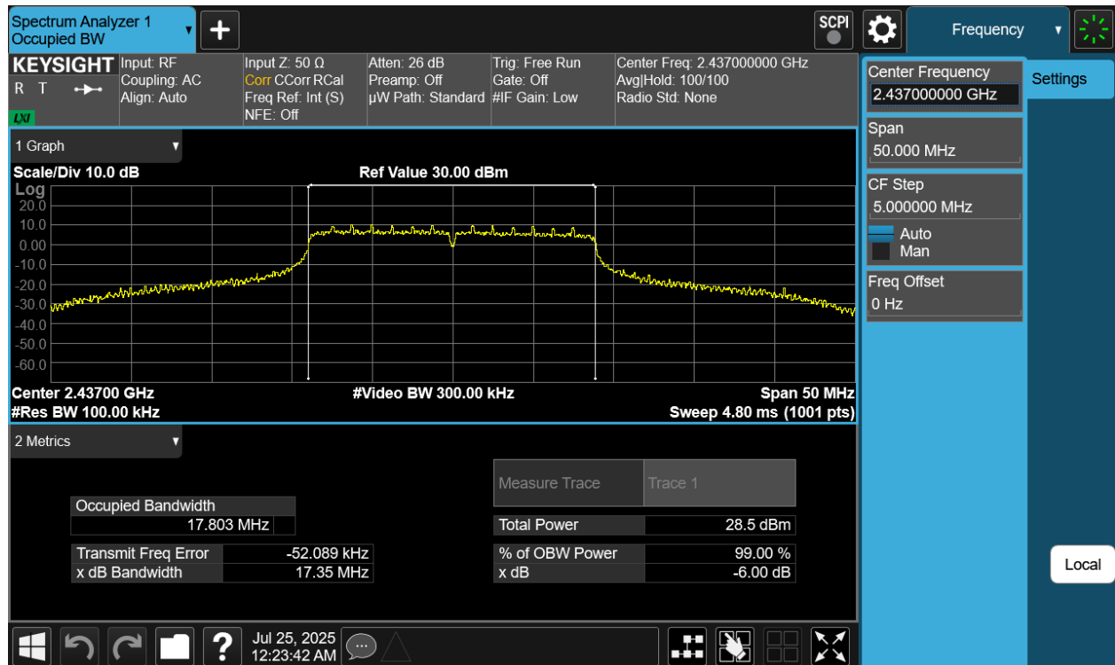
Plot 7-10 6dB BW & 99% OBW Antenna WF9 (20MHz BW 802.11g - Ch.6)
