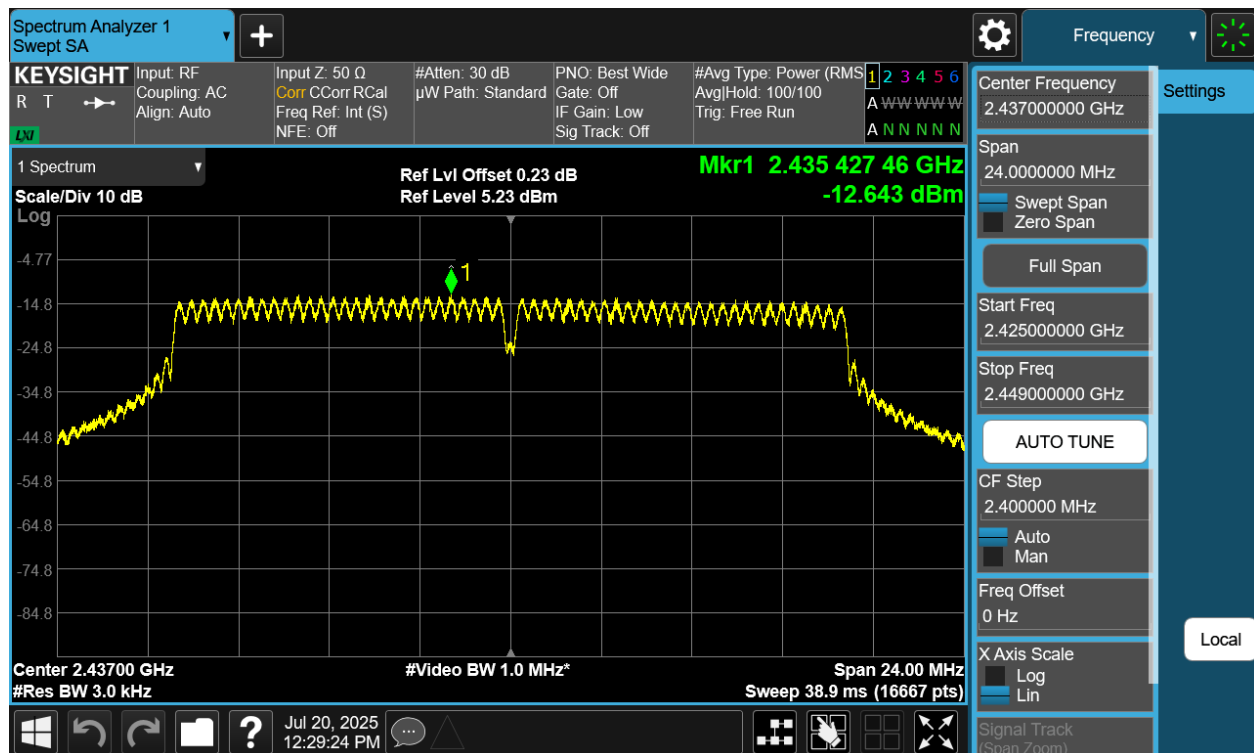
Plot 7-39 PSD CDD Diversity Antenna WF9 (20MHz BW 802.11n - Ch.6)
