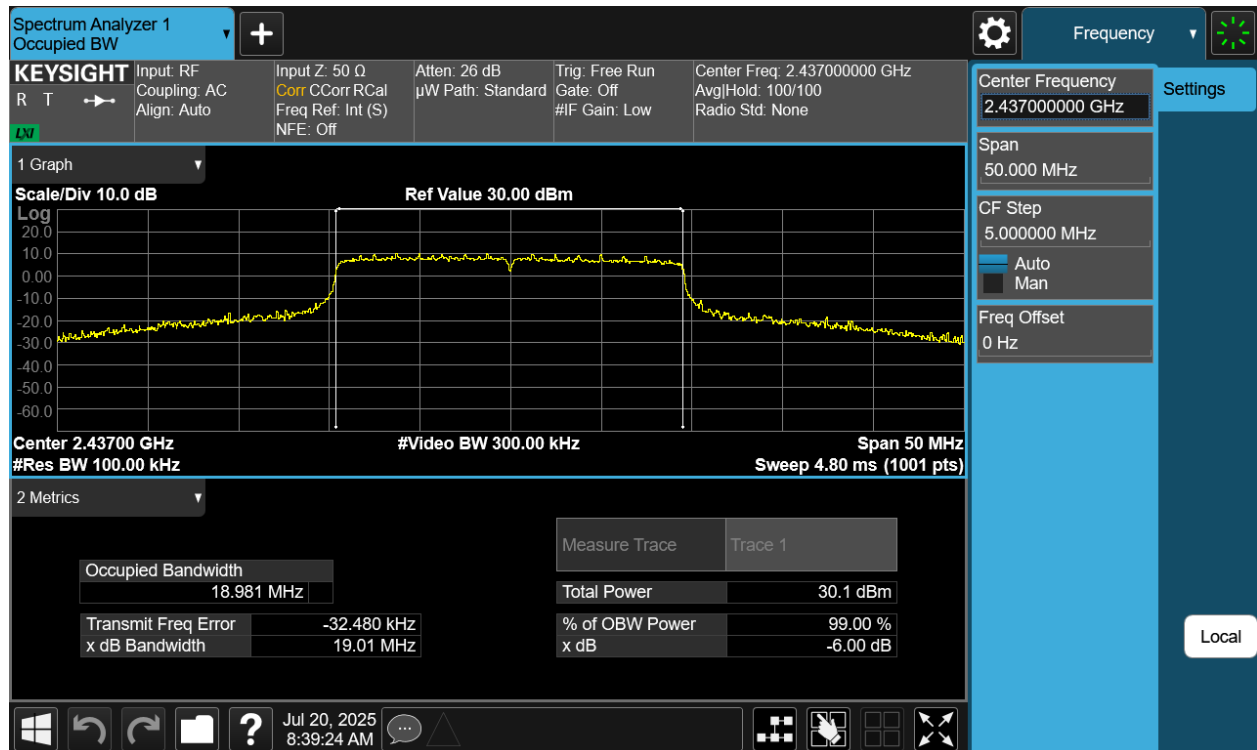
Plot 7-12 6dB BW & 99% OBW Antenna WF9 (20MHz BW 802.11be(SU) - Ch.6)
