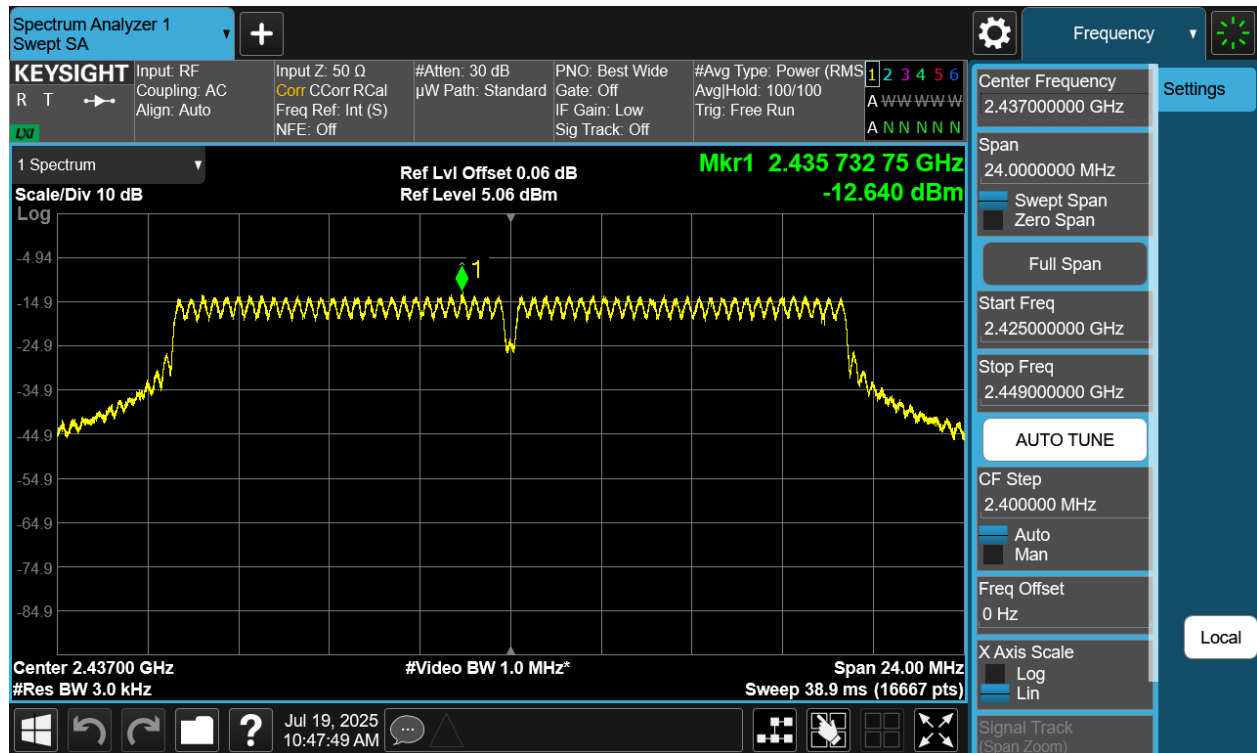
Plot 7-27 PSD CDD Primary Antenna WF8 (20MHz BW 802.11n - Ch.6)
