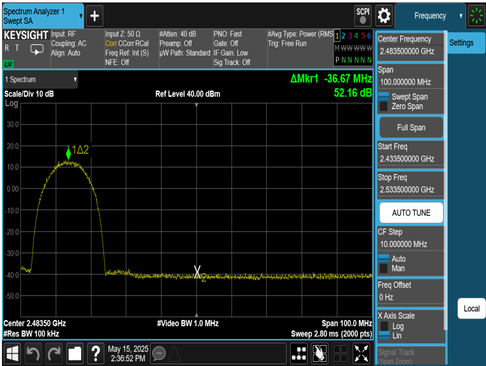
Plot 7-45. Band Edge Plot Antenna WF8 (802.11b – Ch. 8)
