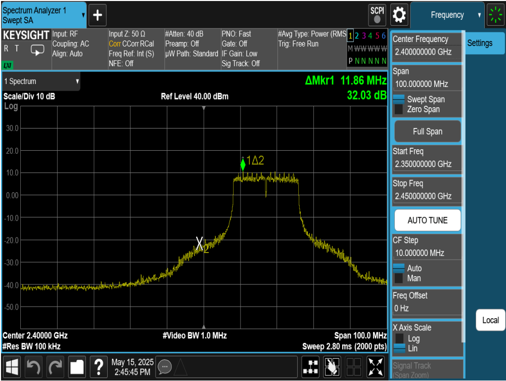
Plot 7-52. Band Edge Plot Antenna WF8 (802.11g – Ch. 2)
