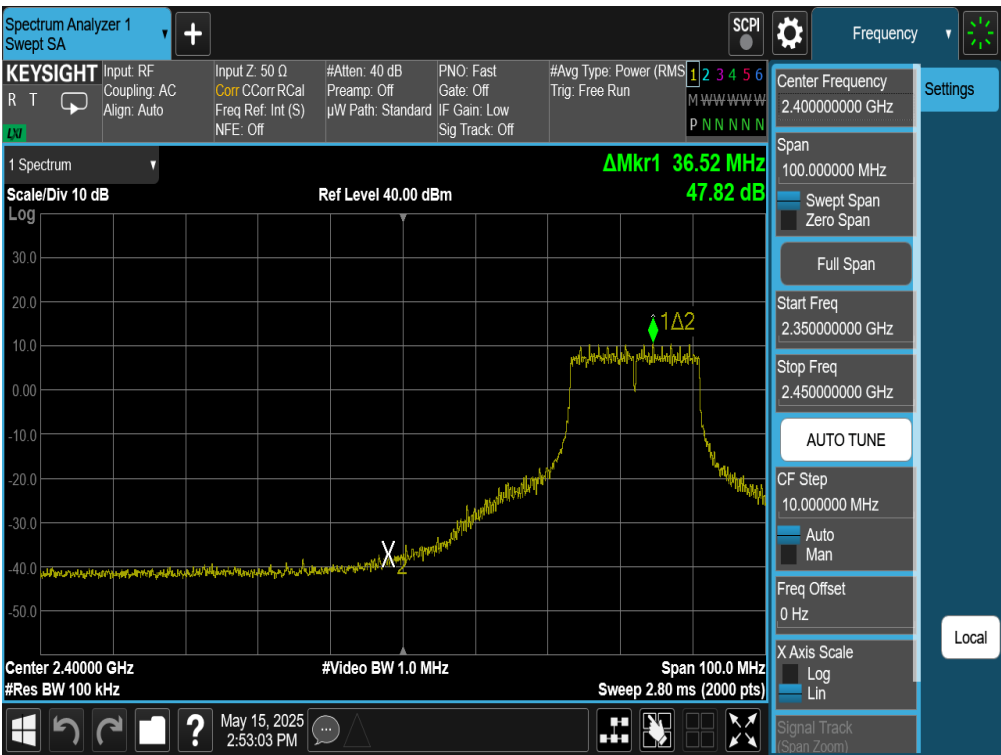
Plot 7-55. Band Edge Plot Antenna WF8 (802.11g – Ch. 5)
