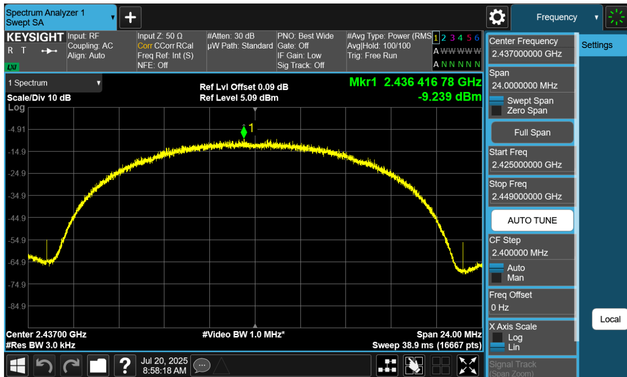
Plot 7-21 PSD Antenna WF9 (20MHz BW 802.11b - Ch.6)
