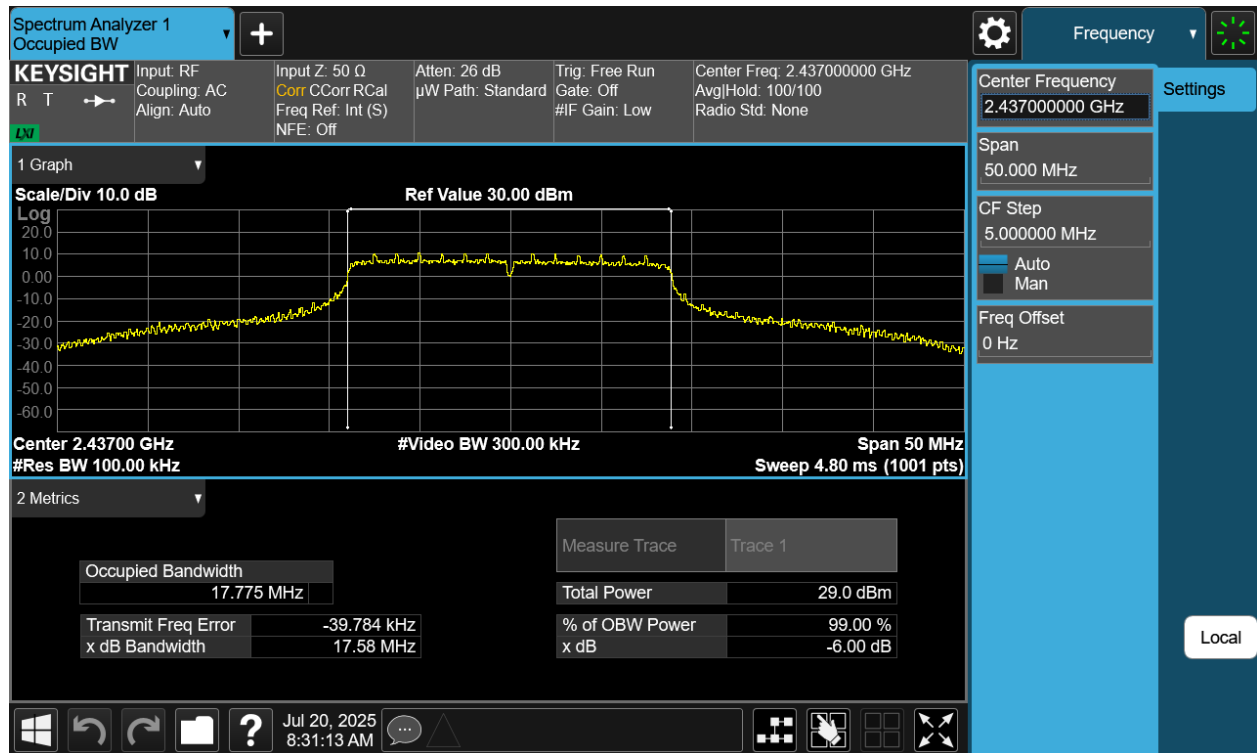
Plot 7-11 6dB BW & 99% OBW Antenna WF9 (20MHz BW 802.11n - Ch.6)
