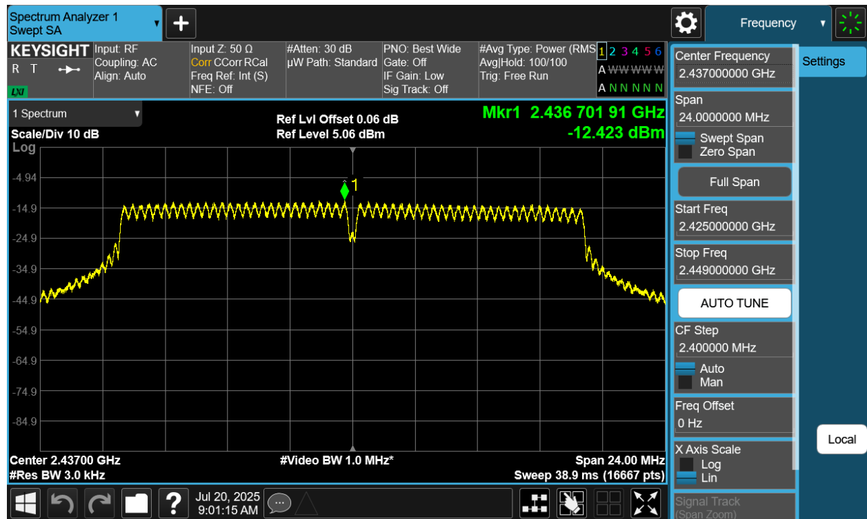
Plot 7-23 PSD Antenna WF9 (20MHz BW 802.11n - Ch.6)
