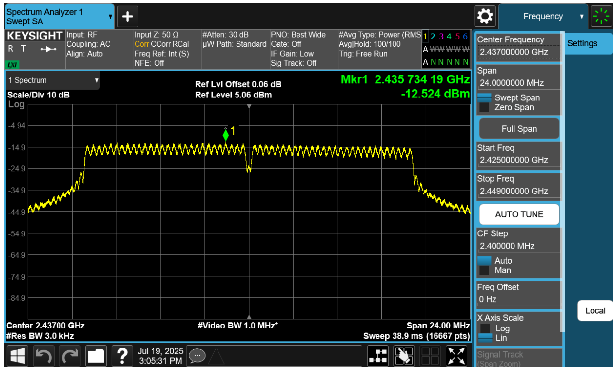
Plot 7-31 PSD CDD Primary Antenna WF7 (20MHz BW 802.11n - Ch.6)
