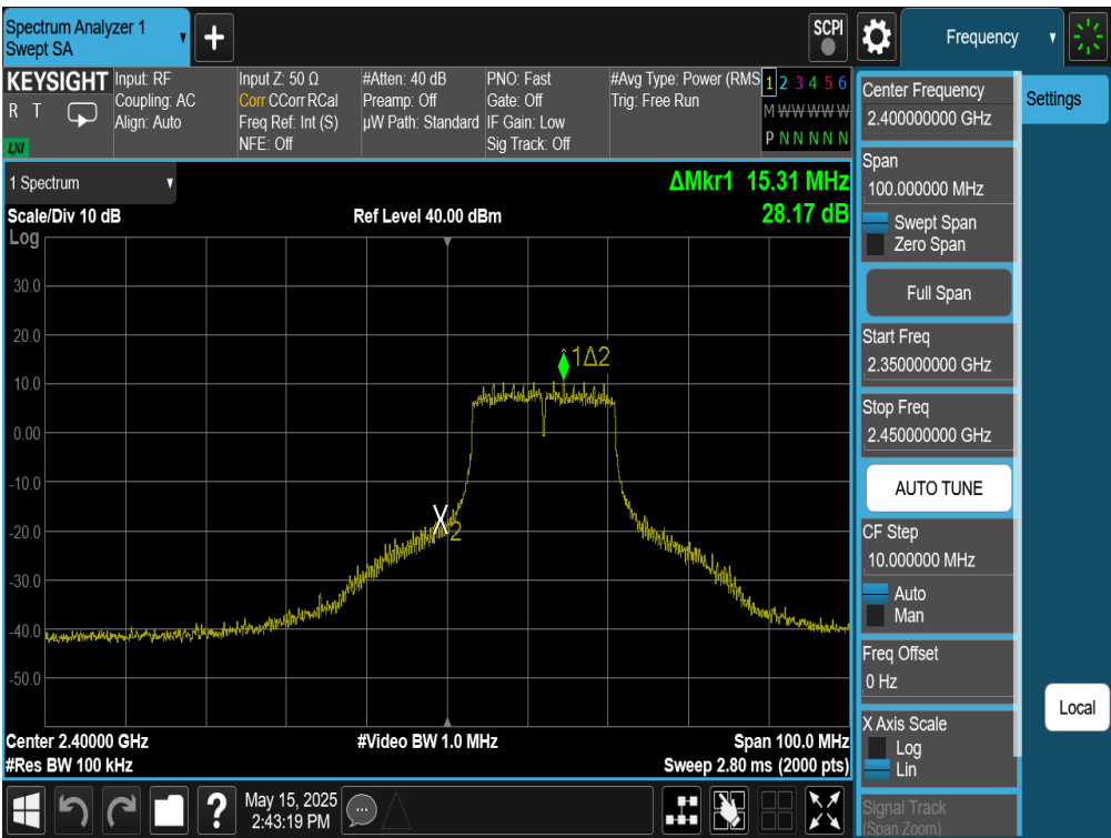
Plot 7-51. Band Edge Plot Antenna WF8 (802.11g – Ch. 1)
