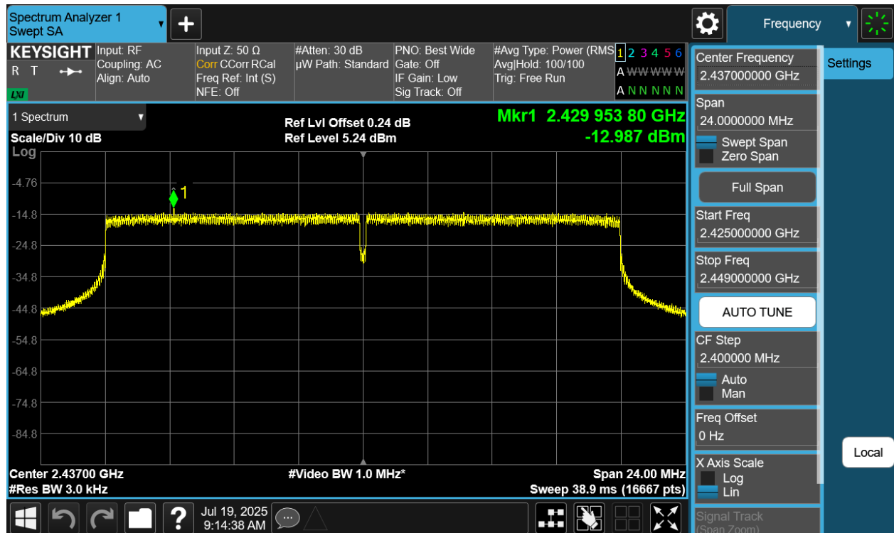
Plot 7-16 PSD Antenna WF8 (20MHz BW 802.11be(SU) - Ch.6)
