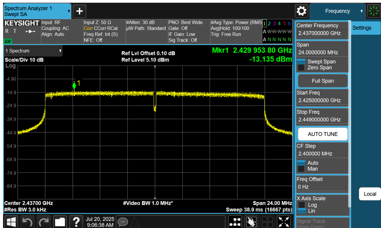
Plot 7-24 PSD Antenna WF9 (20MHz BW 802.11be(SU) - Ch.6)
