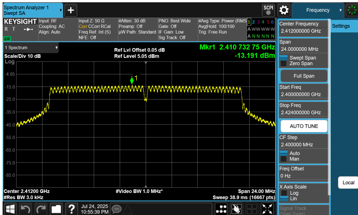
Plot 7-34 PSD CDD Diversity Antenna WF8 (20MHz BW 802.11g - Ch.1)
