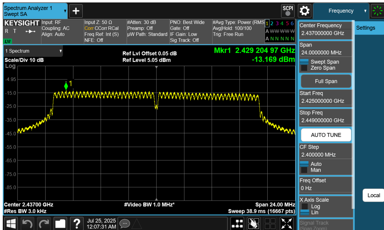
Plot 7-30 PSD CDD Primary Antenna WF7 (20MHz BW 802.11g - Ch.6)
