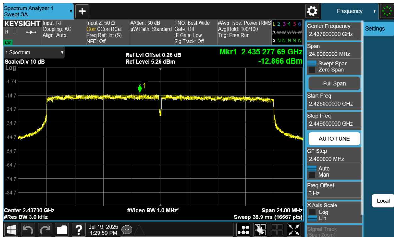
Plot 7-20 PSD Antenna WF7 (20MHz BW 802.11be(SU) - Ch.6)
