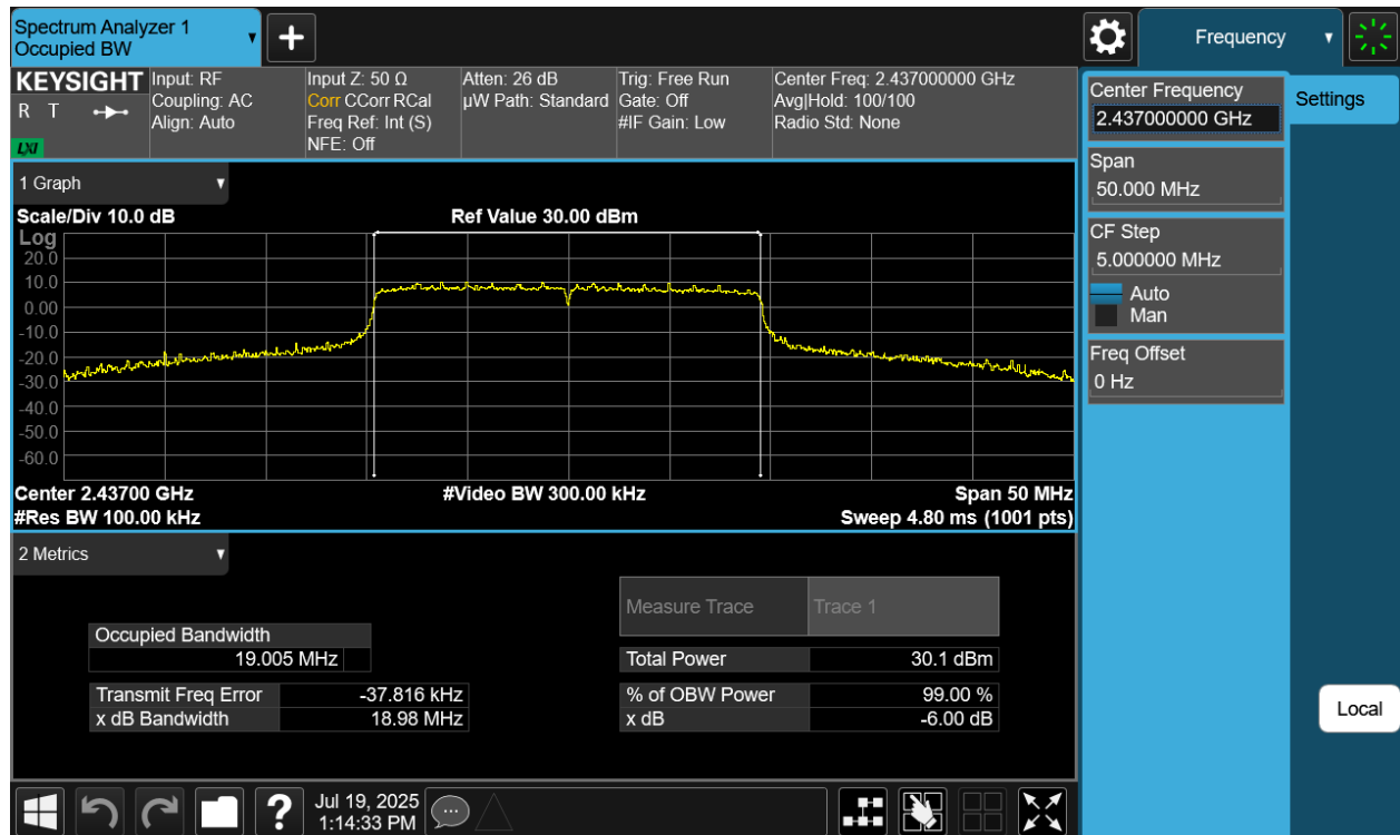
Plot 7-8 6dB BW & 99% OBW Antenna WF7 (20MHz BW 802.11be(SU) - Ch.6)
