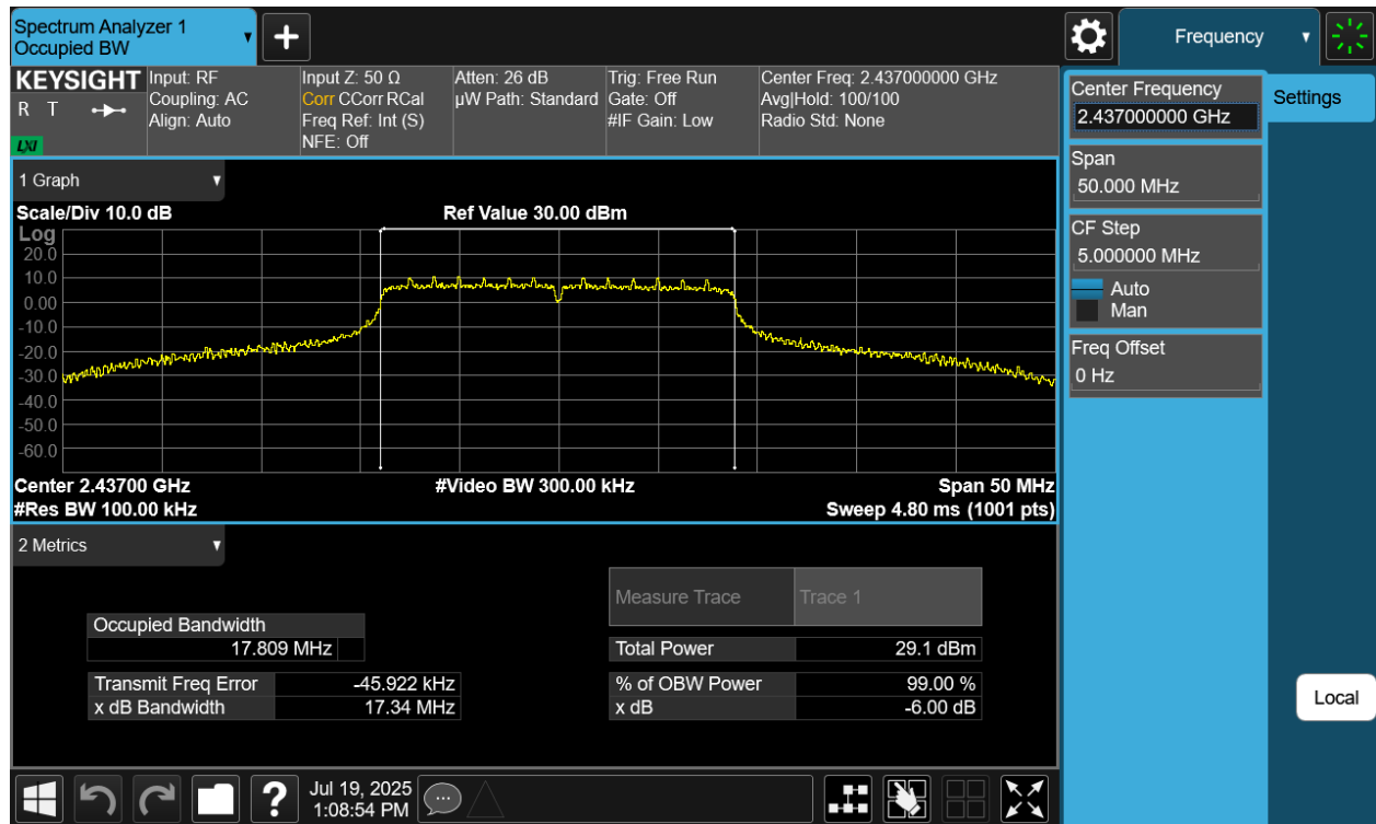
Plot 7-7 6dB BW & 99% OBW Antenna WF7 (20MHz BW 802.11n - Ch.6)
