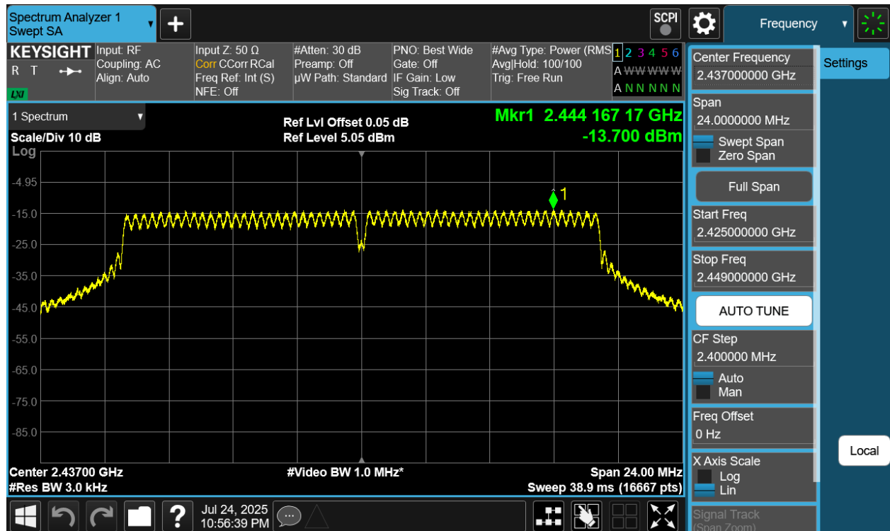
Plot 7-26 PSD CDD Primary Antenna WF8 (20MHz BW 802.11g - Ch.6)
