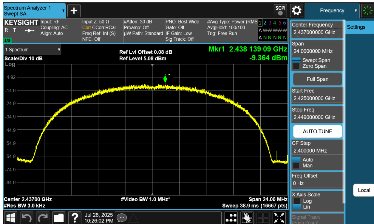
Plot 7-33 PSD CDD Diversity Antenna WF8 (20MHz BW 802.11b - Ch.6)
