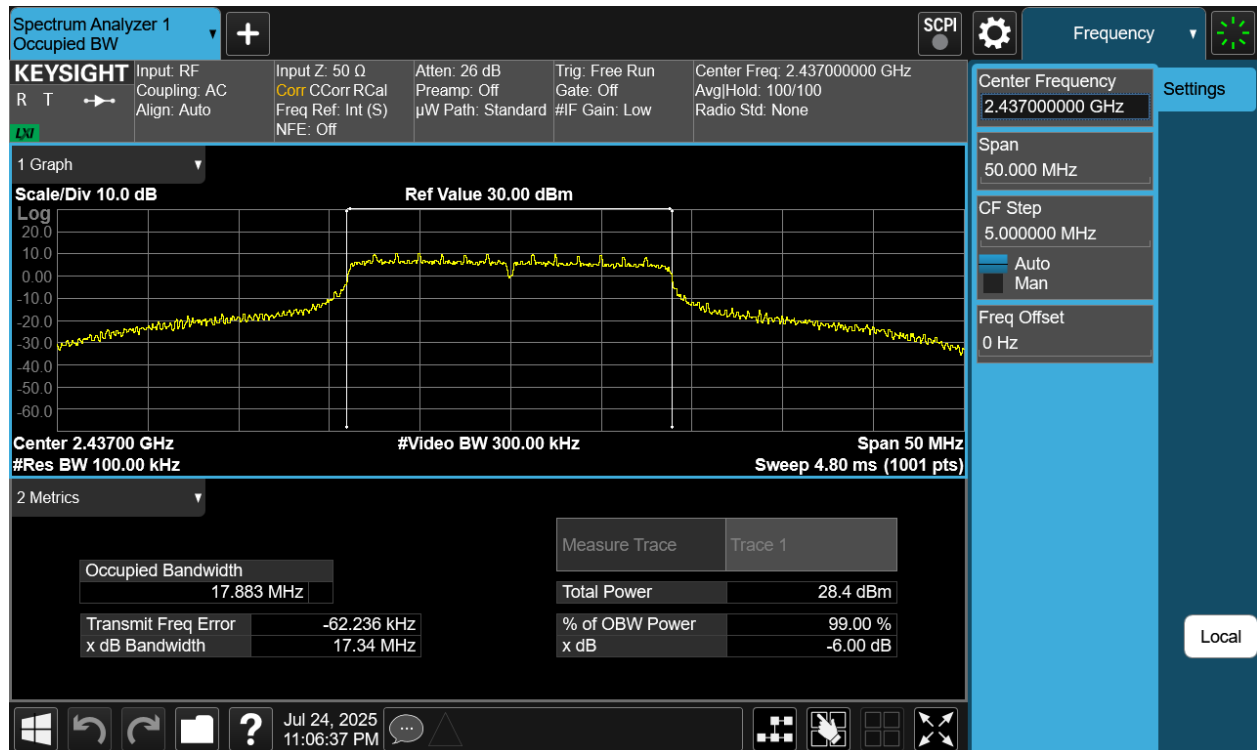
Plot 7-6 6dB BW & 99% OBW Antenna WF7 (20MHz BW 802.11g - Ch.6)
