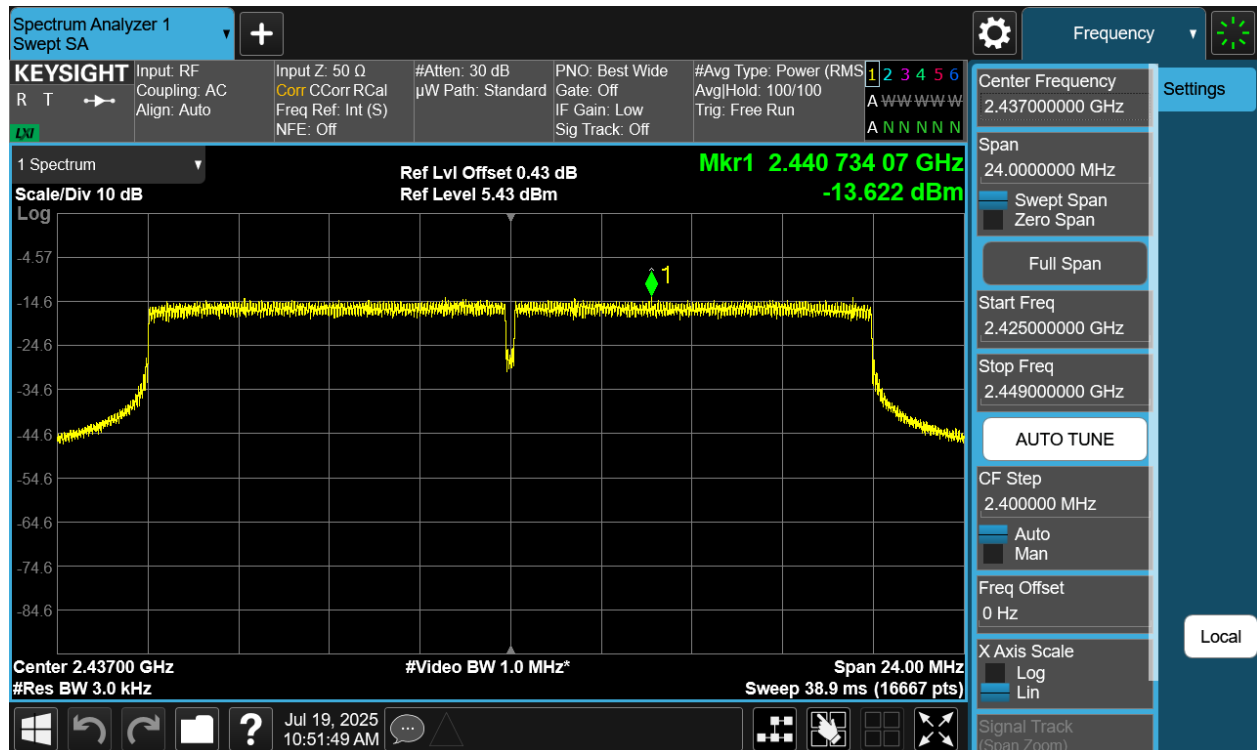
Plot 7-28 PSD CDD Primary Antenna WF8 (20MHz BW 802.11be(SU) - Ch.6)
