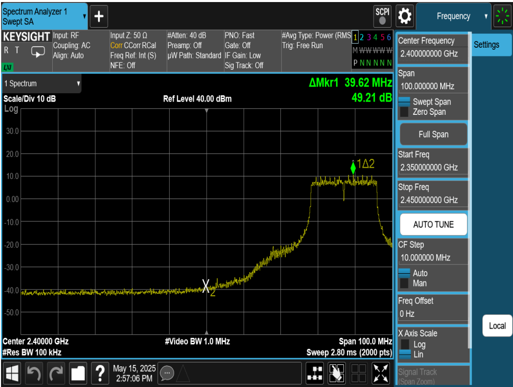
Plot 7-56. Band Edge Plot Antenna WF8 (802.11g – Ch. 6)
