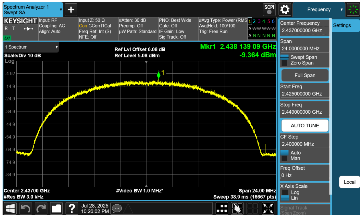
Plot 7-25 PSD CDD Primary Antenna WF8 (20MHz BW 802.11b - Ch.6)
