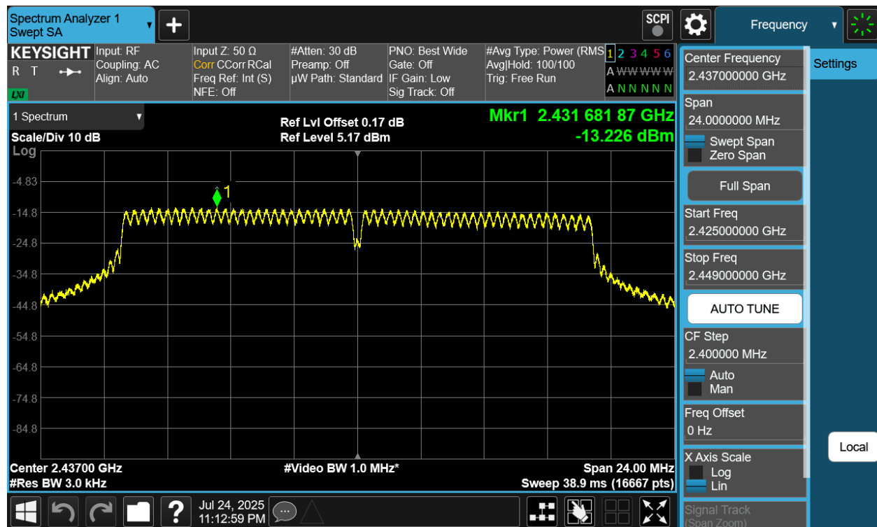
Plot 7-18 PSD Antenna WF7 (20MHz BW 802.11g - Ch.6)
