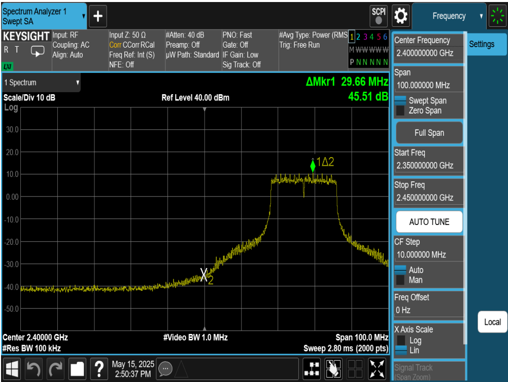
Plot 7-54. Band Edge Plot Antenna WF8 (802.11g – Ch. 4)
