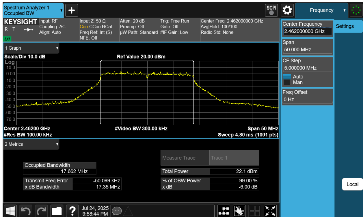
Plot 7-2 6dB BW & 99% OBW Antenna WF8 (20MHz BW 802.11g - Ch.11)
