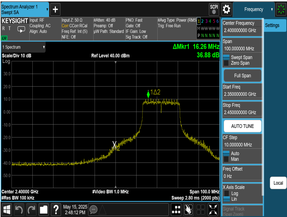
Plot 7-53. Band Edge Plot Antenna WF8 (802.11g – Ch. 3)
