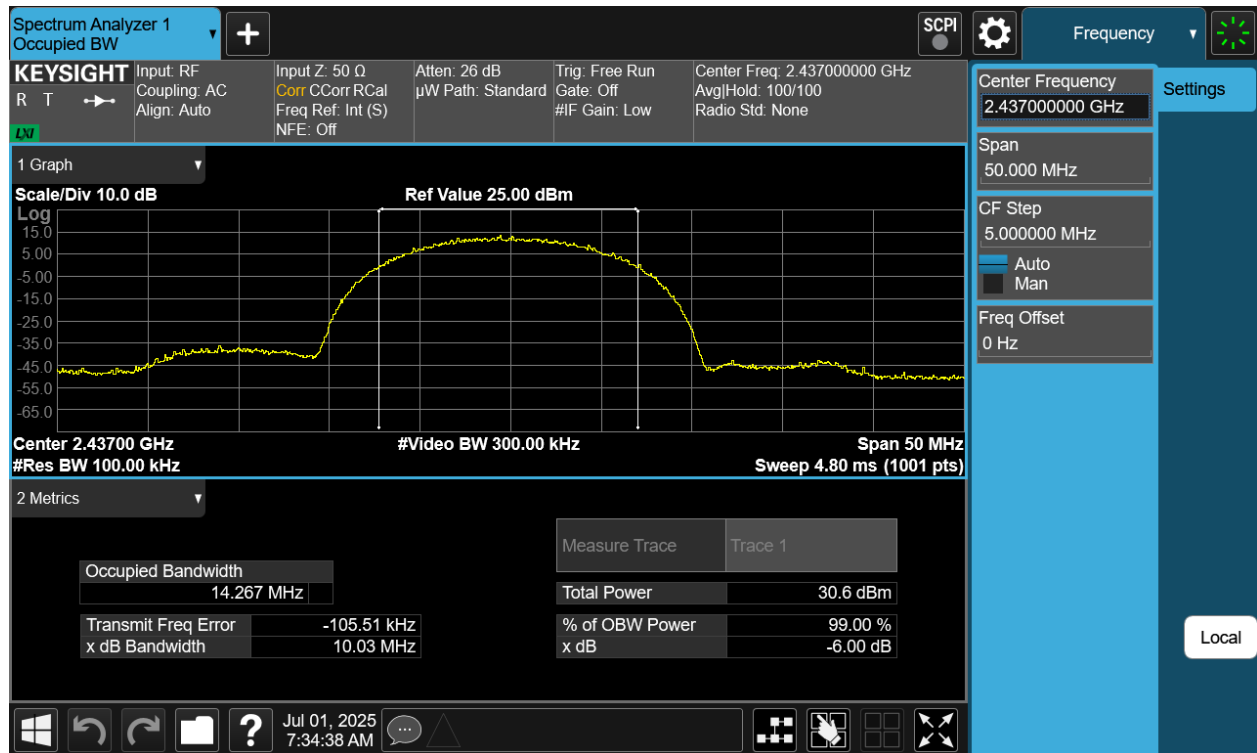
Plot 7-5 6dB BW & 99% OBW Antenna WF7 (20MHz BW 802.11b - Ch.6)
