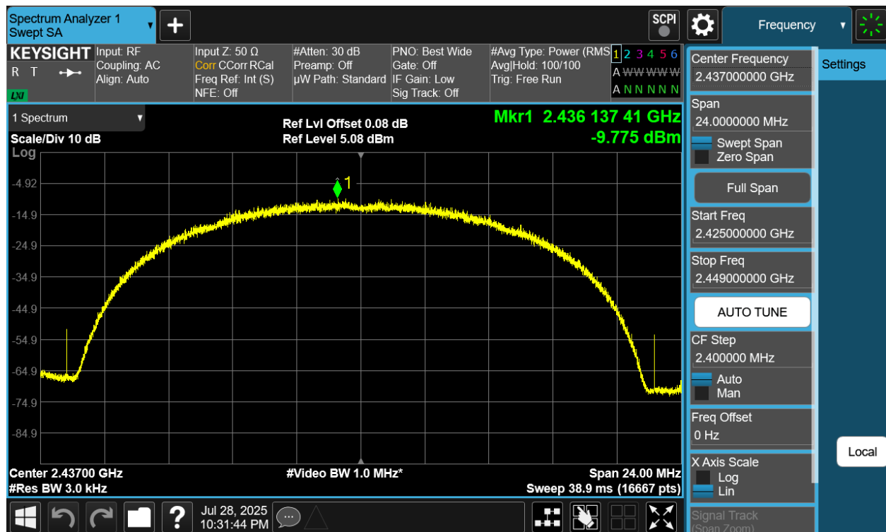
Plot 7-29 PSD CDD Primary Antenna WF7 (20MHz BW 802.11b - Ch.6)
