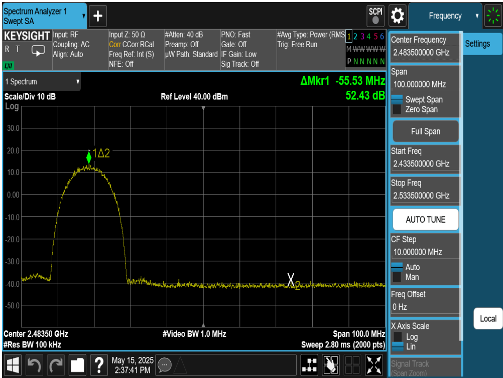
Plot 7-46. Band Edge Plot Antenna WF8 (802.11b – Ch. 9)
