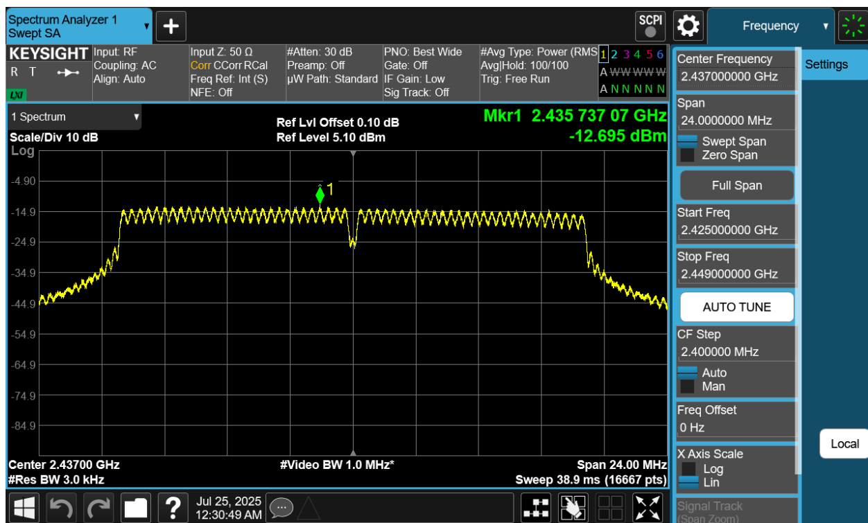
Plot 7-22 PSD Antenna WF9 (20MHz BW 802.11g - Ch.6)
