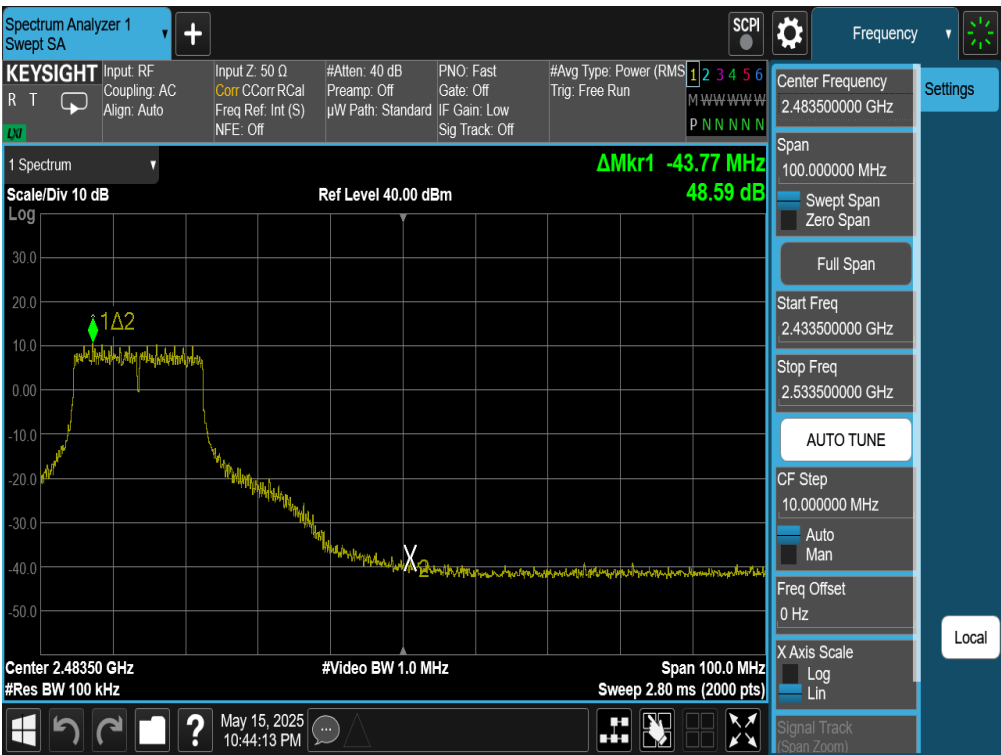
Plot 7-121. Band Edge Plot Antenna WF7 (802.11n (2.4GHz) – Ch. 8)
