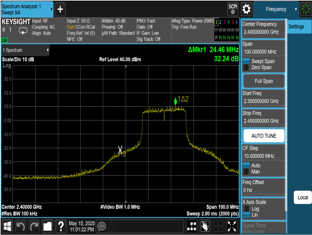
Plot 7-128. Band Edge Plot Antenna WF7 (802.11be (SU - 2.4GHz) – Ch. 2)
