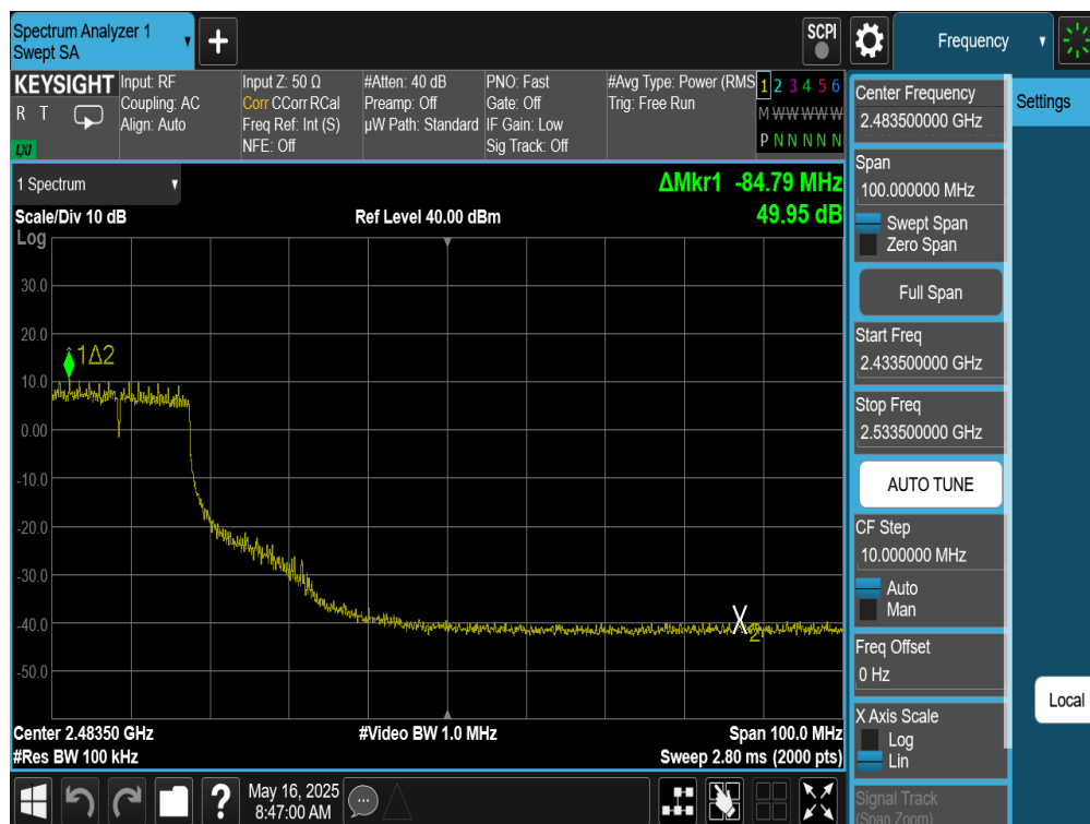
Plot 7-157. Band Edge Plot Antenna WF9 (802.11g – Ch. 7)
