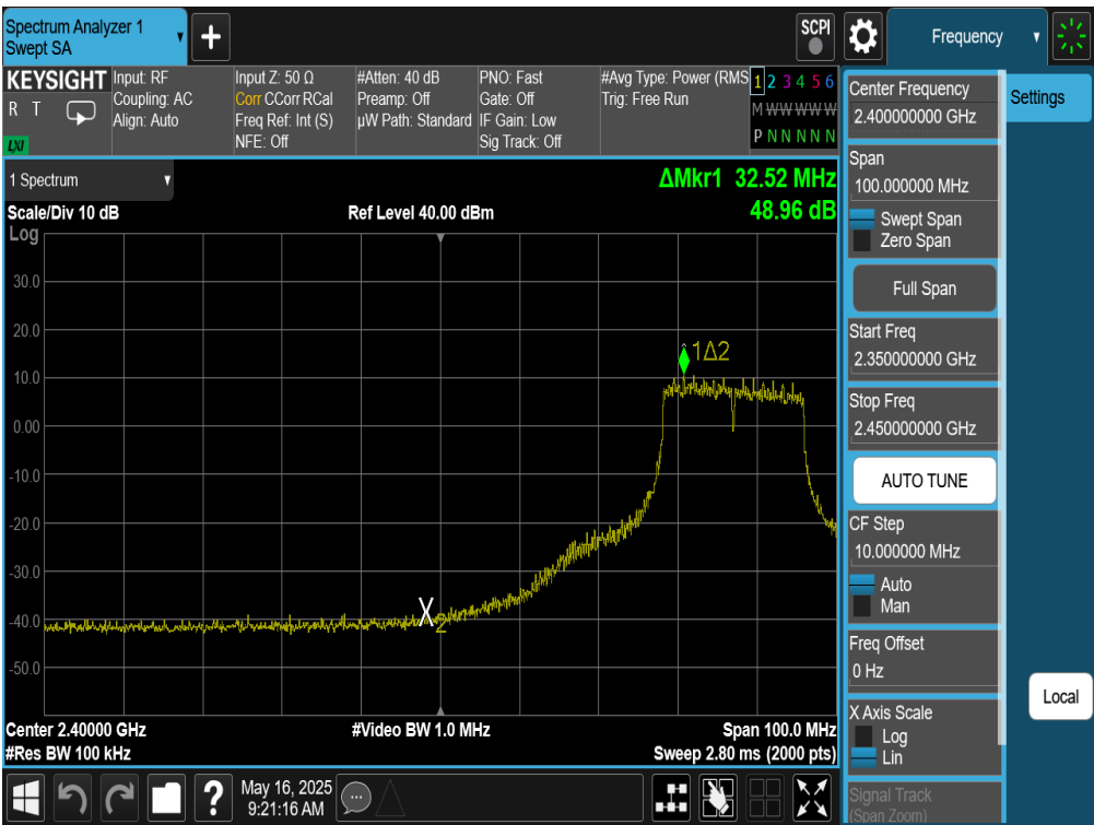
Plot 7-169. Band Edge Plot Antenna WF9 (802.11n (2.4GHz) – Ch. 6)
