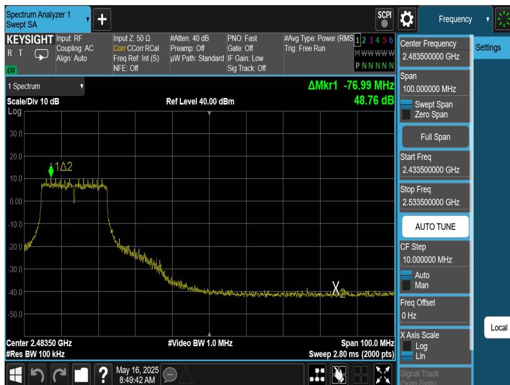
Plot 7-158. Band Edge Plot Antenna WF9 (802.11g – Ch. 8)
