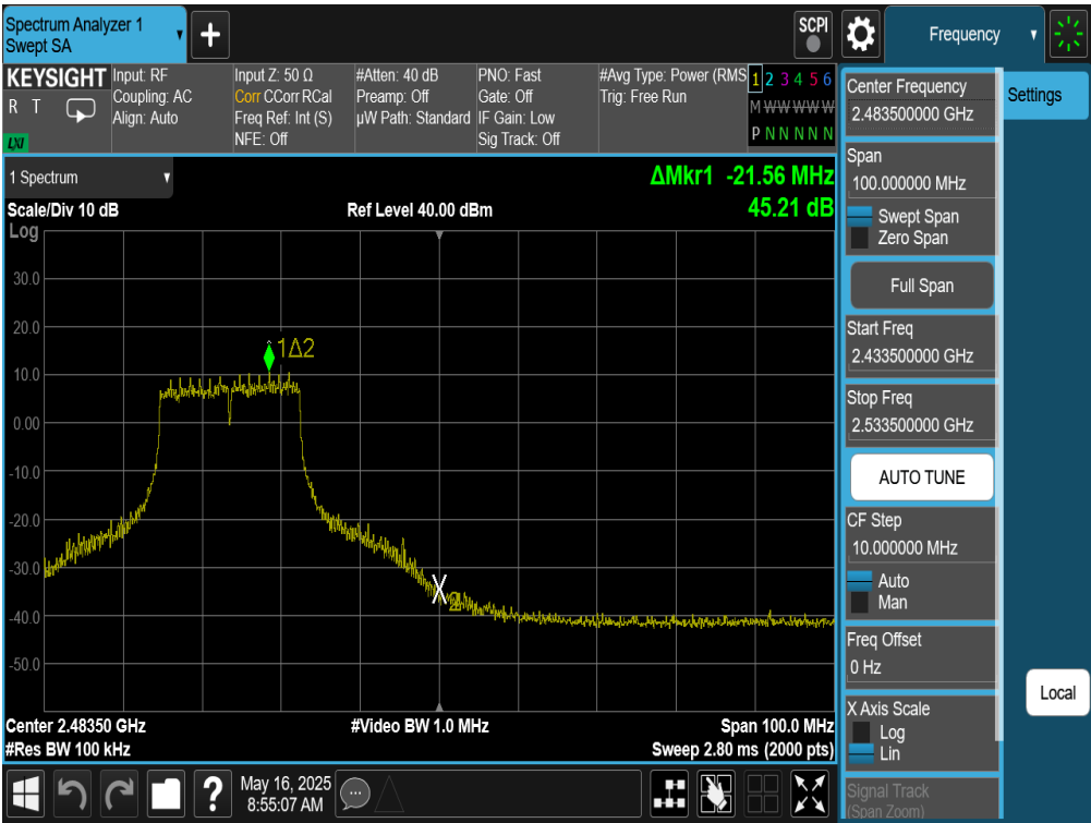
Plot 7-160. Band Edge Plot Antenna WF9 (802.11g – Ch. 10)
