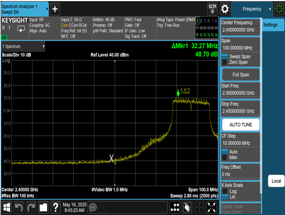
Plot 7-156. Band Edge Plot Antenna WF9 (802.11g – Ch. 6)
