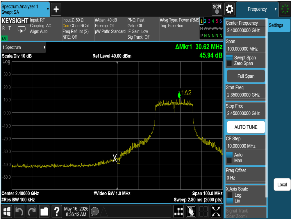
Plot 7-154. Band Edge Plot Antenna WF9 (802.11g – Ch. 4)
