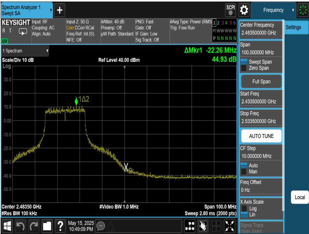
Plot 7-123. Band Edge Plot Antenna WF7 (802.11n (2.4GHz) – Ch. 10)
