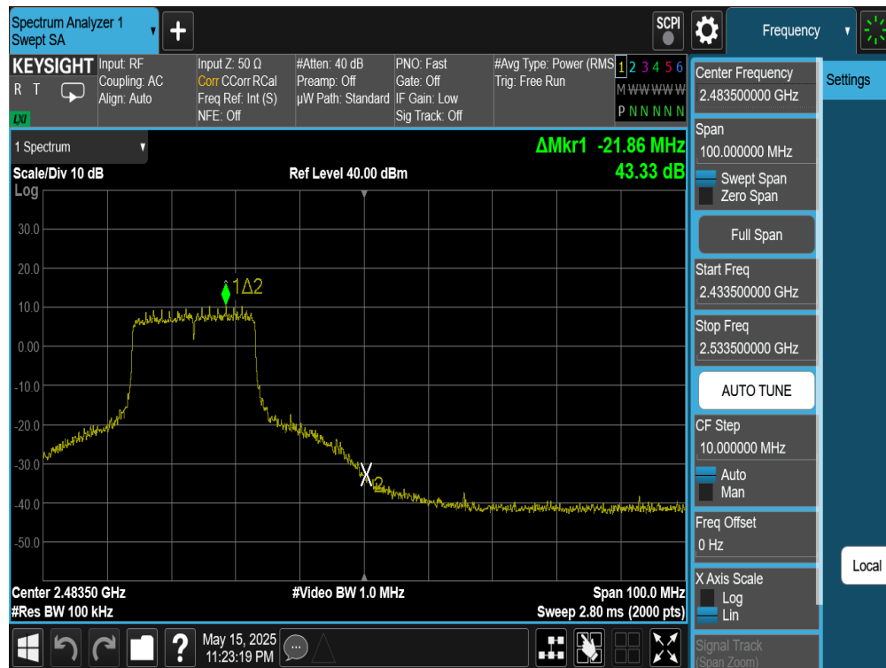
Plot 7-137. Band Edge Plot Antenna WF7 (802.11be (SU - 2.4GHz) – Ch. 10)
