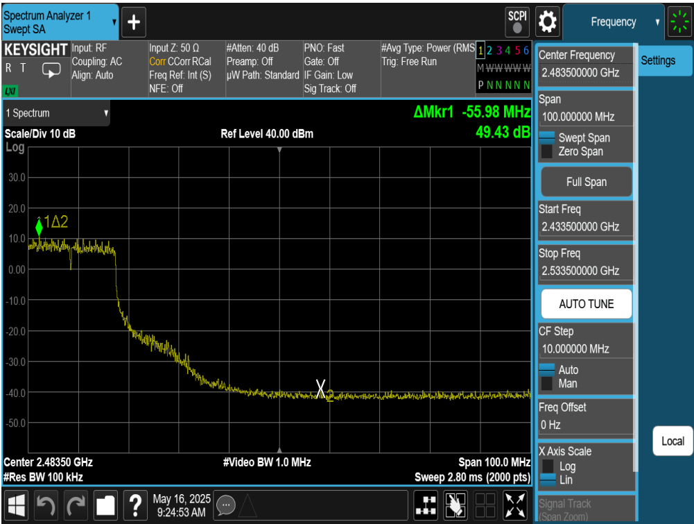
Plot 7-170. Band Edge Plot Antenna WF9 (802.11n (2.4GHz) – Ch. 7)
