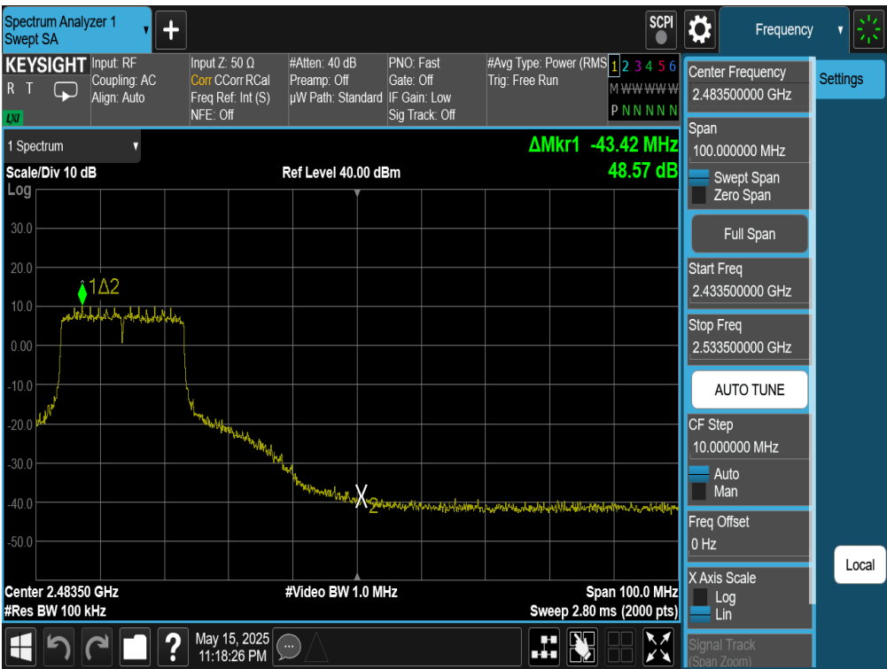
Plot 7-135. Band Edge Plot Antenna WF7 (802.11be (SU - 2.4GHz) – Ch. 8)
