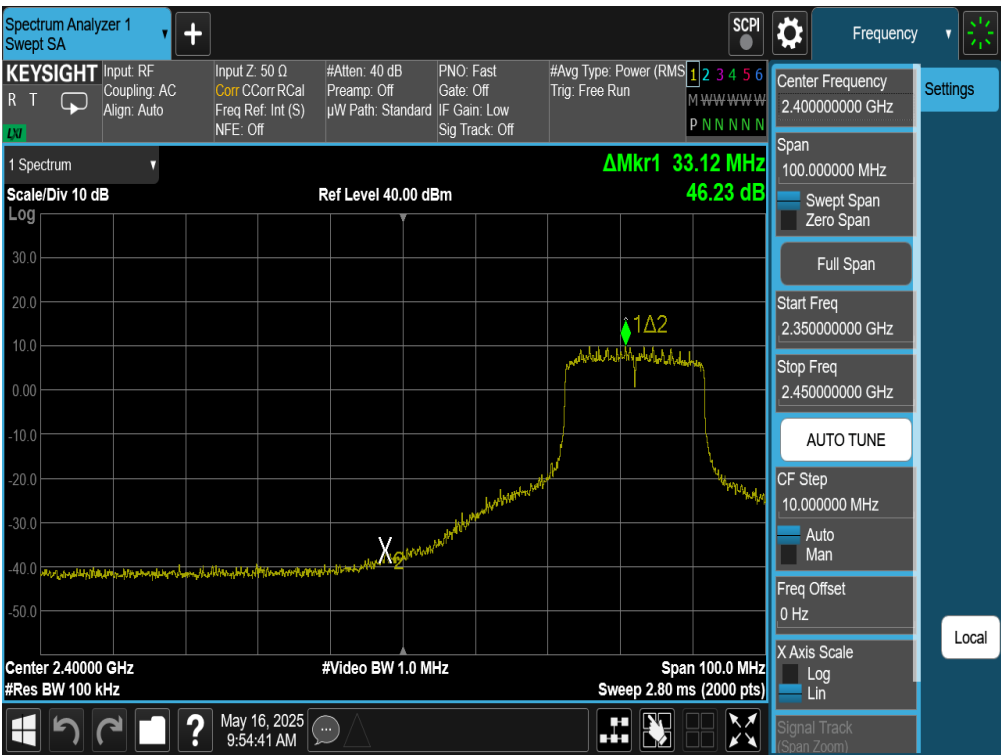
Plot 7-181. Band Edge Plot Antenna WF9 (802.11be (SU - 2.4GHz) – Ch. 5)
