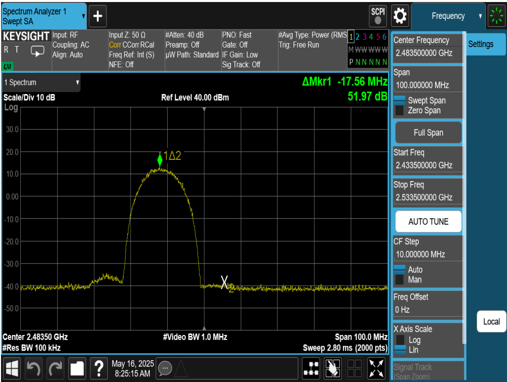
Plot 7-150. Band Edge Plot Antenna WF9 (802.11b – Ch. 13)
