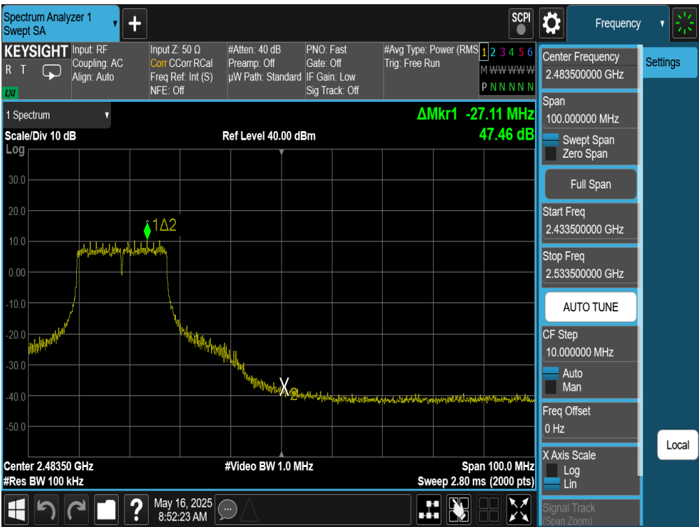
Plot 7-159. Band Edge Plot Antenna WF9 (802.11g – Ch. 9)
