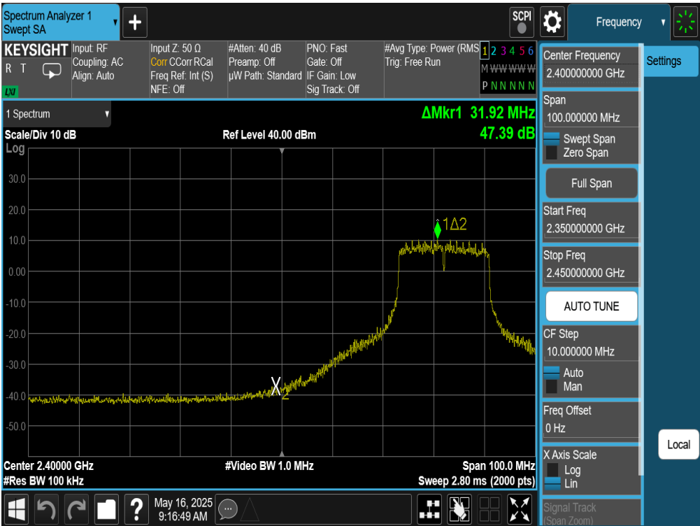
Plot 7-168. Band Edge Plot Antenna WF9 (802.11n (2.4GHz) – Ch. 5)
