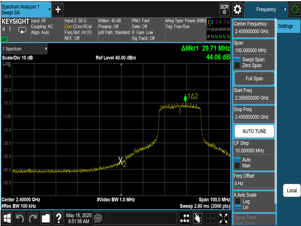
Plot 7-180. Band Edge Plot Antenna WF9 (802.11be (SU - 2.4GHz) – Ch. 4)
