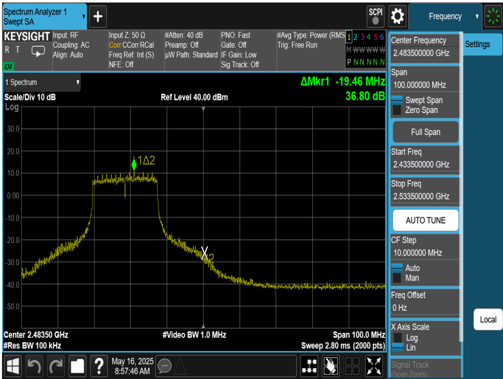
Plot 7-161. Band Edge Plot Antenna WF9 (802.11g – Ch. 11)
