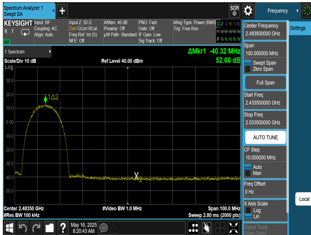
Plot 7-145. Band Edge Plot Antenna WF9 (802.11b – Ch. 8)
