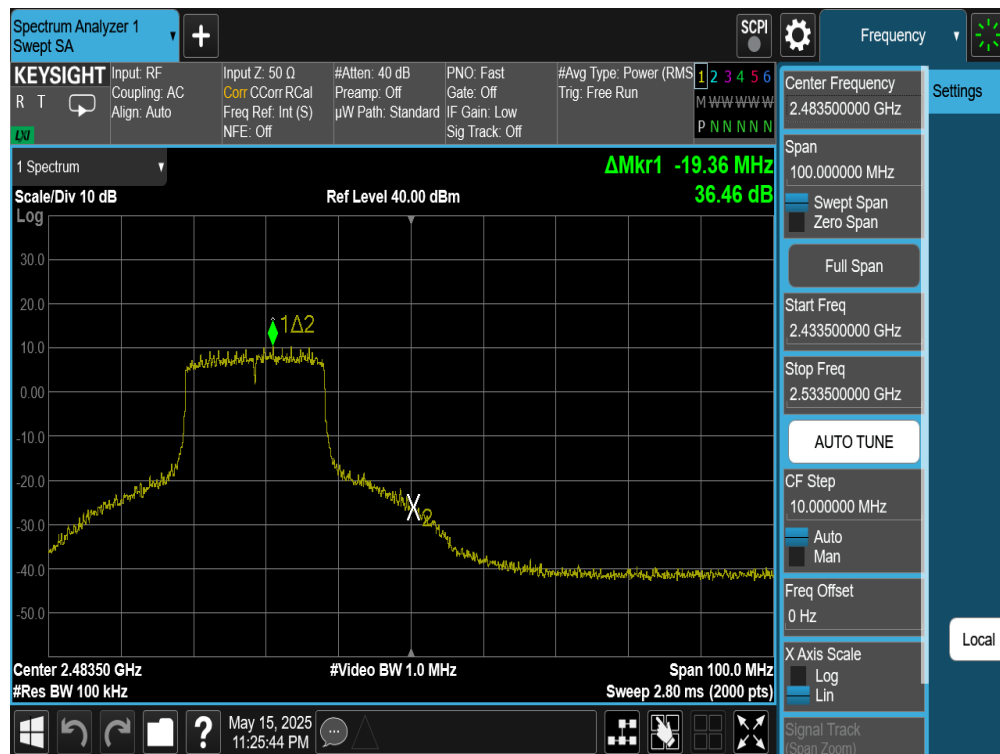
Plot 7-138. Band Edge Plot Antenna WF7 (802.11be (SU - 2.4GHz) – Ch. 11)
