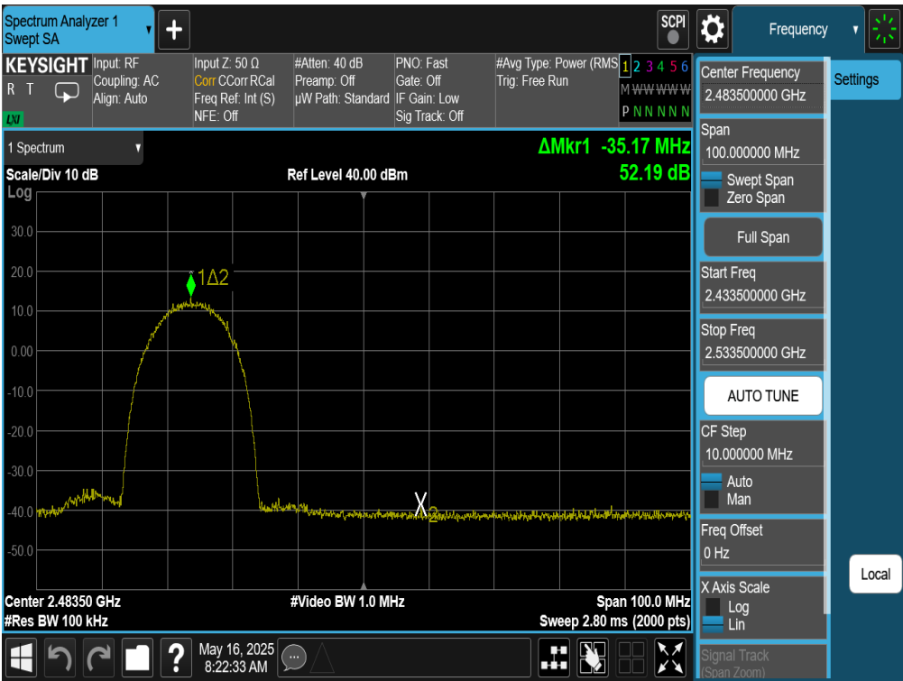
Plot 7-147. Band Edge Plot Antenna WF9 (802.11b - Ch. 10)
