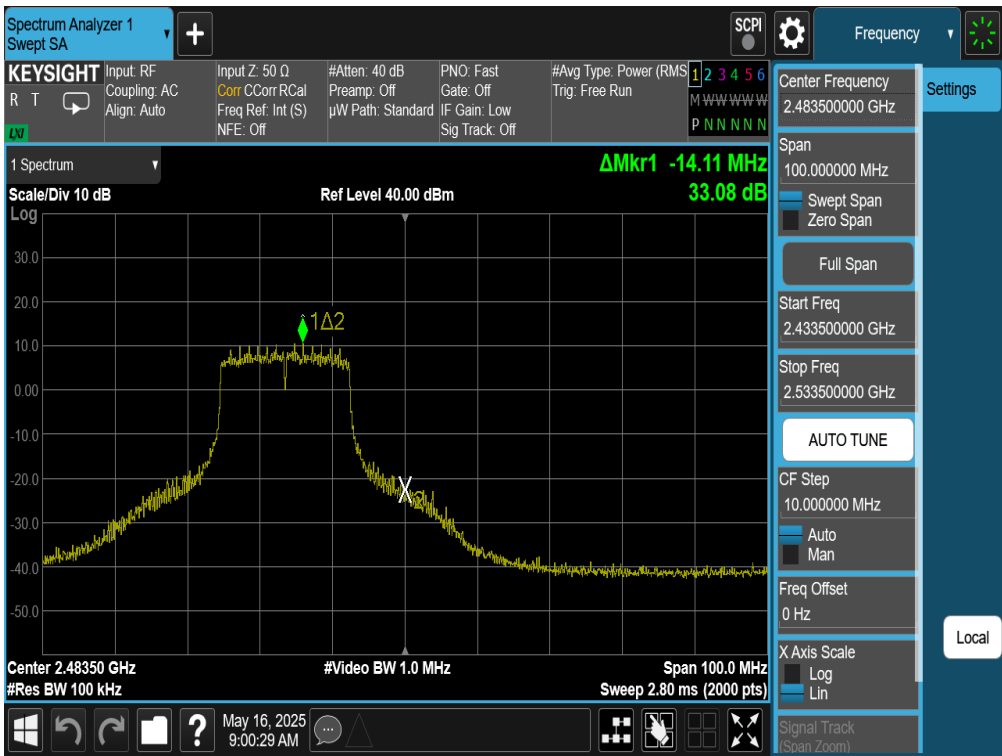
Plot 7-162. Band Edge Plot Antenna WF9 (802.11g – Ch. 12)
