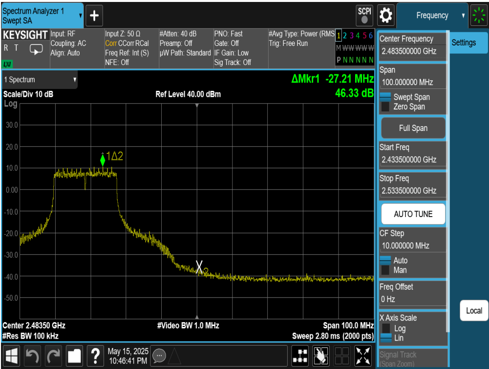
Plot 7-122. Band Edge Plot Antenna WF7 (802.11n (2.4GHz) – Ch. 9)
