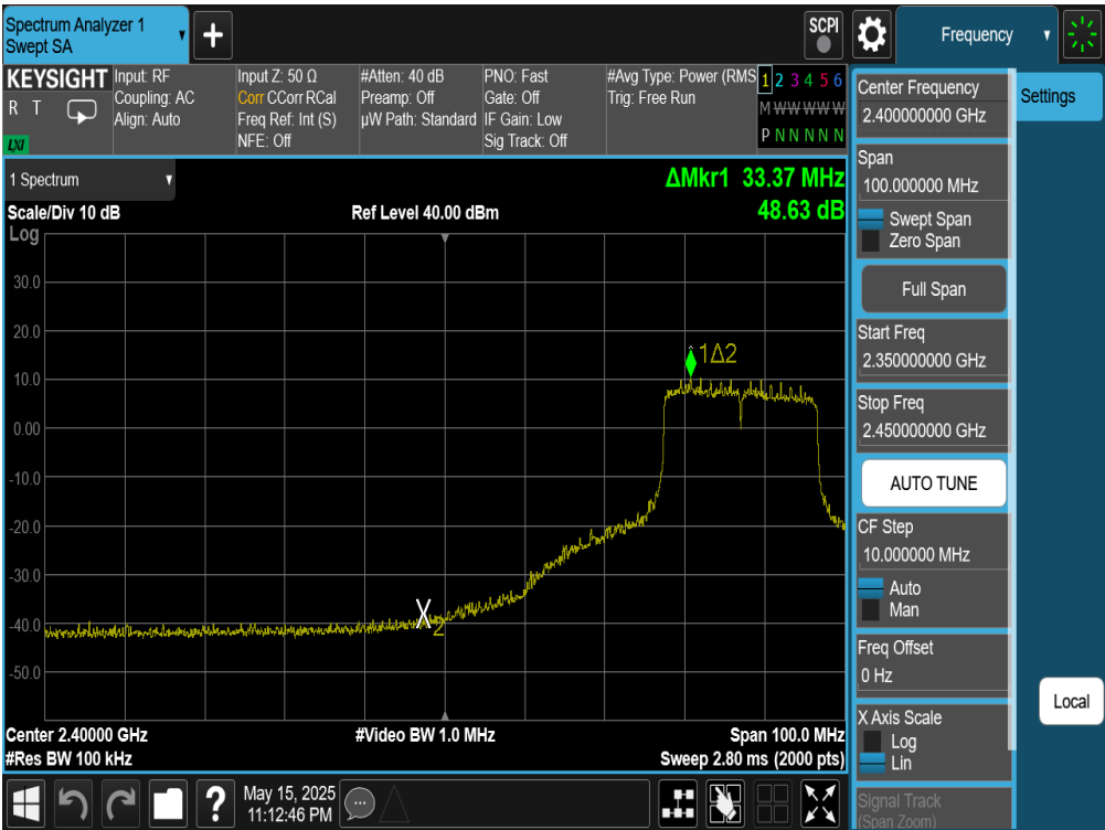
Plot 7-132. Band Edge Plot Antenna WF7 (802.11be (SU - 2.4GHz) – Ch. 6)
