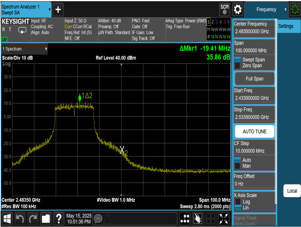
Plot 7-124. Band Edge Plot Antenna WF7 (802.11n (2.4GHz) – Ch. 11)
