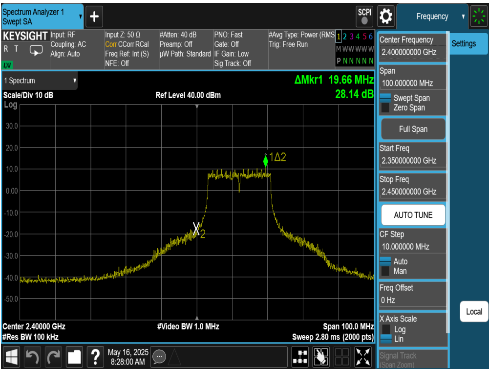
Plot 7-151. Band Edge Plot Antenna WF9 (802.11g – Ch. 1)
