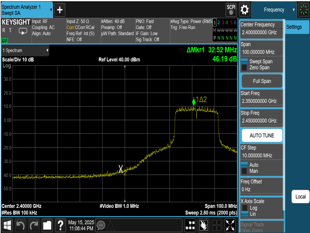
Plot 7-131. Band Edge Plot Antenna WF7 (802.11be (SU - 2.4GHz) – Ch. 5)
