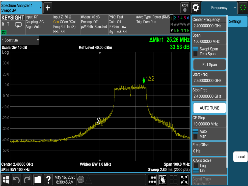
Plot 7-152. Band Edge Plot Antenna WF9 (802.11g – Ch. 2)
