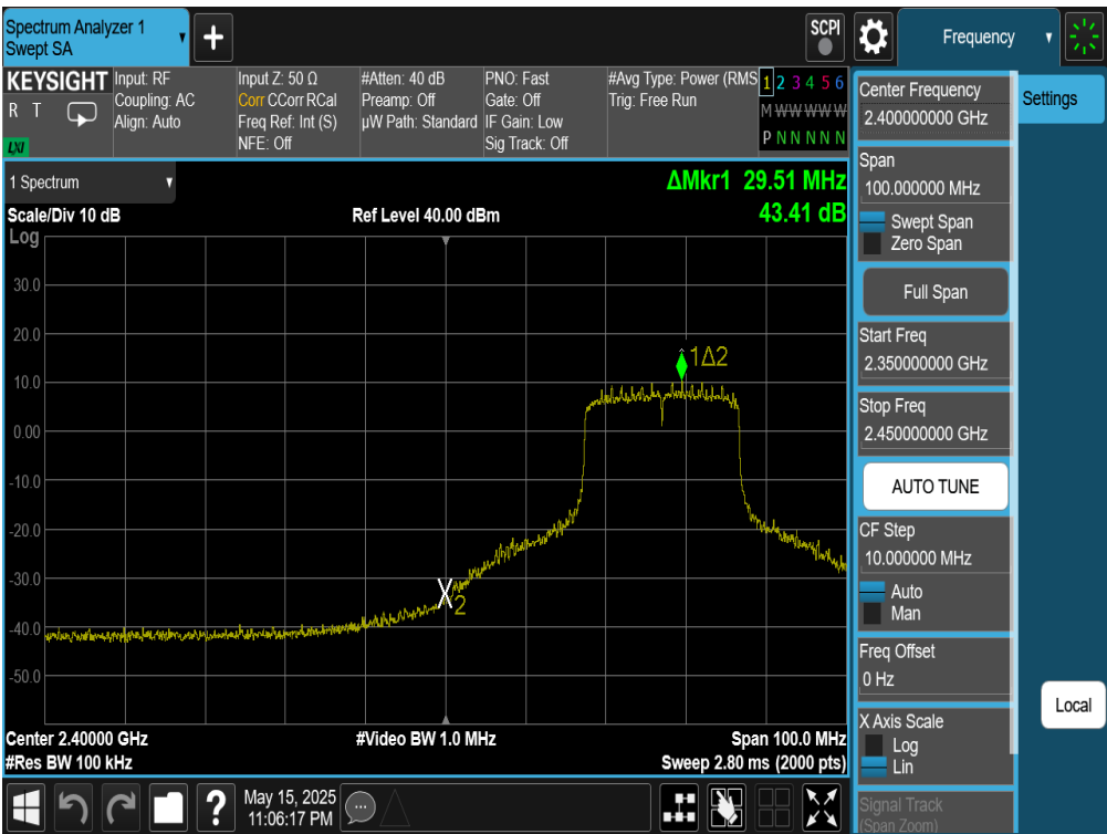
Plot 7-130. Band Edge Plot Antenna WF7 (802.11be (SU - 2.4GHz) – Ch. 4)
