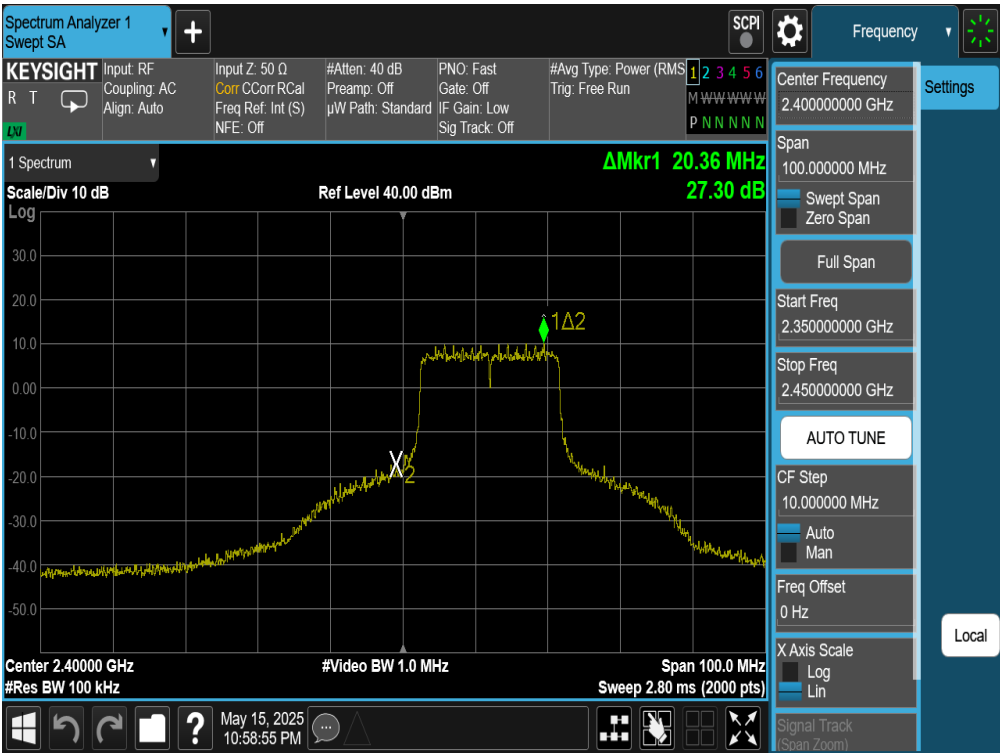
Plot 7-127. Band Edge Plot Antenna WF7 (802.11be (SU - 2.4GHz) – Ch. 1)
