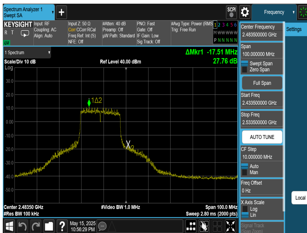
Plot 7-126. Band Edge Plot Antenna WF7 (802.11n (2.4GHz) – Ch. 13)
