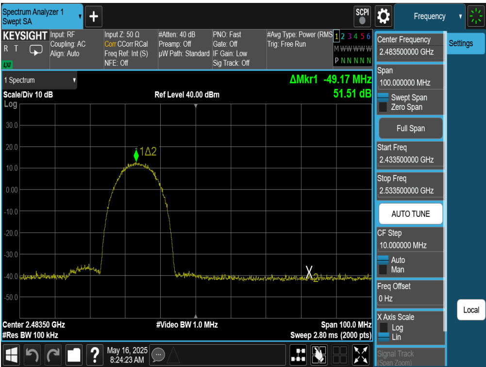
Plot 7-149. Band Edge Plot Antenna WF9 (802.11b – Ch. 12)
