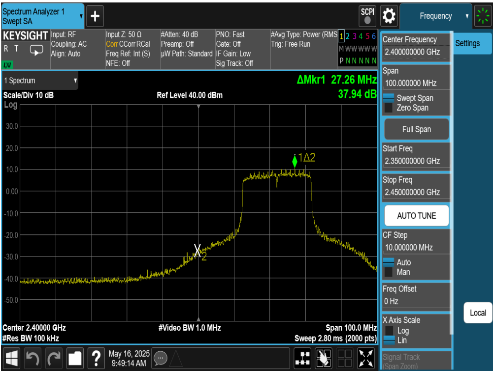
Plot 7-179. Band Edge Plot Antenna WF9 (802.11be (SU - 2.4GHz) – Ch. 3)
