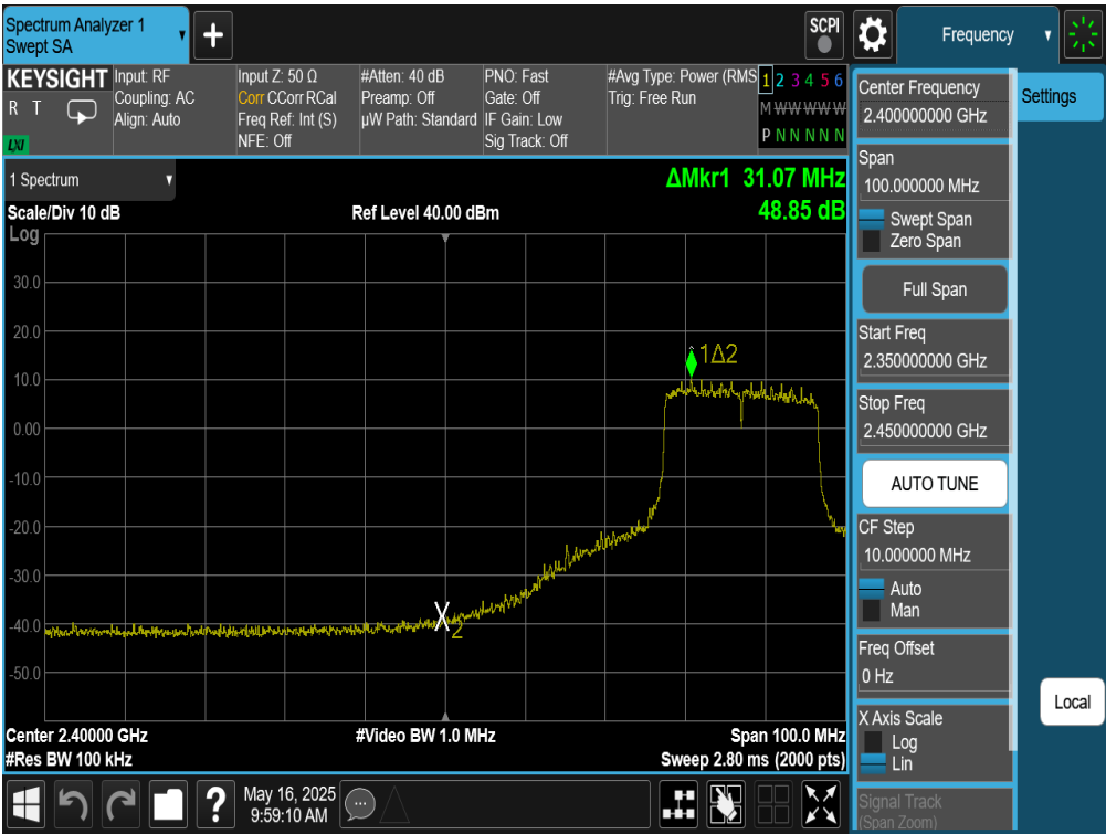
Plot 7-182. Band Edge Plot Antenna WF9 (802.11be (SU - 2.4GHz) – Ch. 6)
