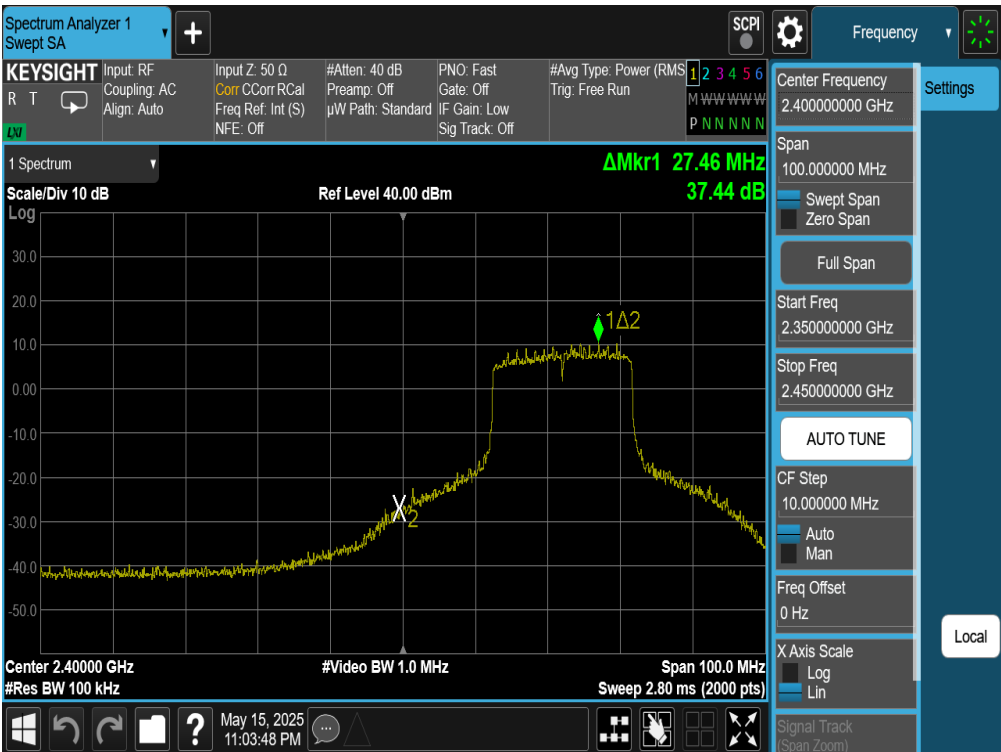
Plot 7-129. Band Edge Plot Antenna WF7 (802.11be (SU - 2.4GHz) – Ch. 3)
