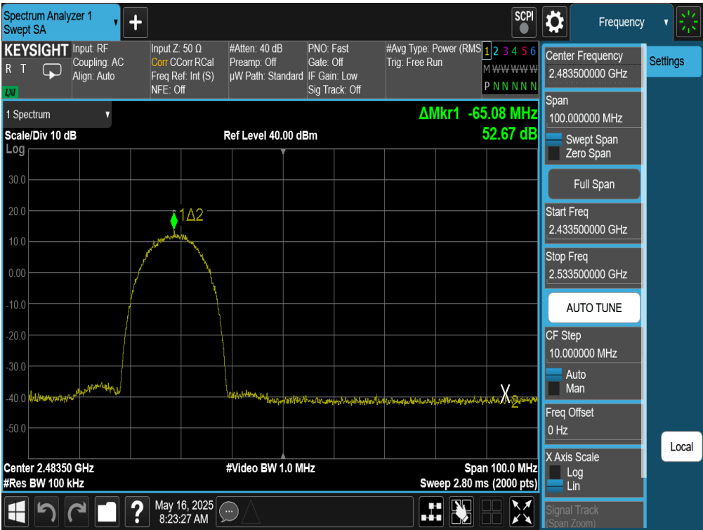
Plot 7-148. Band Edge Plot Antenna WF9 (802.11b - Ch. 11)
