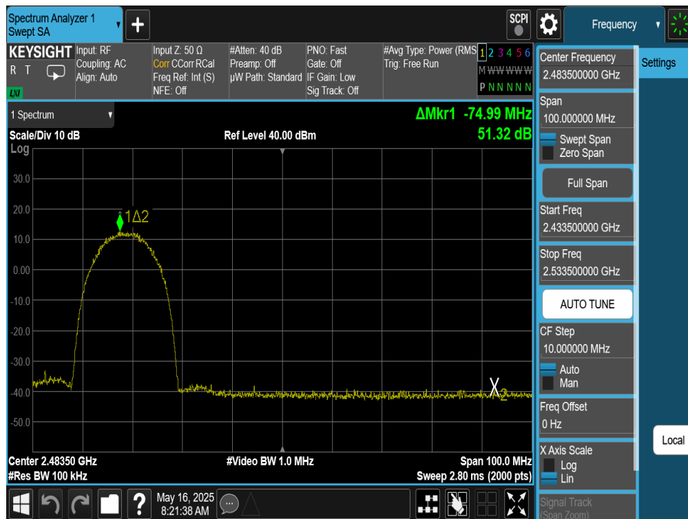
Plot 7-146. Band Edge Plot Antenna WF9 (802.11b – Ch. 9)
