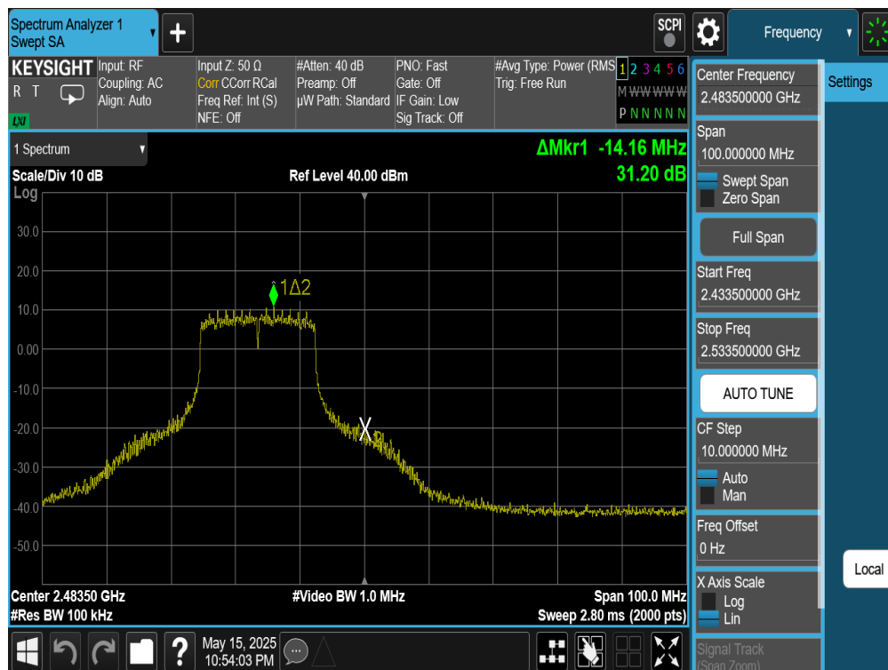
Plot 7-125. Band Edge Plot Antenna WF7 (802.11n (2.4GHz) – Ch. 12)
