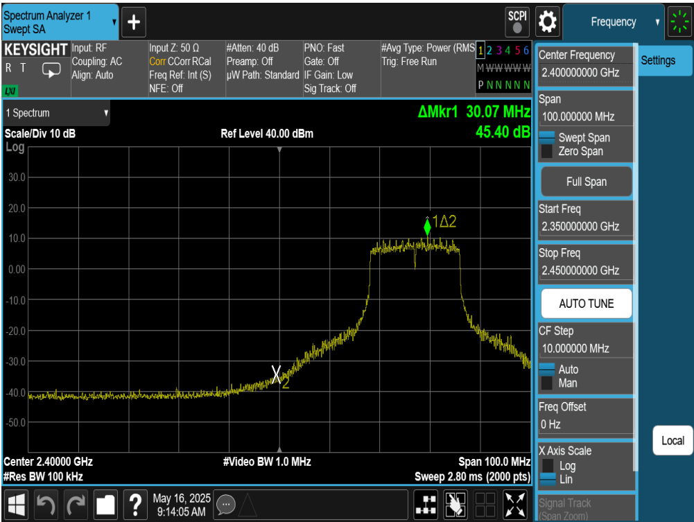
Plot 7-167. Band Edge Plot Antenna WF9 (802.11n (2.4GHz) – Ch. 4)
