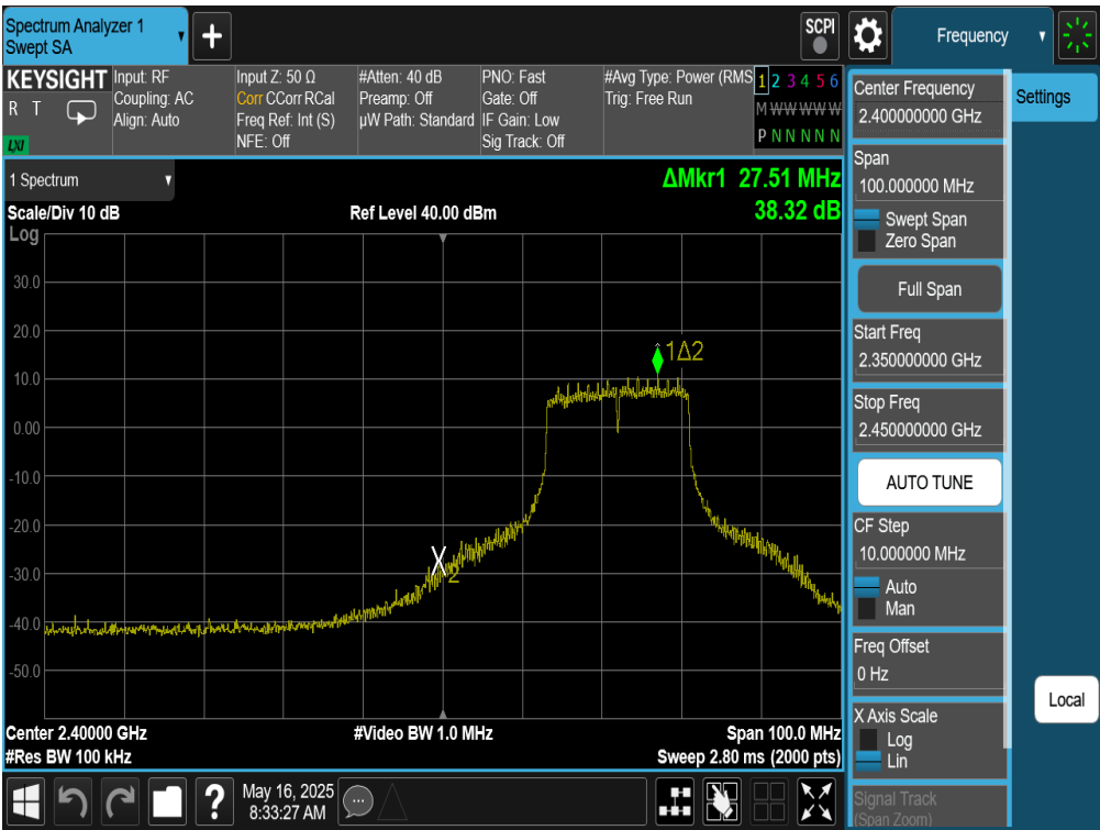
Plot 7-153. Band Edge Plot Antenna WF9 (802.11g – Ch. 3)
