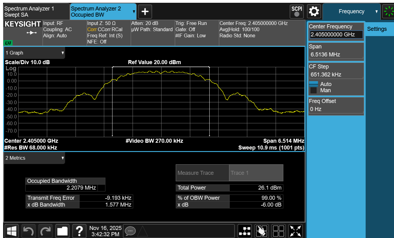
Plot 7-1. 99% OBW Antenna 3a (802.15.4, Ch. 11)
