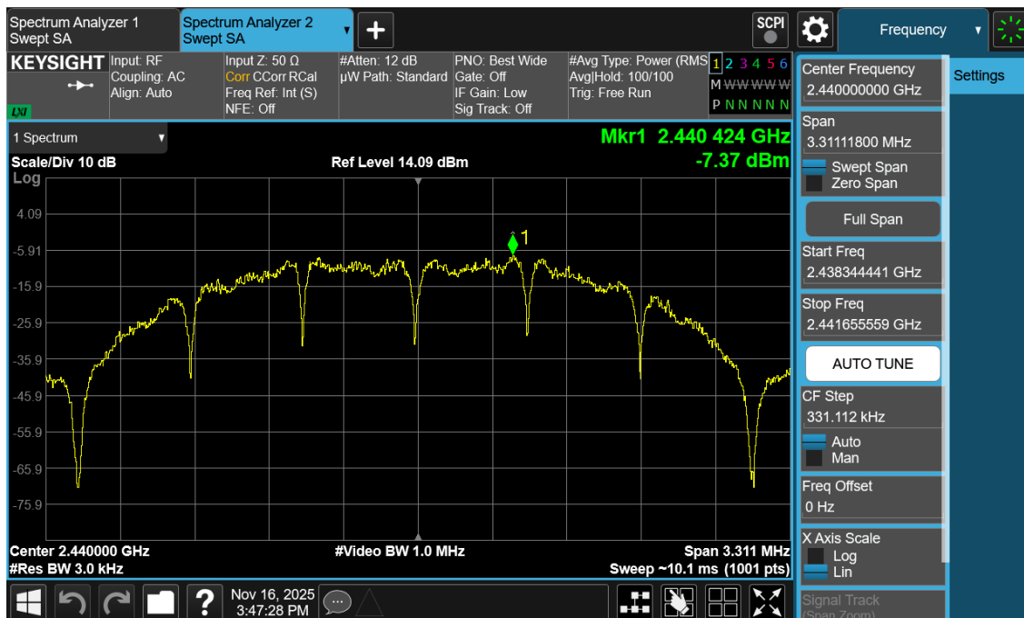
Plot 7-17. Power Spectral Density Antenna 3a (802.15.4, iPA – Ch. 18)
