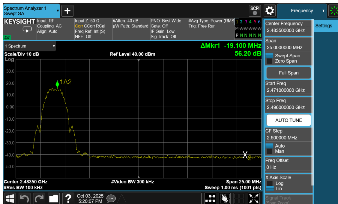
Plot 7-28. Band Edge Antenna 1a (802.15.4, ePA – Ch. 25)
