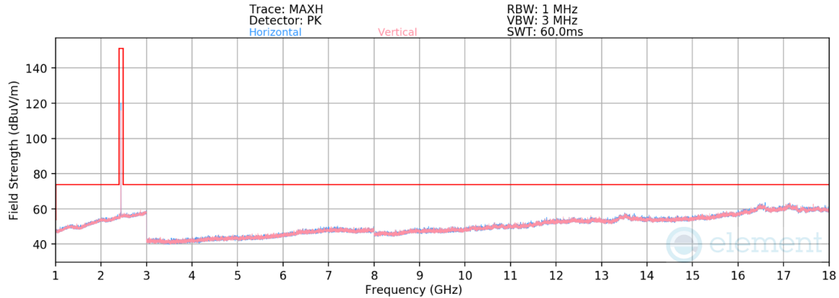
Plot 7-42. Radiated Spurious Emissions 1-18GHz Antenna 3a (802.15.4 ePA – Ch. 18)
