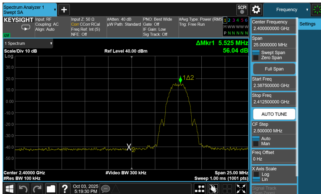
Plot 7-27. Band Edge Antenna 1a (802.15.4, ePA – Ch. 11)
