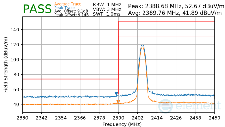
Plot 7-49. Radiated Restricted Lower Band Edge Measurement Antenna 3a
