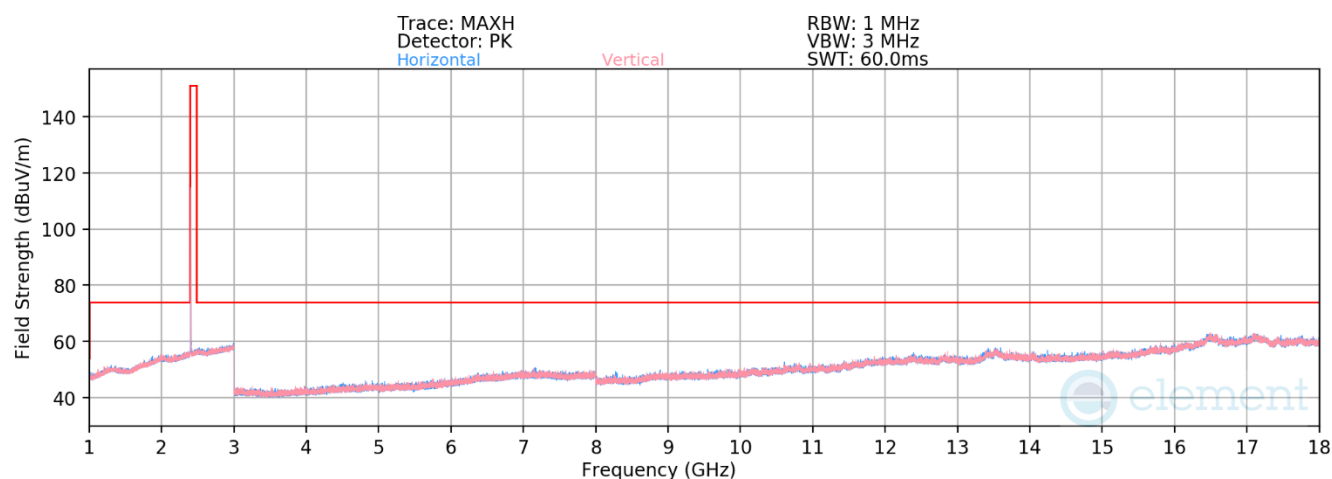
Plot 7-41. Radiated Spurious Emissions 1-18GHz Antenna 3a (802.15.4 ePA – Ch. 11)
