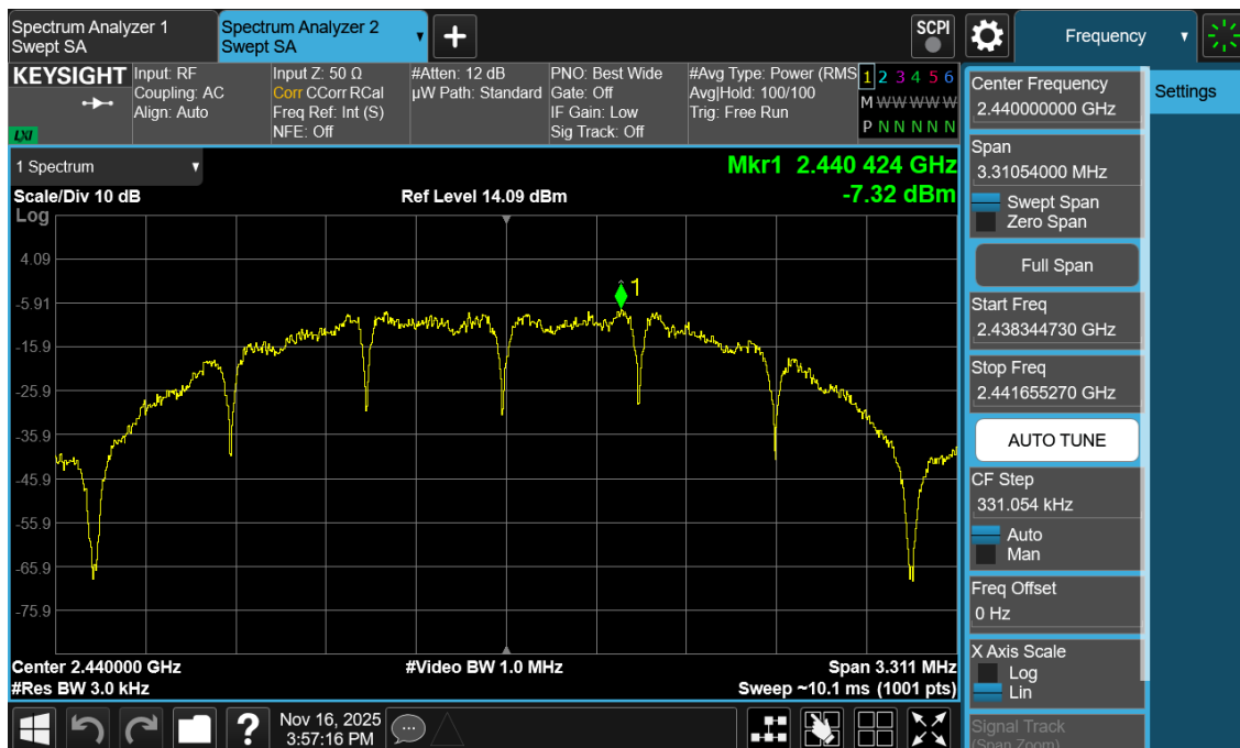
Plot 7-23. Power Spectral Density Antenna 1a (802.15.4, iPA – Ch. 18)
