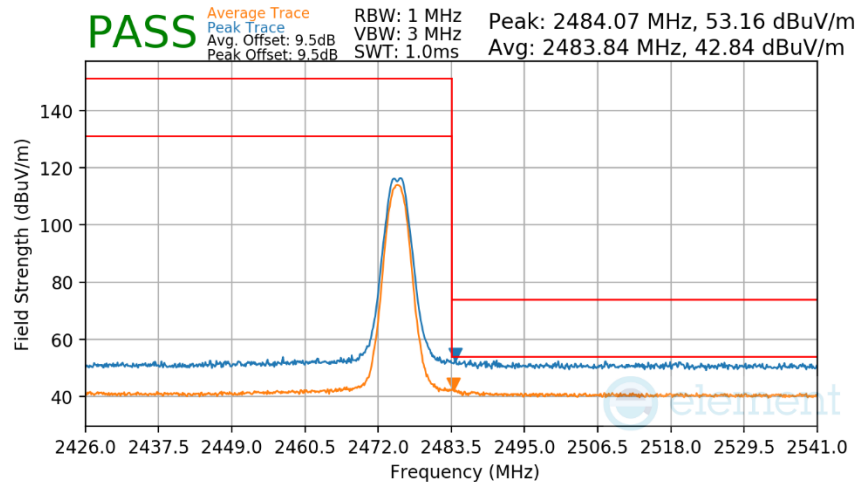
Plot 7-52. Radiated Restricted Upper Band Edge Measurement Antenna 1a
