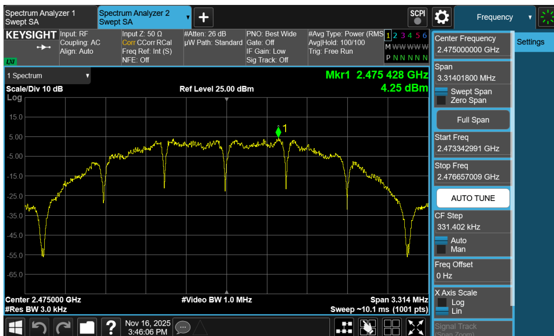
Plot 7-15. Power Spectral Density Antenna 3a (802.15.4, ePA – Ch. 25)
