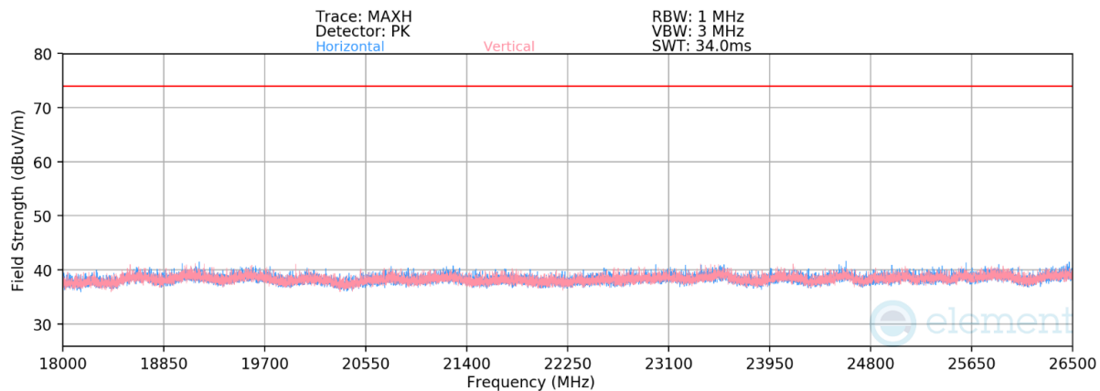
Plot 7-47. Radiated Spurious Emissions Above 18GHz Antenna 1a (802.15.4 ePA – Ch. 18)
