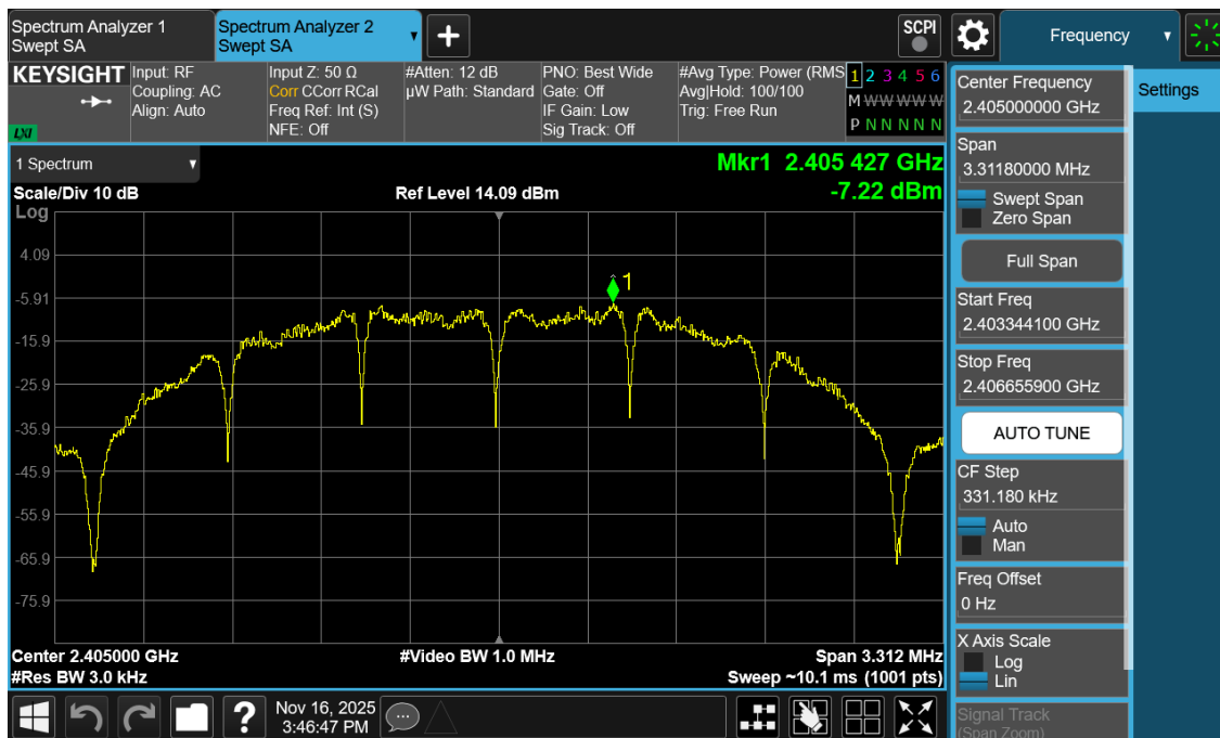
Plot 7-16. Power Spectral Density Antenna 3a (802.15.4, iPA – Ch. 11)
