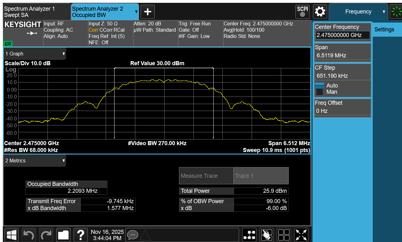
Plot 7-3. 99% OBW Antenna 3a (802.15.4, Ch. 25)
