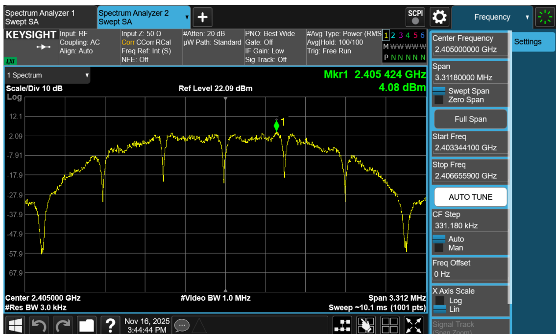
Plot 7-13. Power Spectral Density Antenna 3a (802.15.4, ePA – Ch. 11)
