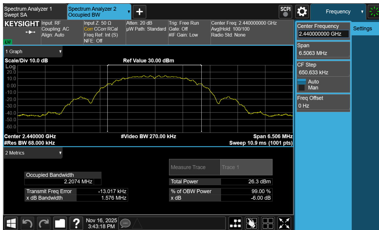
Plot 7-2. 99% OBW Antenna 3a (802.15.4, Ch. 18)
