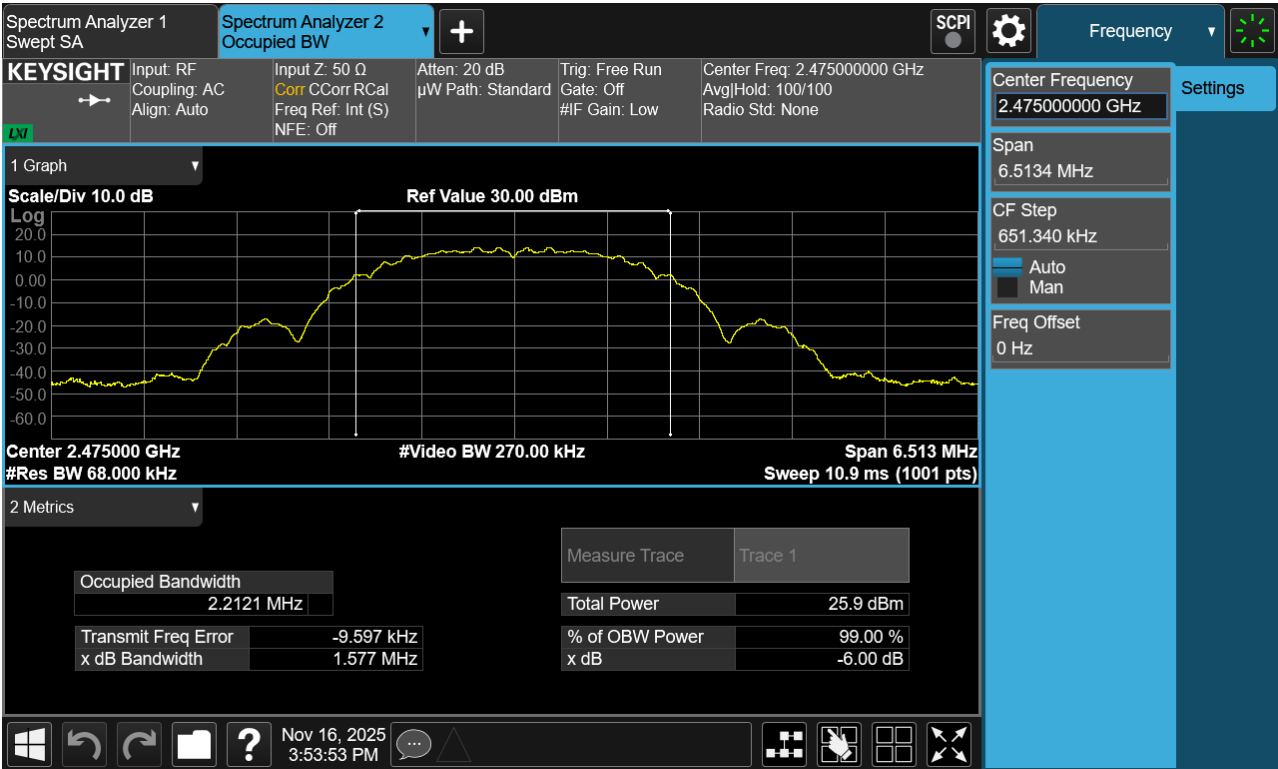
Plot 7-6. 99% OBW Antenna 1a(802.15.4, Ch. 25)
