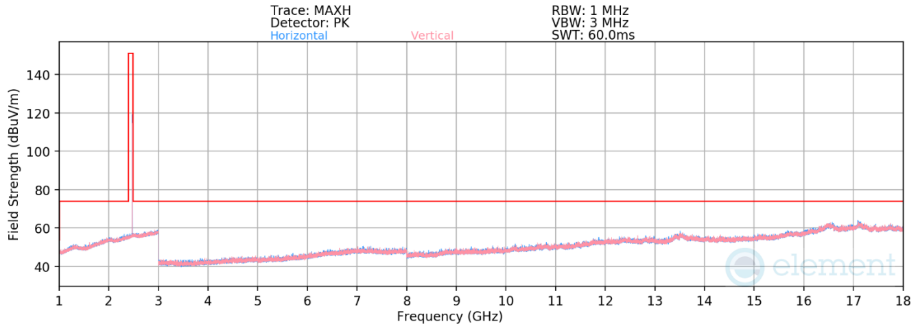
Plot 7-44. Radiated Spurious Emissions 1-18GHz Antenna 3a (802.15.4 ePA – Ch. 25)
