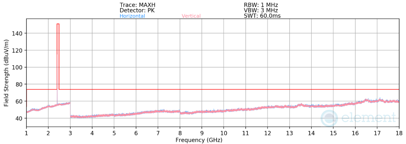
Plot 7-45. Radiated Spurious Emissions 1-18GHz Antenna 1a (802.15.4 ePA – Ch. 11)
