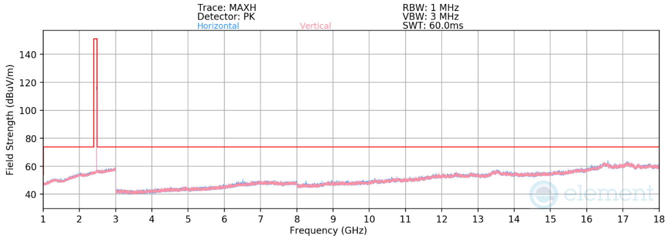
Plot 7-48. Radiated Spurious Emissions 1-18GHz Antenna 1a (802.15.4 ePA – Ch. 25)
