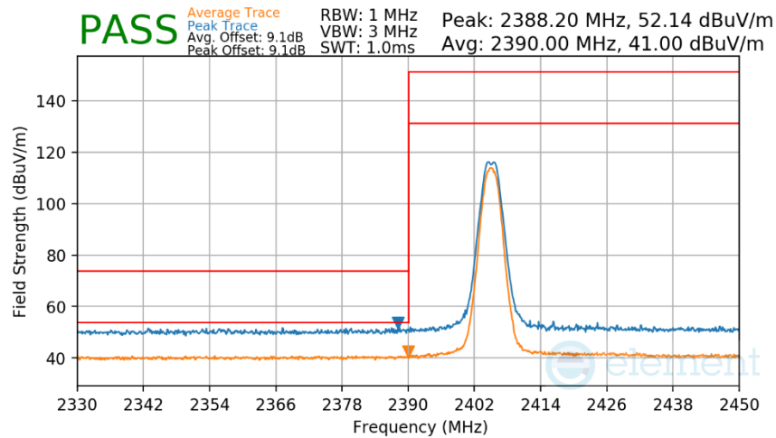
Plot 7-51. Radiated Restricted Lower Band Edge Measurement Antenna 1a
