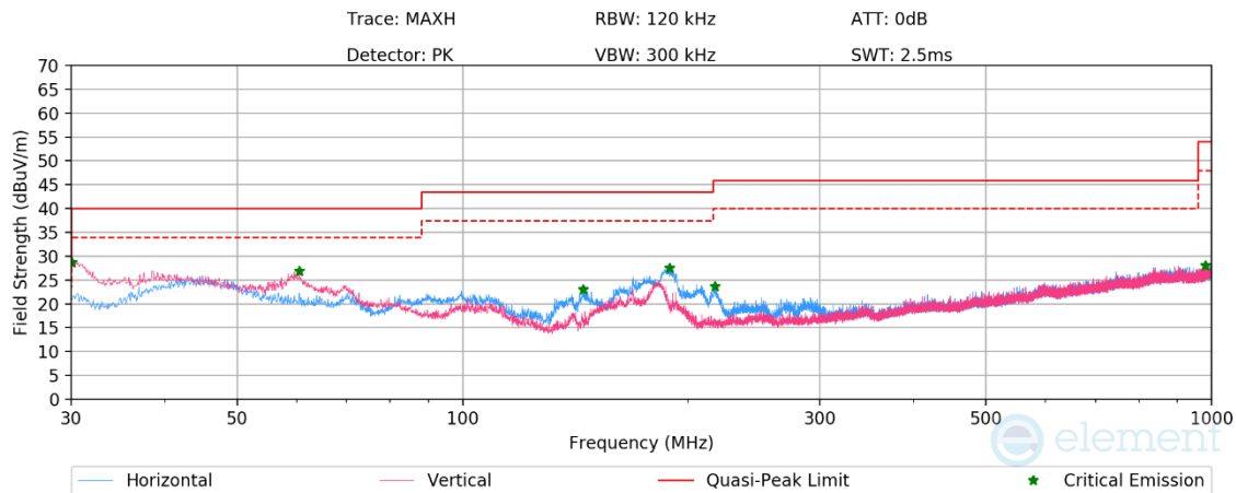
Plot 7-53. Radiated Spurious Emissions 30MHz-1GHz Antenna 3a (ePA - Ch.18, with AC/DC Adapter)
