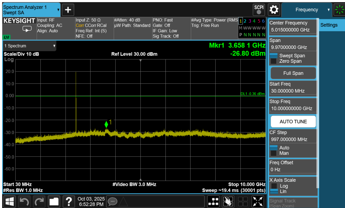
Plot 7-31. Conducted Spurious Antenna 3a (802.15.4, ePA – Ch. 18)
