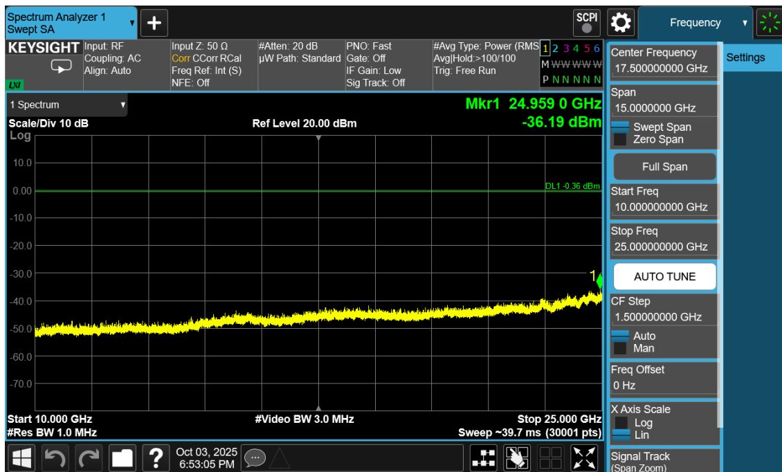
Plot 7-32. Conducted Spurious Antenna 3a (802.15.4, ePA – Ch. 18)
