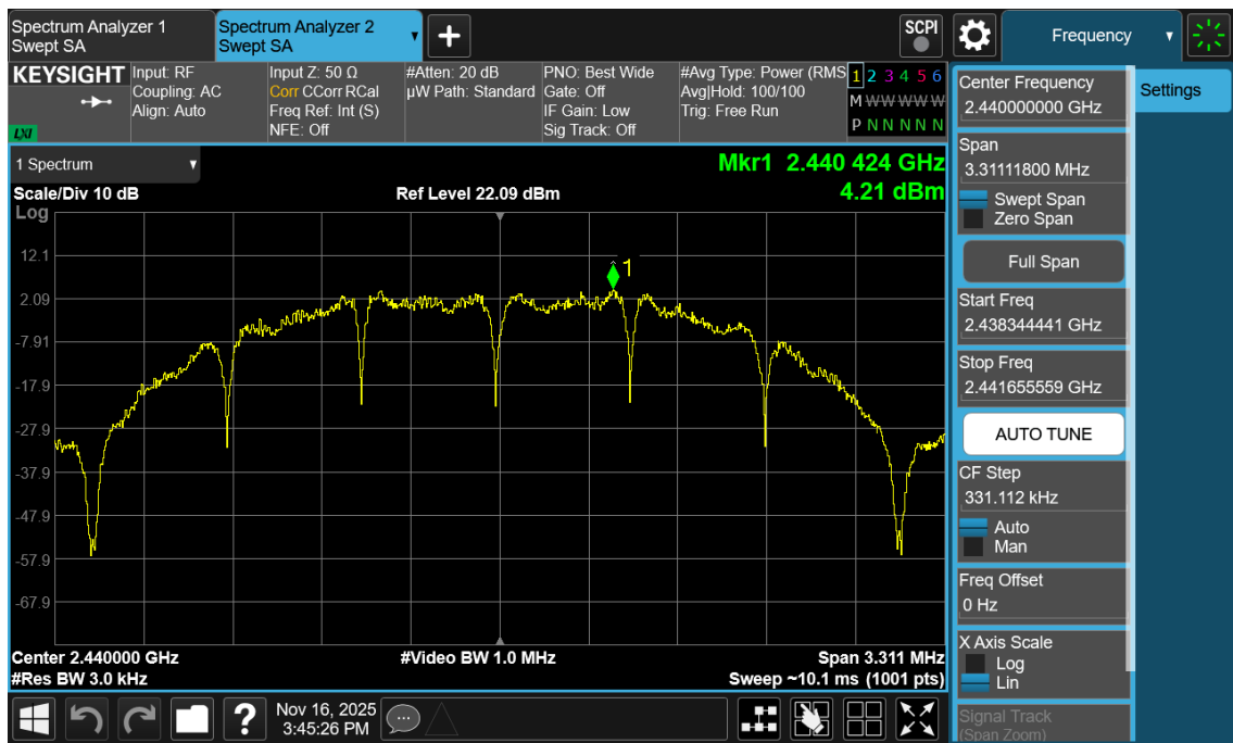
Plot 7-14. Power Spectral Density Antenna 3a (802.15.4, ePA – Ch. 18)
