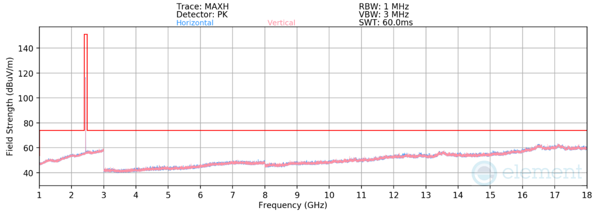
Plot 7-46. Radiated Spurious Emissions 1-18GHz Antenna 1a (802.15.4 ePA – Ch. 18)
