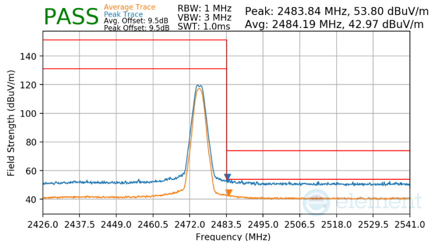
Plot 7-50. Radiated Restricted Upper Band Edge Measurement Antenna 3a
