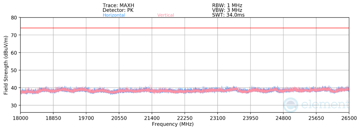
Plot 7-43. Radiated Spurious Emissions Above 18GHz Antenna 3a (802.15.4 ePA – Ch. 18)
