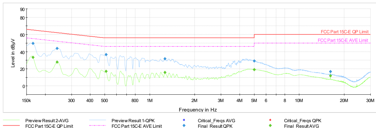
Plot 7-54. AC Line Conducted Emission with 802.15.4 Antenna 3a (L1, Ch.18 - ePA, with AC/DC Adapter)
