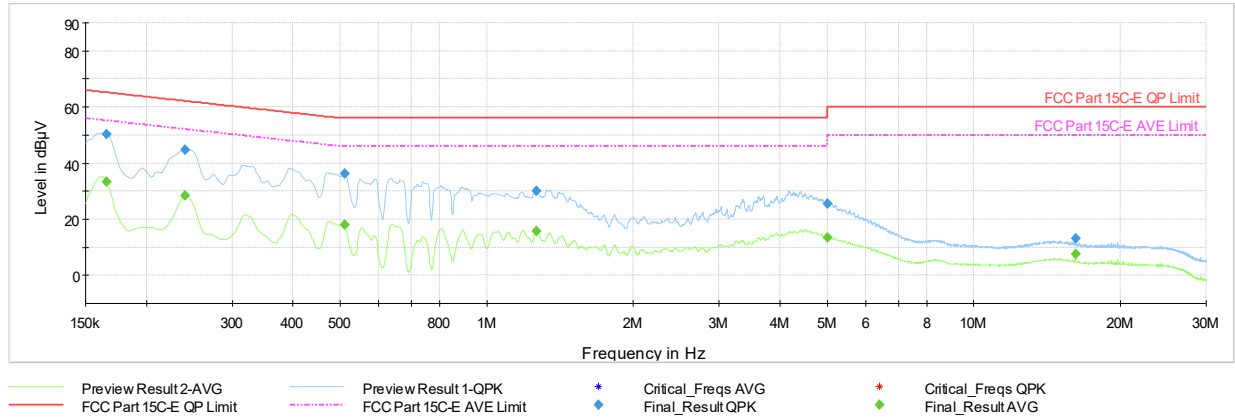
Plot 7-55. AC Line Conducted Emission with 802.15.4 Antenna 3a (N, Ch.18 - ePA, with AC/DC Adapter)
