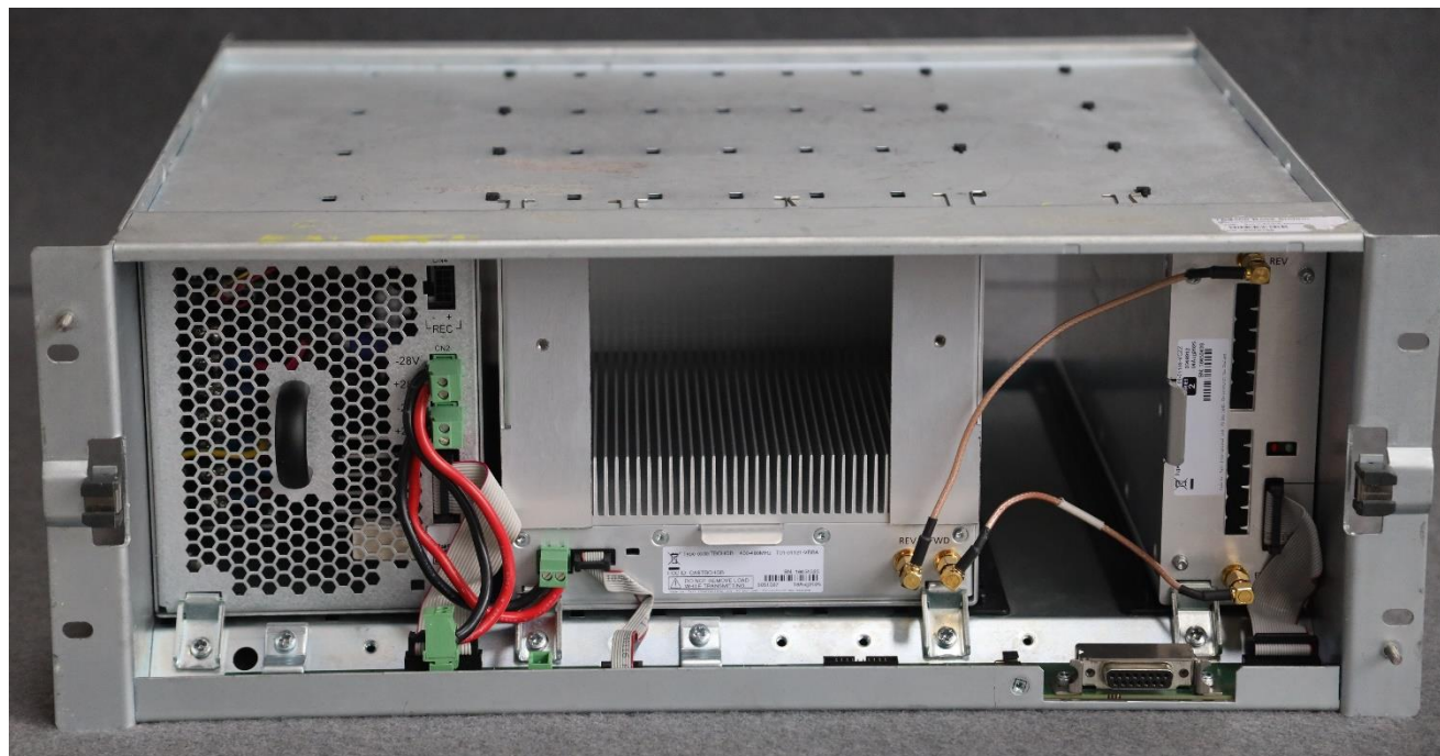
Photograph 07: Base station – Front view -- Open
