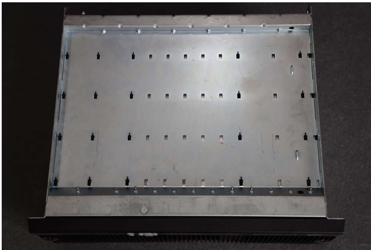
Photograph 06: Base station – Bottom Side view
