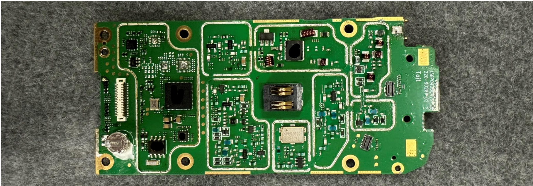
Photograph 02: Receive-Transmit PCB - top (without shields)
