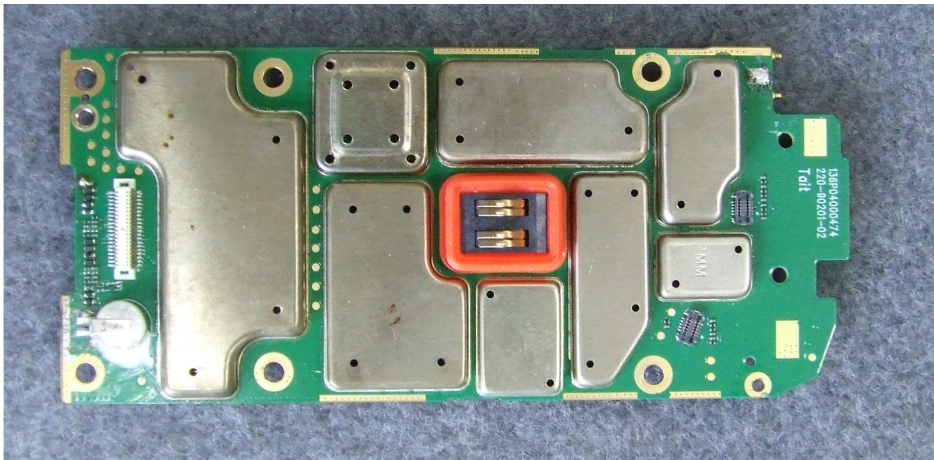
Photograph 01: Receive-Transmit PCB – top (with shields)
