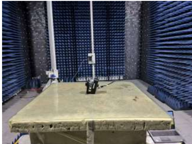
RE (Above 1GHz)
