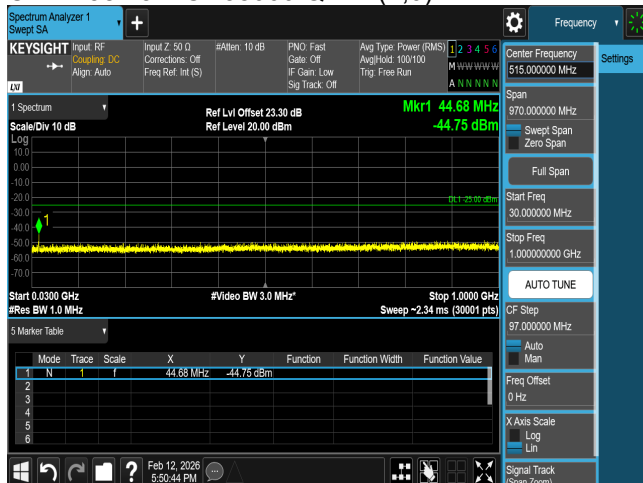
CSE B38 15M CH38175 QPSK(1,0)
