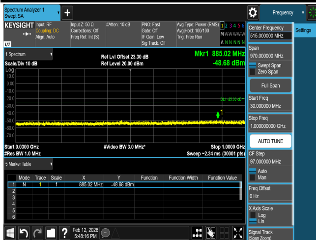
CSE B38 15M CH37825 QPSK(1,0)
