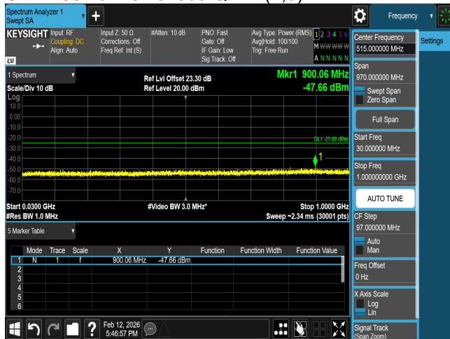
CSE B38 10M CH38000 QPSK(1,0)
