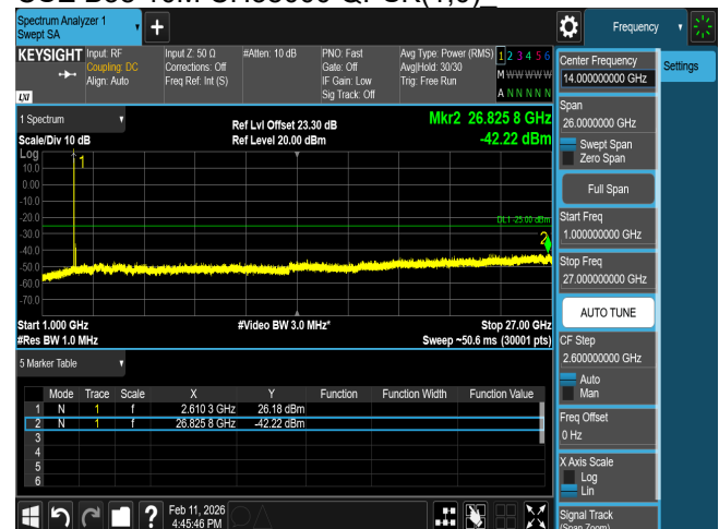
CSE B38 10M CH38200 QPSK(1,0)_
