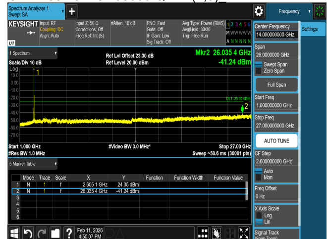
CSE B38 15M CH38175 QPSK(1,0)_
