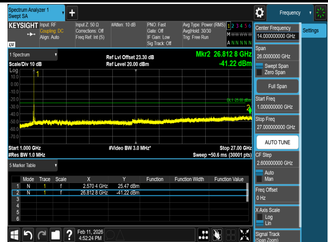
CSE B38 20M CH37850 QPSK(1,0)
