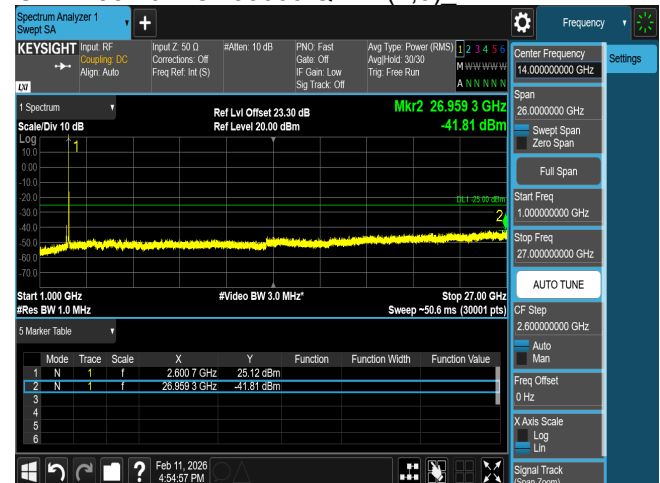
CSE B38 20M CH38000 QPSK(1,0)
