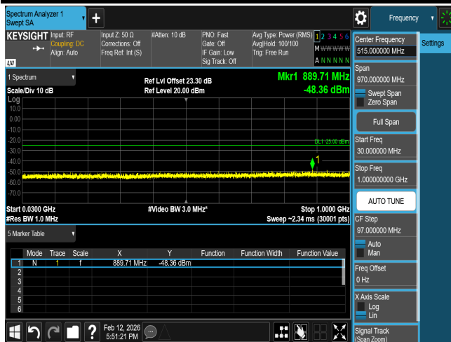
CSE B38 20M CH37850 QPSK(1,0)
