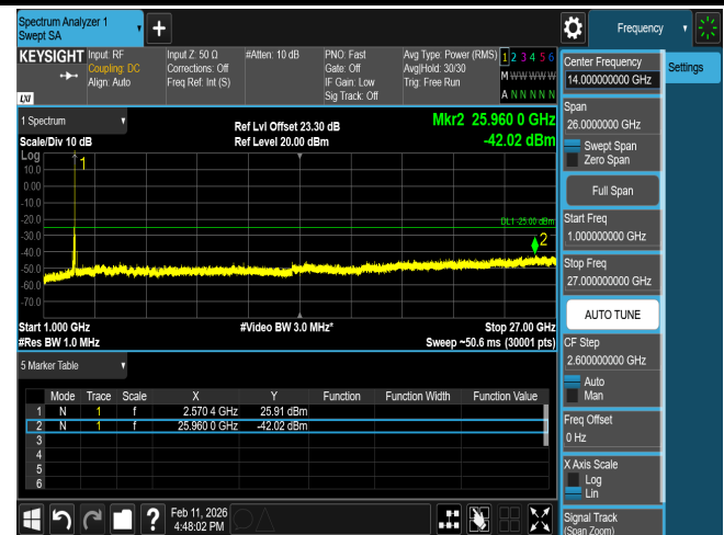
CSE B38 15M CH37825 QPSK(1,0)
