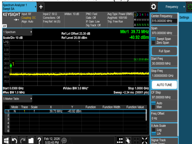
CSE B38 20M CH38000 QPSK(1,0)
