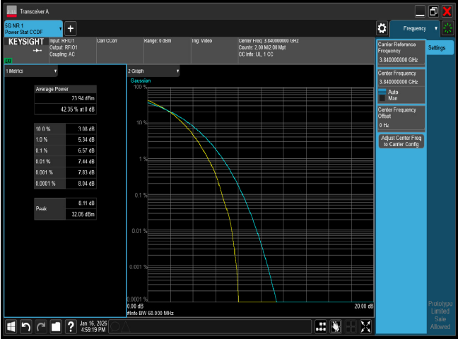
PTAR B77 60M CH656000 64QAM
