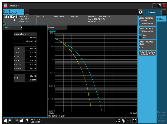
PTAR B77 90M CH656000 256QAM
