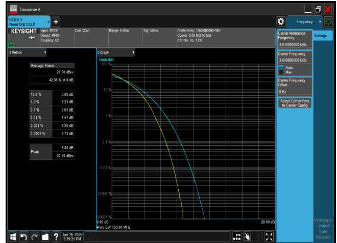
PTAR B77 100M CH656000 256QAM
