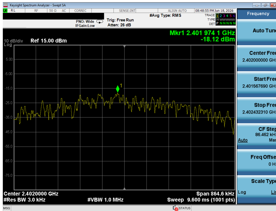
Plot 7-10. Power Spectral Density Plot (ANT – Ch. 1)
