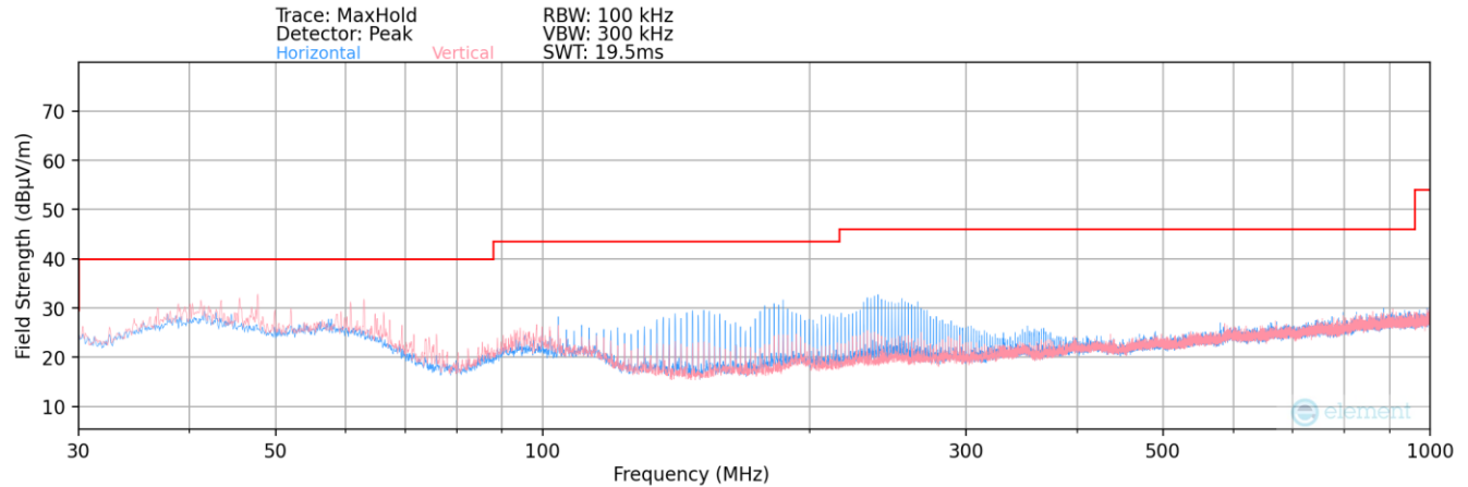
Plot 7-27. Radiated Spurious Plot below 1GHz
