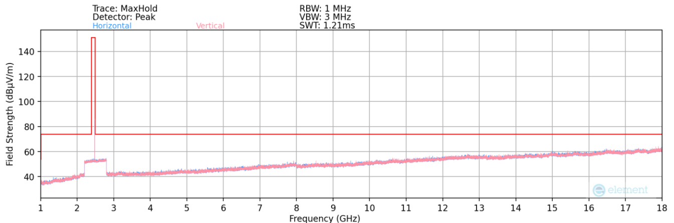
Plot 7-23. Radiated Spurious Plot above 1GHz (ANT – Ch. 79)
