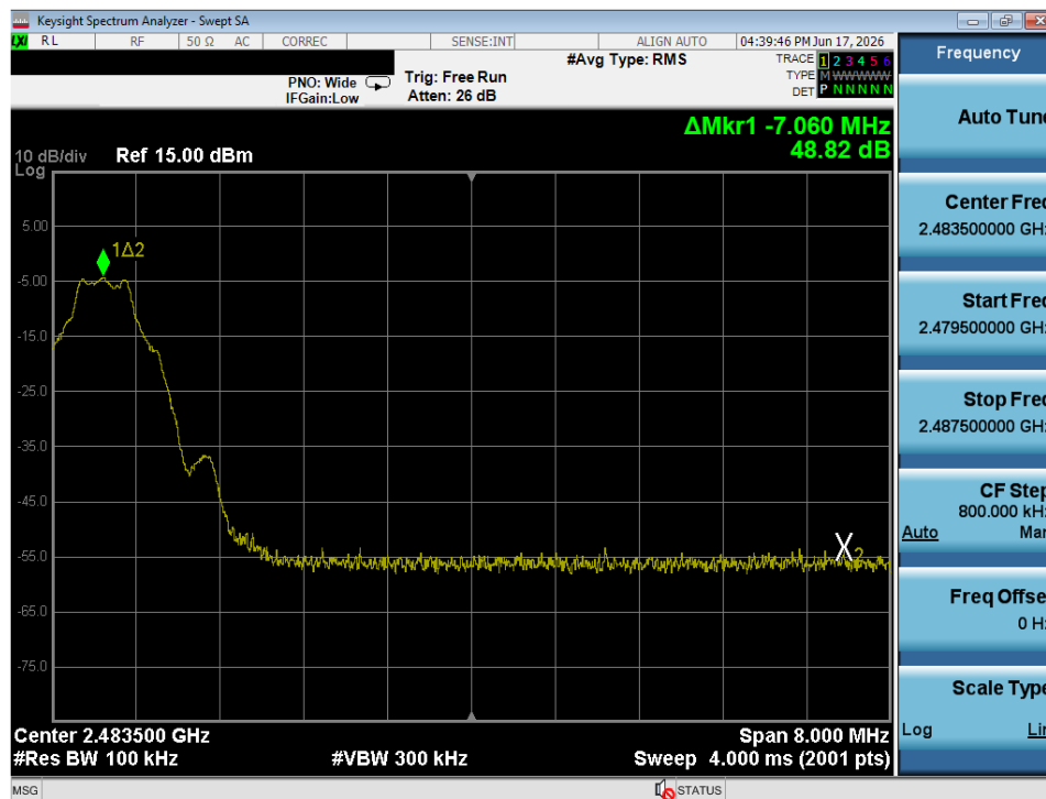
Plot 7-14. Band Edge Plot (ANT – Ch. 79)
