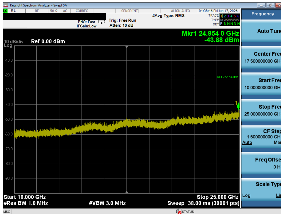
Plot 7-18. Conducted Spurious Plot (ANT - Ch. 39)
