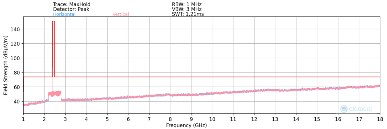
Plot 7-21. Radiated Spurious Plot above 1GHz (ANT – Ch. 1)
