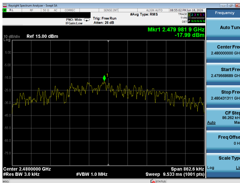
Plot 7-12. Power Spectral Density Plot (ANT – Ch. 79)
