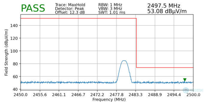
Plot 7-26. Radiated Restricted Upper Band Edge Measurement (Peak)
