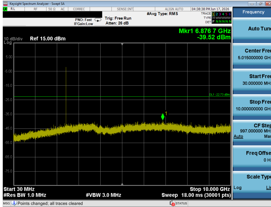
Plot 7-17. Conducted Spurious Plot (ANT - Ch. 39)
