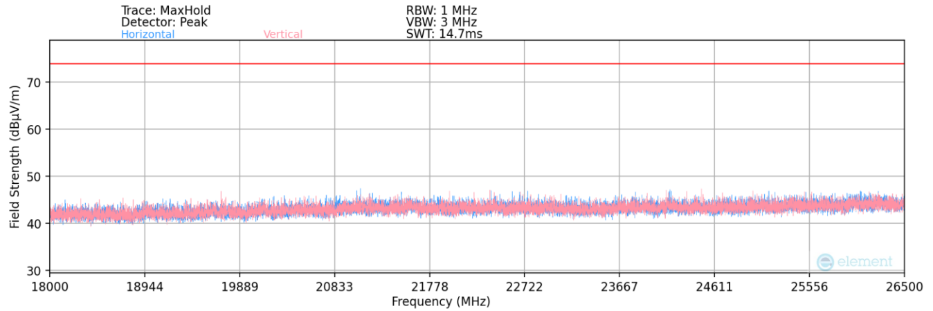
Plot 7-24. Radiated Spurious Plot above 18GHz (ANT – Ch. 39)
