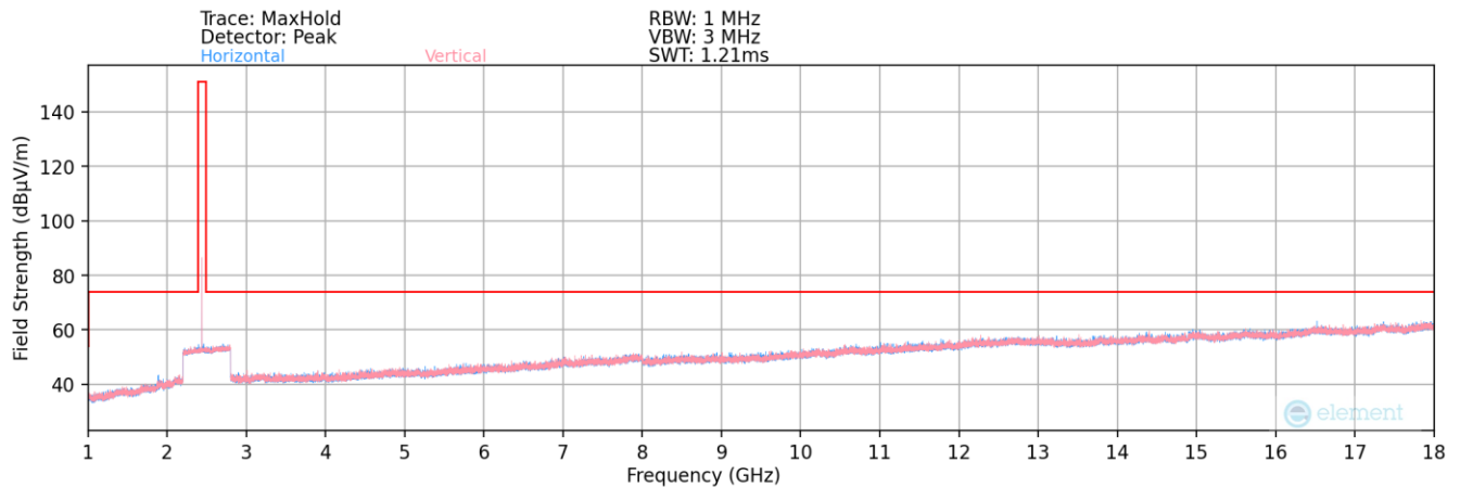
Plot 7-22. Radiated Spurious Plot above 1GHz (ANT – Ch. 39)
