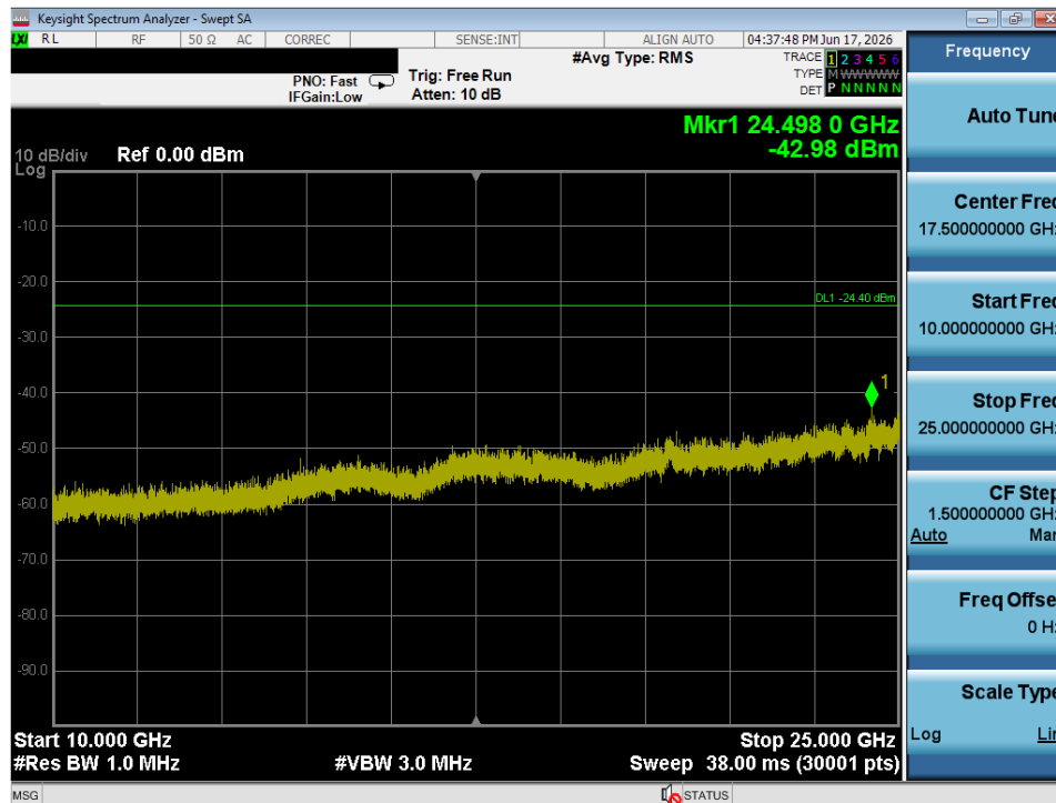
Plot 7-16. Conducted Spurious Plot (ANT – Ch. 1)
