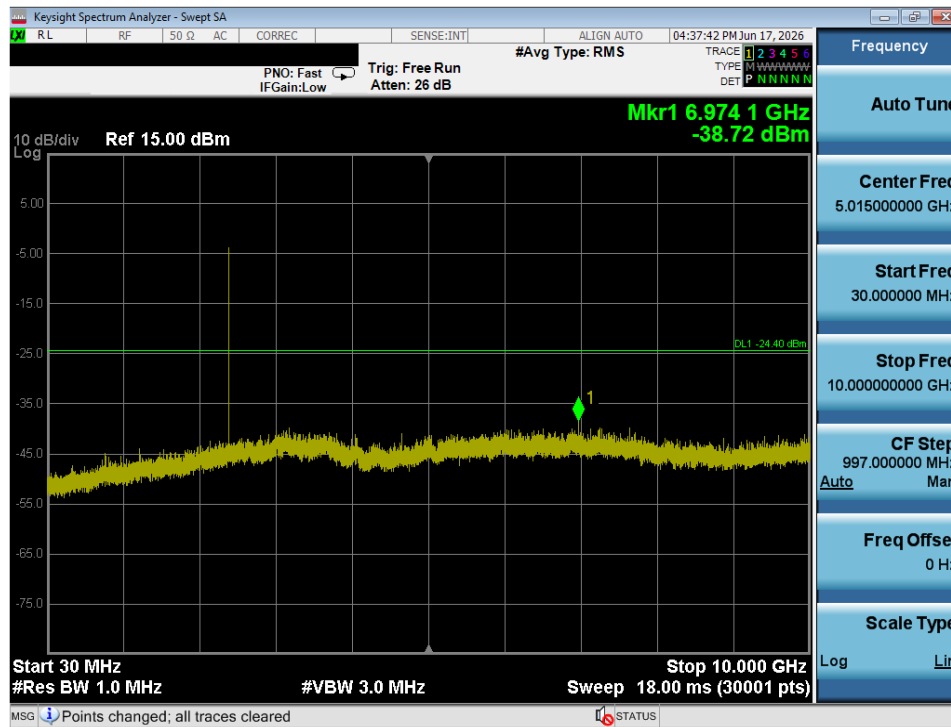
Plot 7-15. Conducted Spurious Plot (ANT – Ch. 1)
