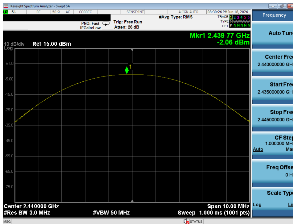
Plot 7-8. Peak Power Plot (ANT – Ch. 39)
