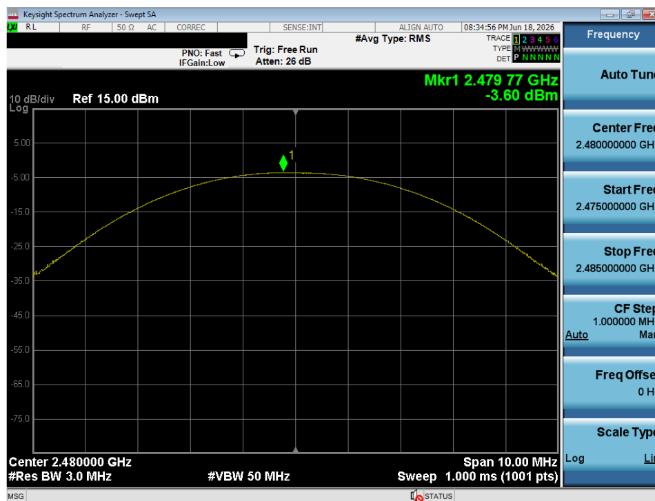
Plot 7-9. Peak Power Plot (ANT – Ch. 79)
