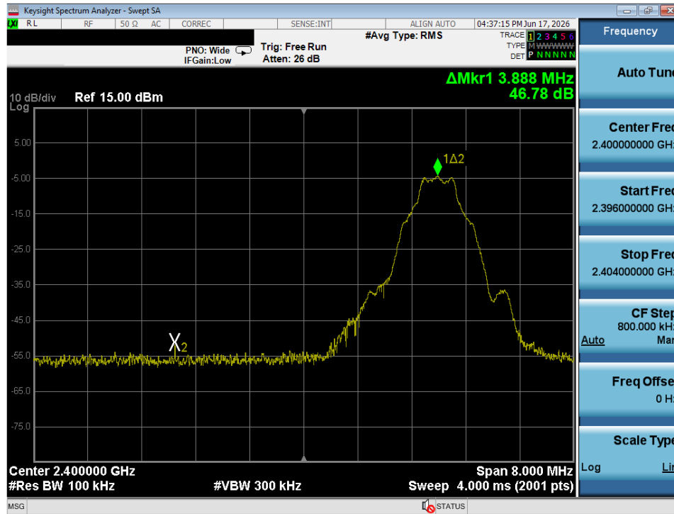
Plot 7-13. Band Edge Plot (ANT – Ch. 1)
