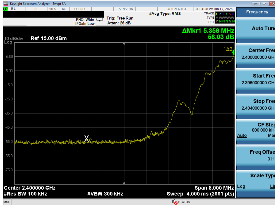
Plot 7-27. Band Edge Plot (Bluetooth (LE), 2Mbps – Ch. 0)
