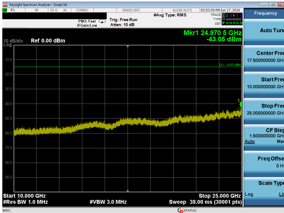
Plot 7-30. Conducted Spurious Plot (Bluetooth (LE), 1Mbps – Ch. 37)
