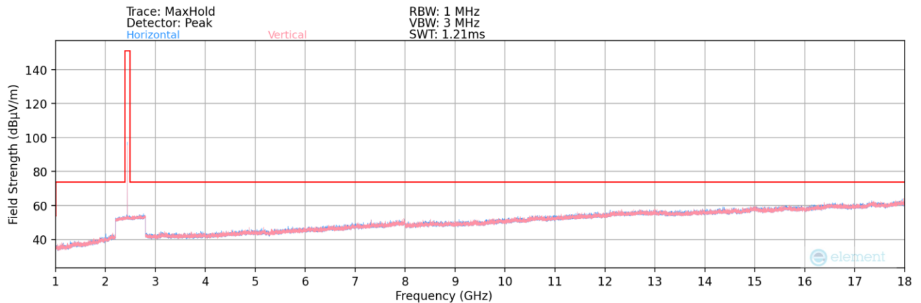
Plot 7-36. Radiated Spurious Plot above 1GHz (Bluetooth (LE) – Ch. 17)
