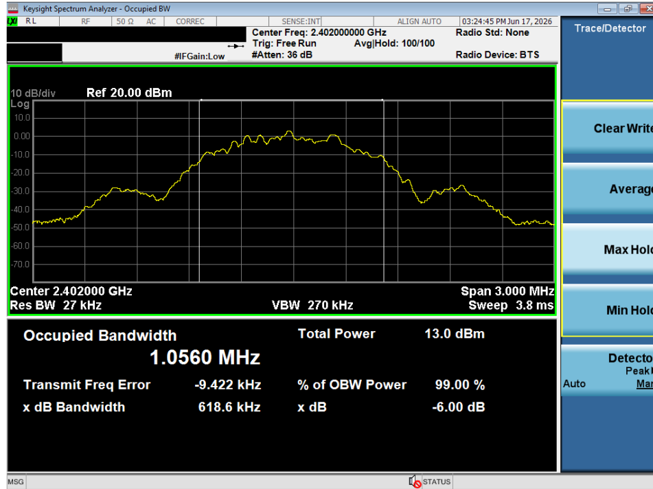
Plot 7-7. OBW Plot (Bluetooth (LE), 1Mbps – Ch. 37)
