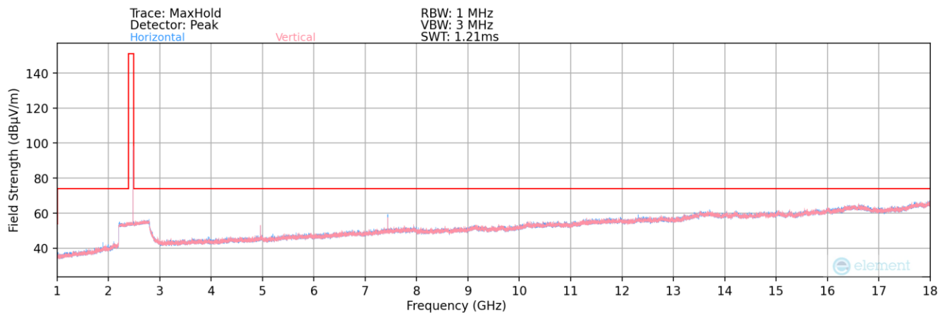
Plot 7-37. Radiated Spurious Plot above 1GHz (Bluetooth (LE) – Ch. 39)
