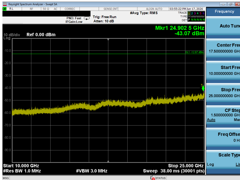
Plot 7-32. Conducted Spurious Plot (Bluetooth (LE), 1Mbps – Ch. 17)
