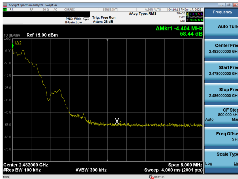
Plot 7-28. Band Edge Plot (Bluetooth (LE), 2Mbps – Ch. 36)
