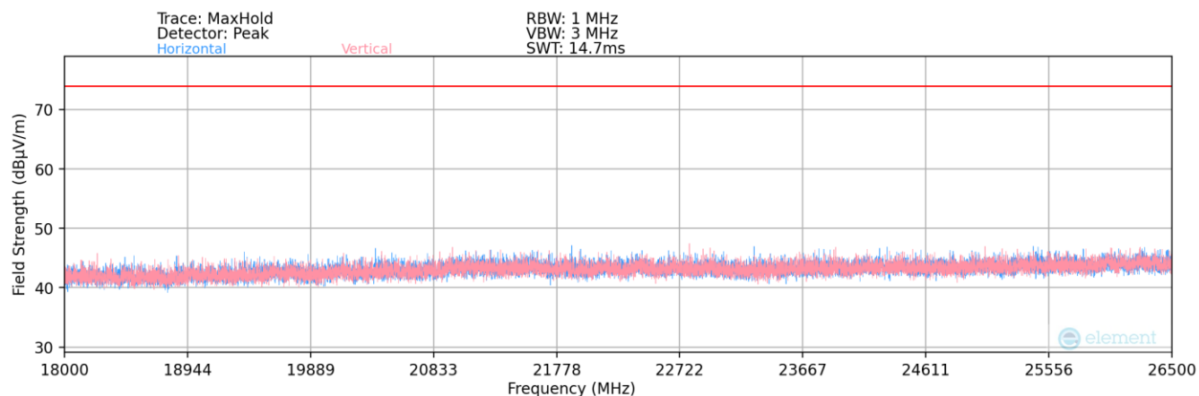
Plot 7-38. Radiated Spurious Plot above 18GHz (Bluetooth (LE))
