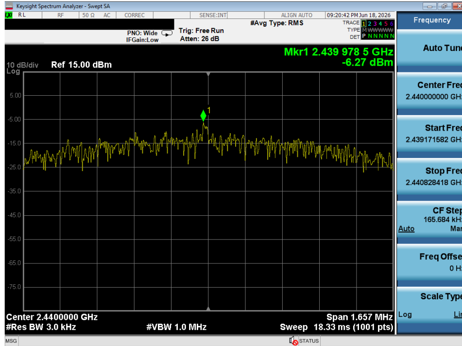
Plot 7-23. Power Spectral Density Plot (Bluetooth (LE), 2Mbps – Ch. 17)
