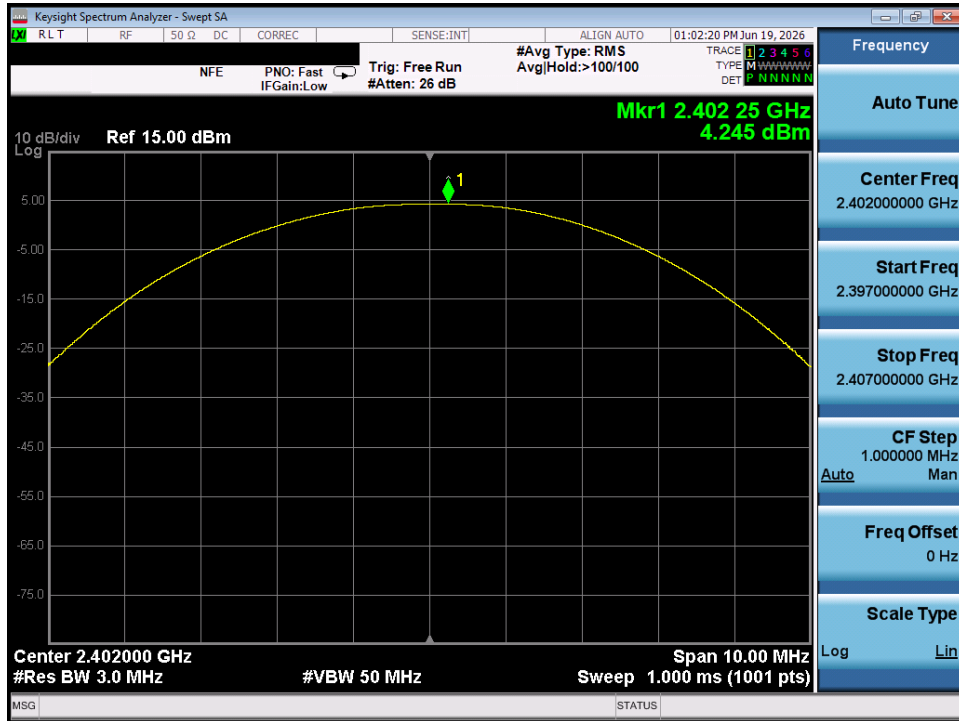
Plot 7-13. Peak Power Plot (Bluetooth (LE), 1Mbps – Ch. 37)
