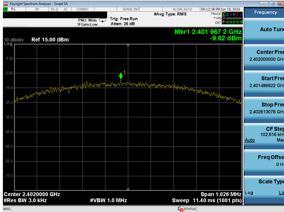
Plot 7-19. Power Spectral Density Plot (Bluetooth (LE), 1Mbps – Ch. 37)
