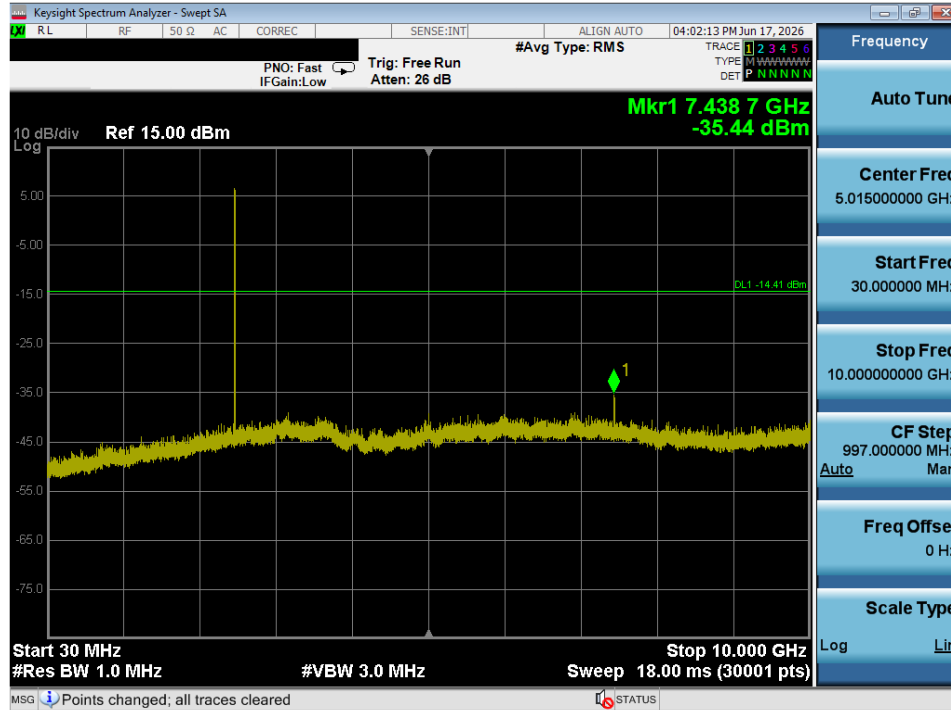
Plot 7-33. Conducted Spurious Plot (Bluetooth (LE), 1Mbps – Ch. 39)
