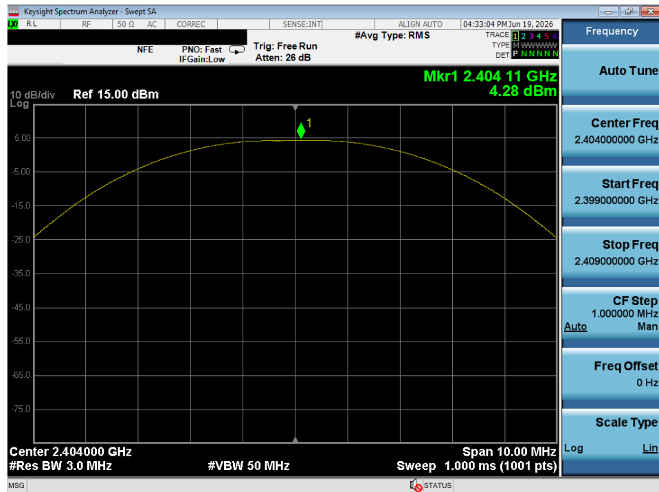
Plot 7-16. Peak Power Plot (Bluetooth (LE), 2Mbps – Ch. 0)
