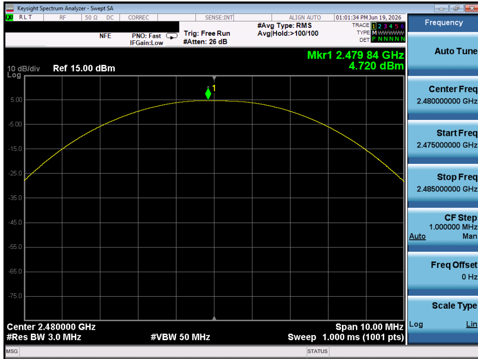
Plot 7-15. Peak Power Plot (Bluetooth (LE), 1Mbps – Ch. 39)
