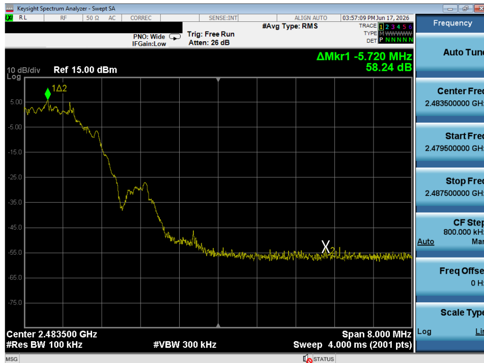
Plot 7-26. Band Edge Plot (Bluetooth (LE), 1Mbps – Ch. 39)
