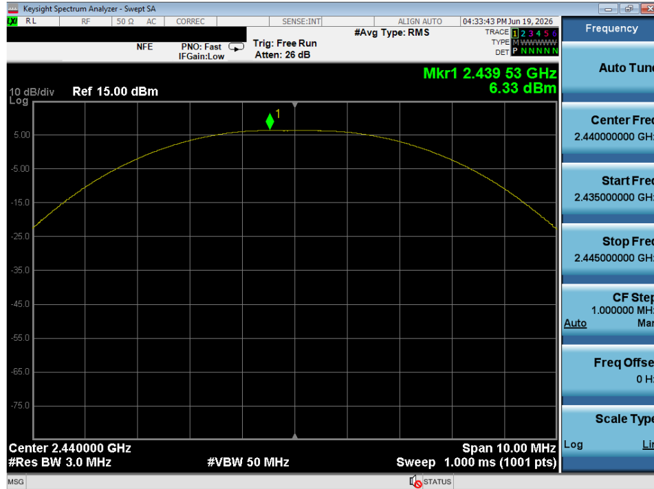
Plot 7-17. Peak Power Plot (Bluetooth (LE), 2Mbps – Ch. 17)
