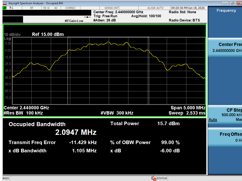
Plot 7-5. 6dB Bandwidth Plot (Bluetooth (LE), 2Mbps – Ch. 17)
