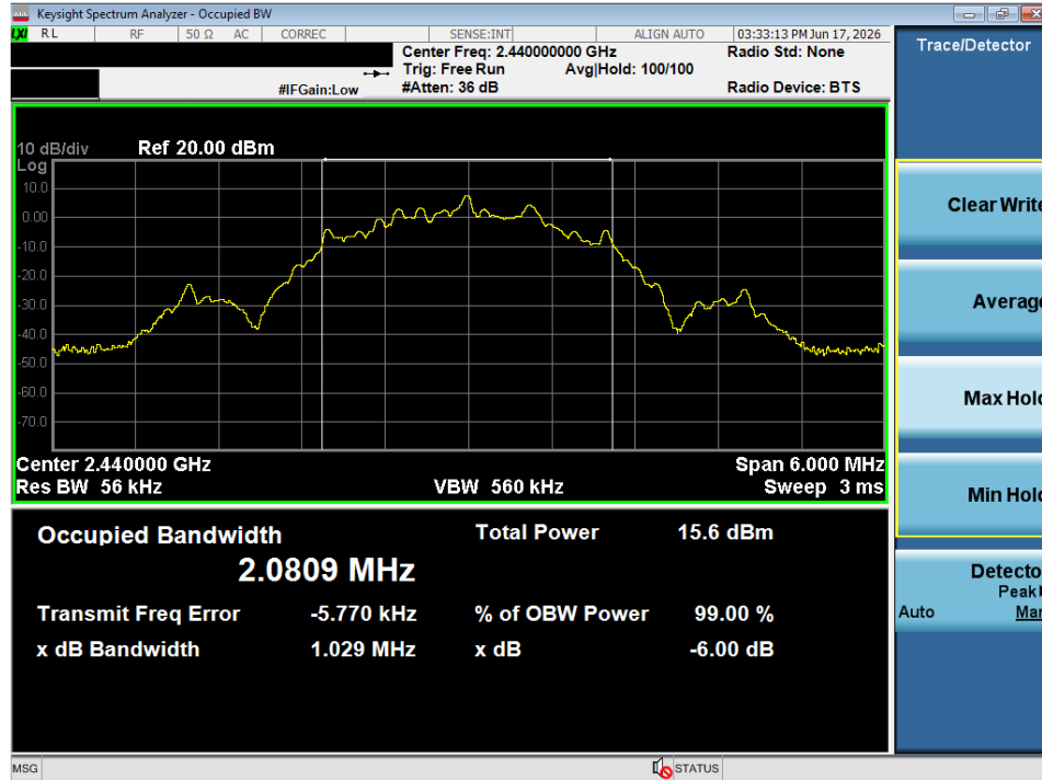
Plot 7-11. OBW Plot (Bluetooth (LE), 2Mbps – Ch. 17)
