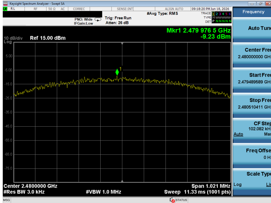
Plot 7-21. Power Spectral Density Plot (Bluetooth (LE), 1Mbps – Ch. 39)
