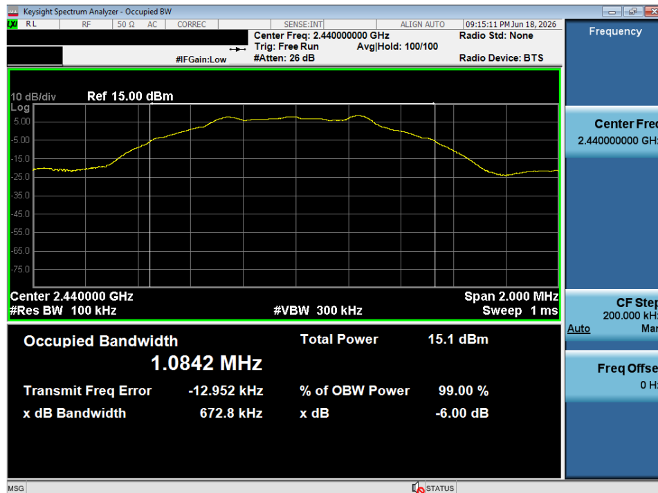
Plot 7-2. 6dB Bandwidth Plot (Bluetooth (LE), 1Mbps – Ch. 17)
