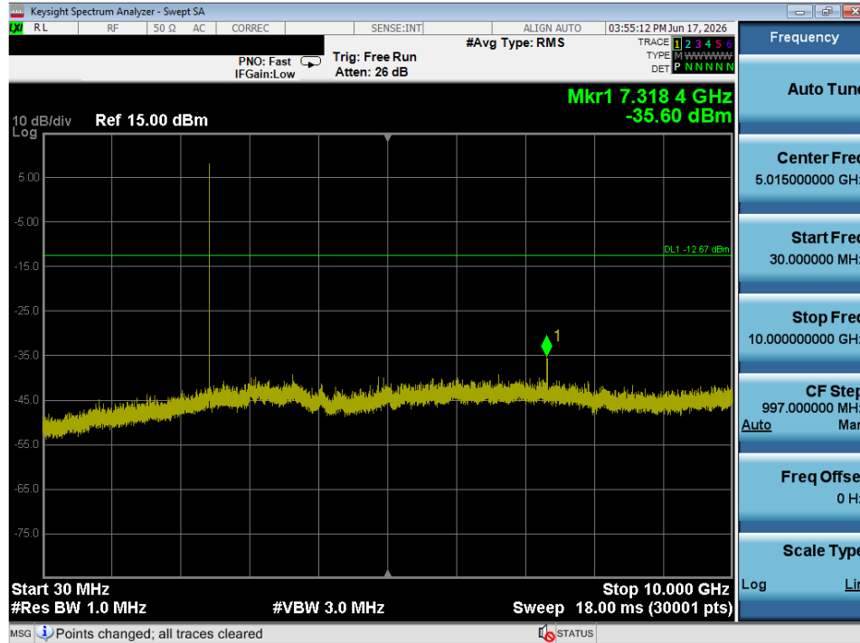
Plot 7-31. Conducted Spurious Plot (Bluetooth (LE), 1Mbps – Ch. 17)
