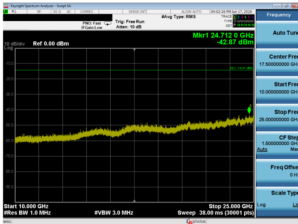
Plot 7-34. Conducted Spurious Plot (Bluetooth (LE), 1Mbps – Ch. 39)
