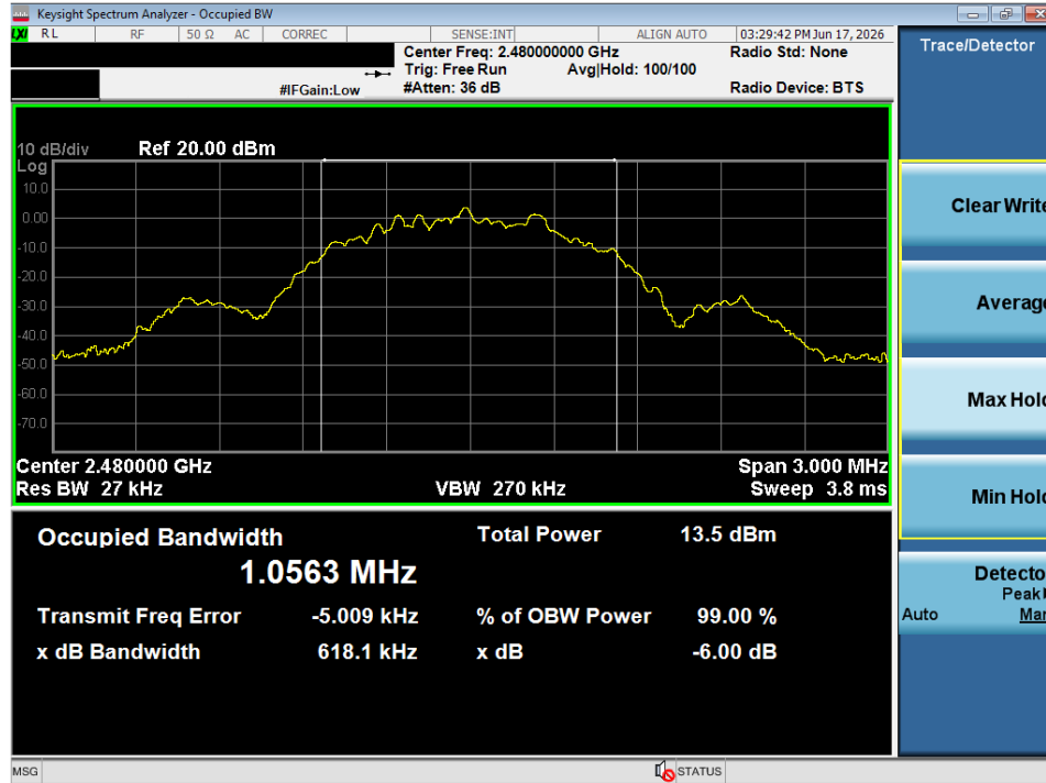
Plot 7-9. OBW Plot (Bluetooth (LE), 1Mbps – Ch. 39)
