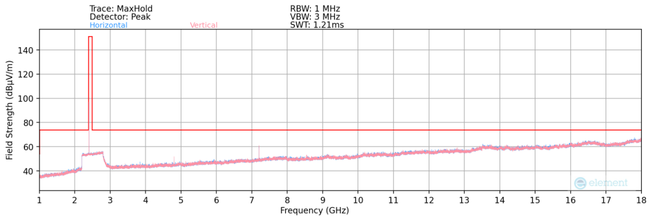
Plot 7-35. Radiated Spurious Plot above 1GHz (Bluetooth (LE) – Ch. 37)
