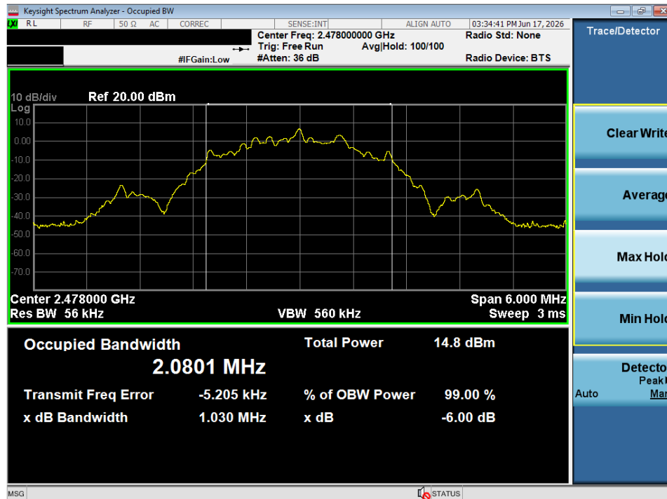
Plot 7-12. OBW Plot (Bluetooth (LE), 2Mbps – Ch. 36)
