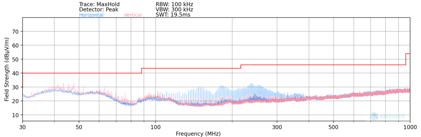
Plot 7-43. Radiated Spurious Plot below 1GHz
