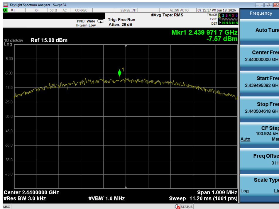
Plot 7-20. Power Spectral Density Plot (Bluetooth (LE), 1Mbps – Ch. 17)
