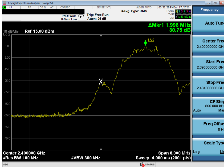
Plot 7-25. Band Edge Plot (Bluetooth (LE), 1Mbps – Ch. 37)
