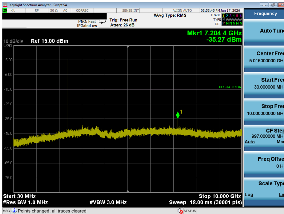
Plot 7-29. Conducted Spurious Plot (Bluetooth (LE), 1Mbps – Ch. 37)
