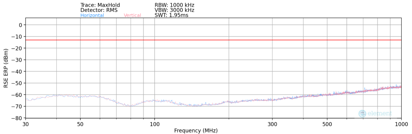
Plot 7-25. Radiated Spurious Plot below 1GHz LTE CAT-M1 Band 4 + Bluetooth
