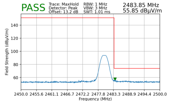
Plot 7-40. Radiated Restricted Upper Band Edge Measurement (Peak)
