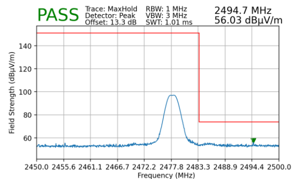
Plot 7-38. Radiated Restricted Upper Band Edge Measurement (Peak)
