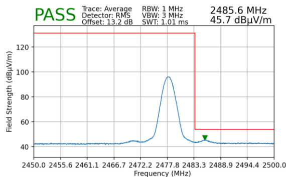
Plot 7-37. Radiated Restricted Upper Band Edge Measurement (Average)
