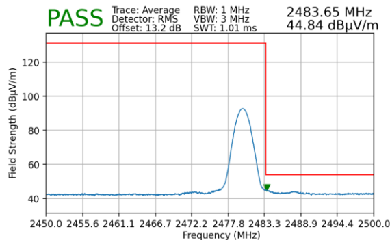
Plot 7-39. Radiated Restricted Upper Band Edge Measurement (Average)
