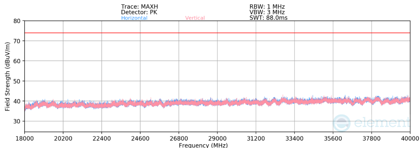
Plot 7-37. Radiated Spurious Emissions above 18GHz (BT GFSK – Ch. 78)
