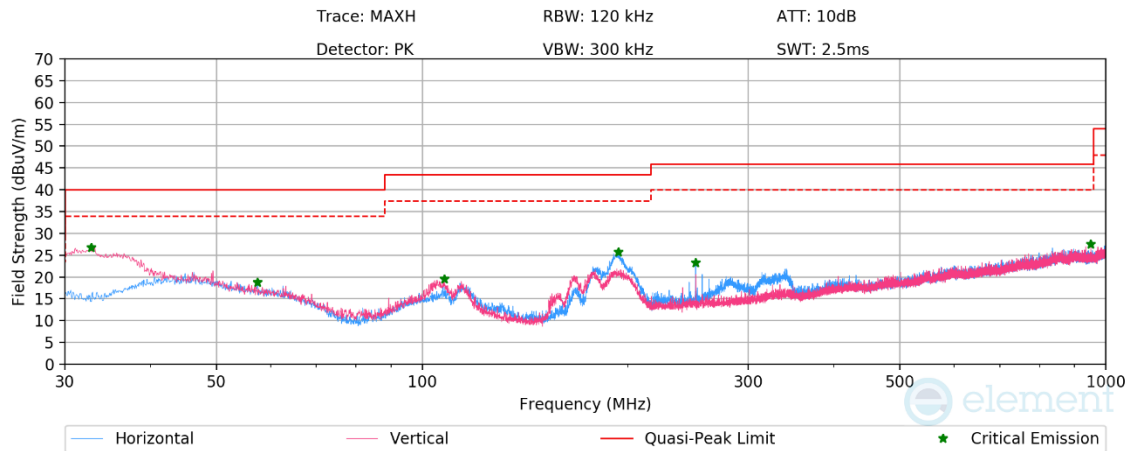
Plot 7-46. Radiated Spurious Emissions Below 1GHz (GFSK – Ch.78, with AC/DC Adapter)
