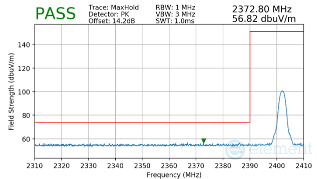
Plot 7-41. Radiated Restricted Lower Band Edge Measurement (Peak)
