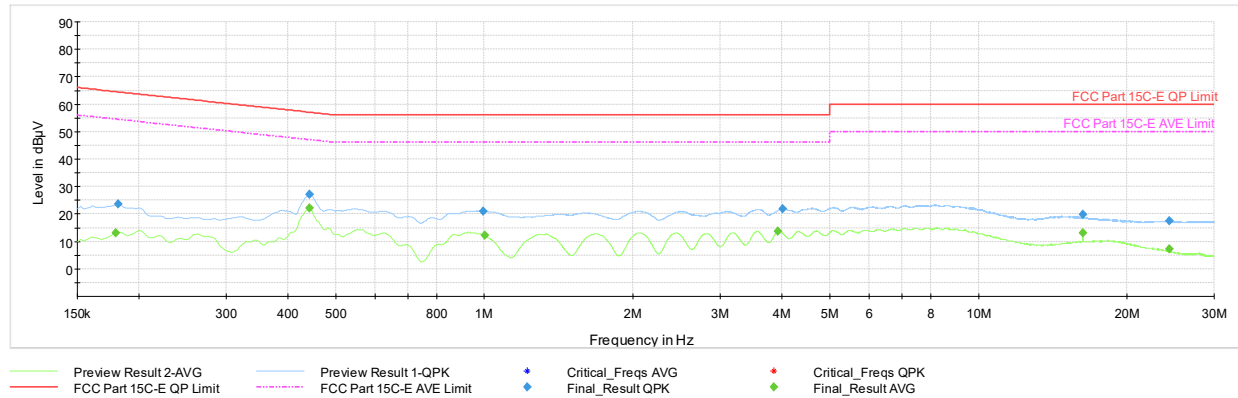
Plot 7-47. AC Line-Conducted Test Plot (L1, GFSK – Ch.39, with AC/DC Adapter)
