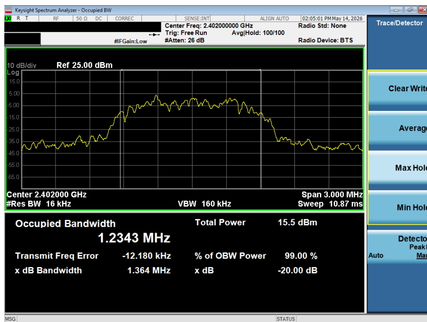
Plot 9-1. 20dB Bandwidth Plot (Spot-check)
