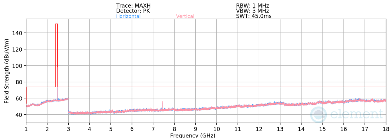
Plot 7-36. Radiated Spurious Emissions above 1GHz (BT GFSK – Ch. 78)
