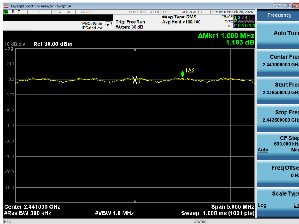
Plot 7-17. Channel Spacing Plot (Bluetooth, \pi/4 -DQPSK)
