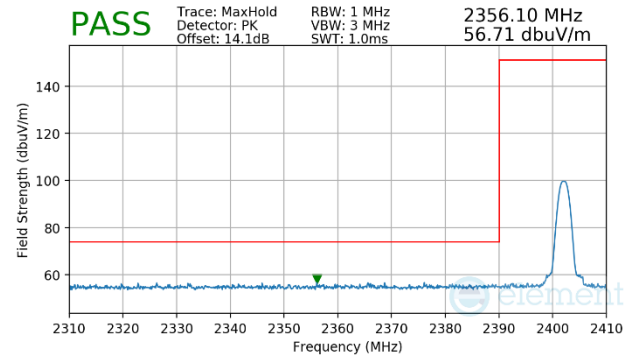
Plot 7-39. Radiated Restricted Lower Band Edge Measurement (Peak)
