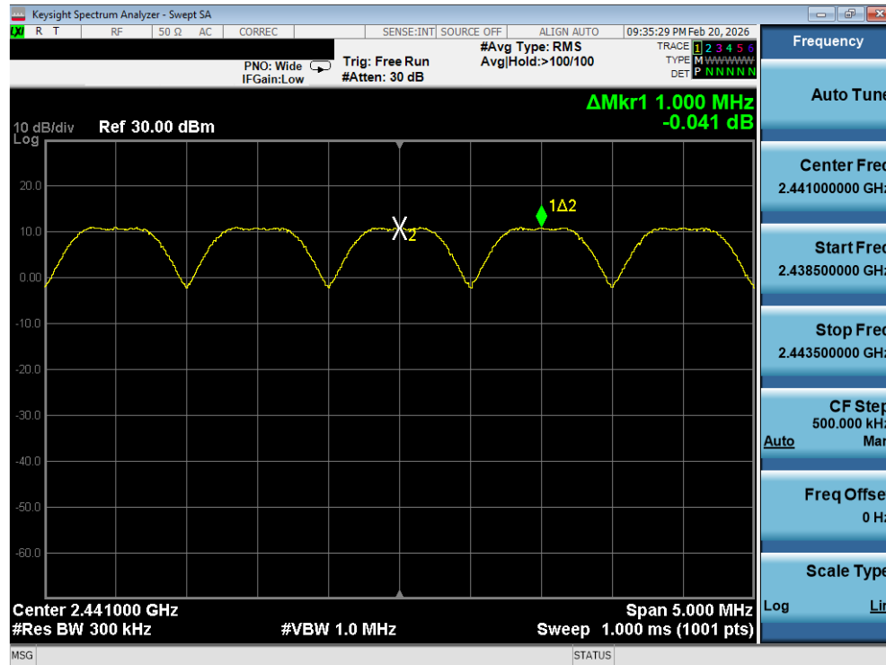
Plot 7-16. Channel Spacing Plot (Bluetooth, GFSK)
