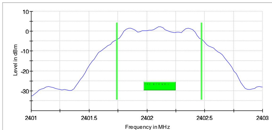
6 dB Bandwidth
