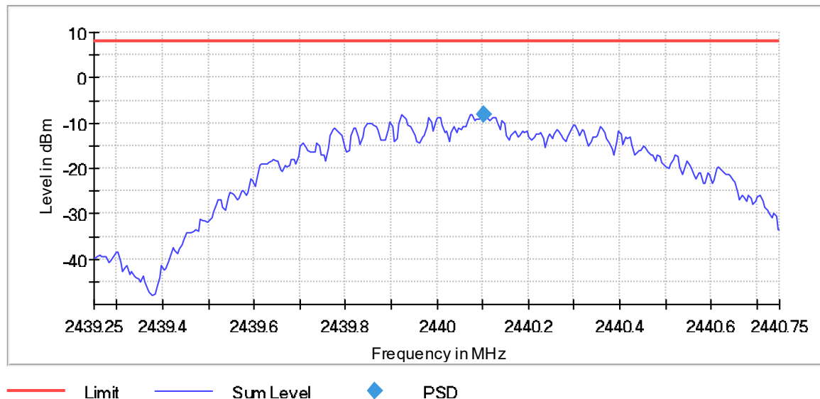
Power Spectral Density (AVG PSD-3)
