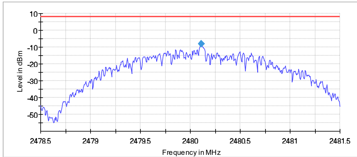
Power Spectral Density (AVG PSD-3)
