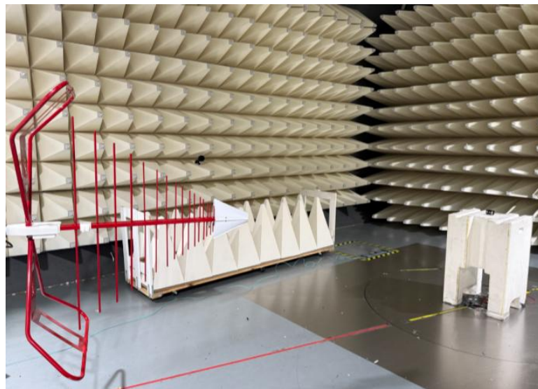
Figure B2: Radiated Low range Setup 30 – 1 GHz
