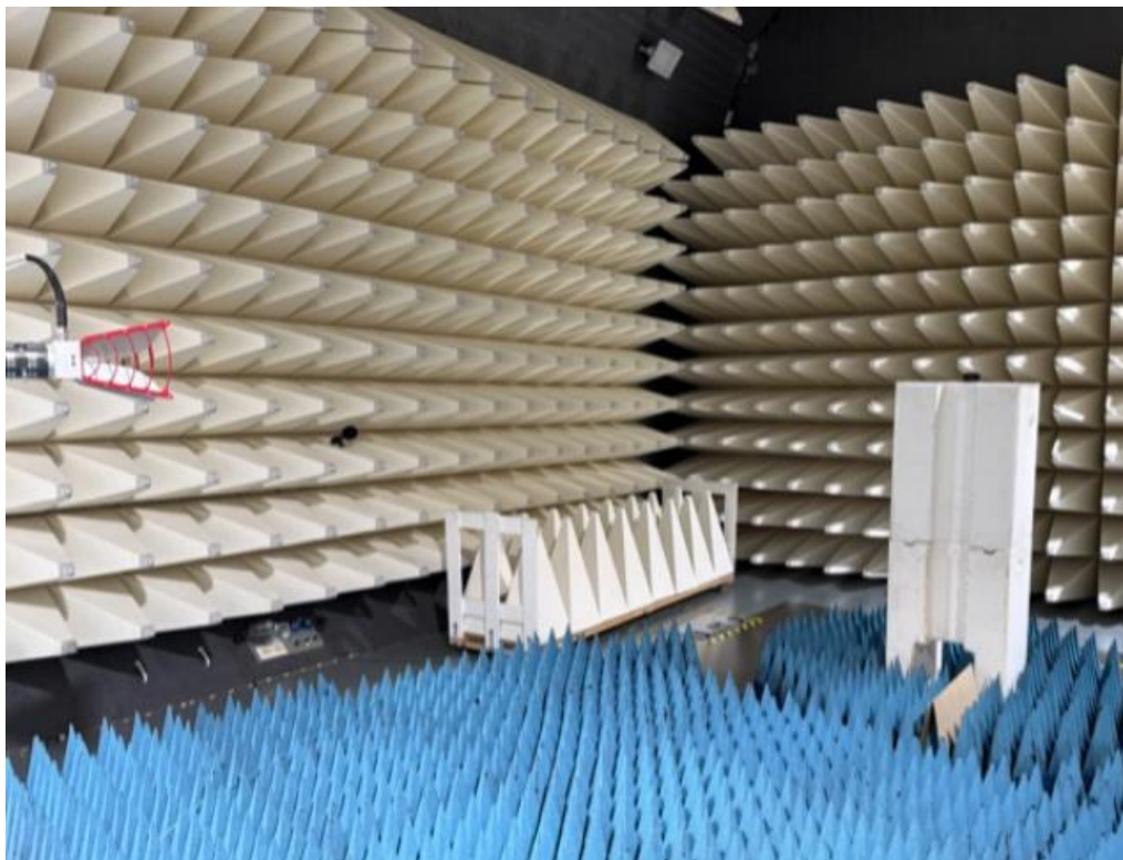
Figure B3: Radiated High range Setup 1 GHz – 18 GHz
