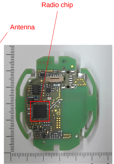
Visualisation board, bottom view *
