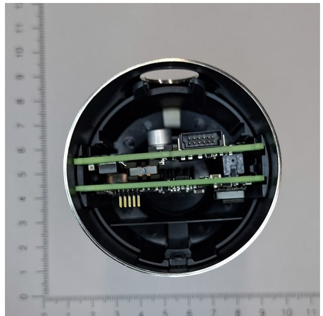
Mainboard and sensor board in housing *
