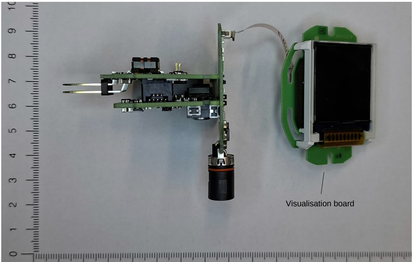
All PCBs connected *
