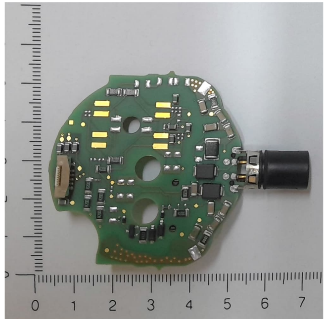
Terminal board - bottom view *
