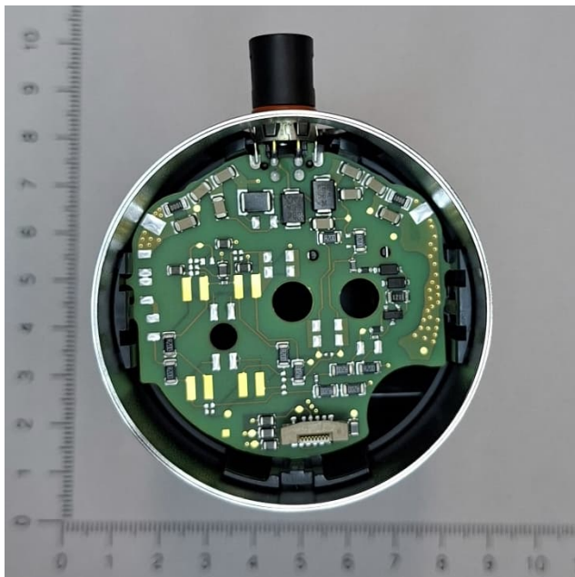
Mainboard, terminal board and sensor board in housing *
