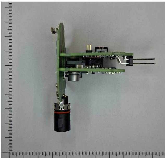
Mainboard, terminal board and sensor board connected - view 1 *
