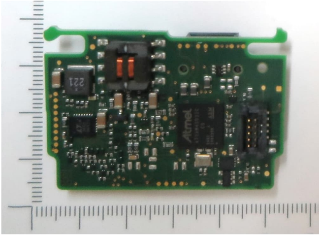
Mainboard - side 1 *
