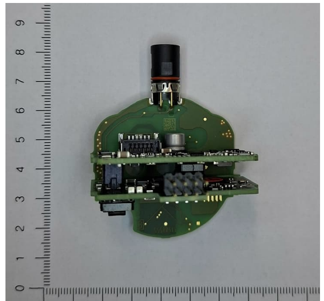
Mainboard, terminal board and sensor board connected - view 2 *
