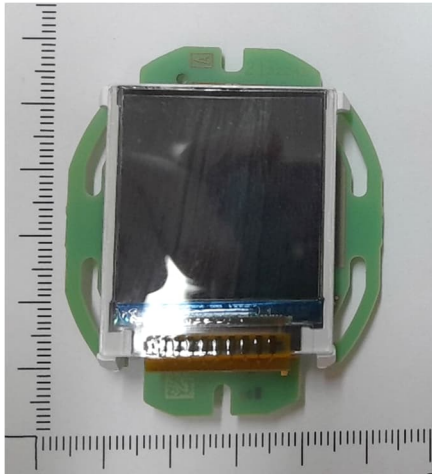
Visualisation board, top view *
