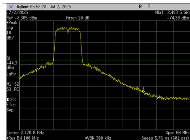
High Ch_2457MHz_10MHz BW_-20dBc_Upper Band Edge_Port 1
