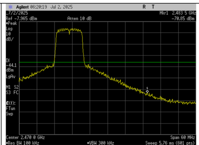
High Ch_2457MHz_10MHz BW_-20dBc_Upper Band Edge_Port 2
